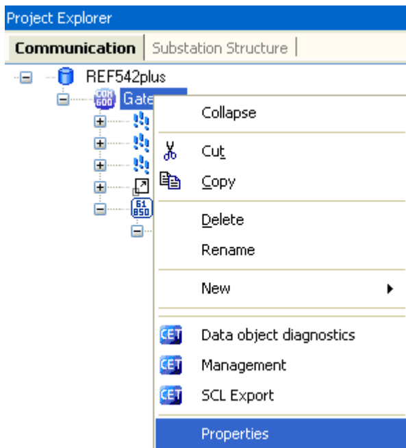
Figure 4-48 SAB600Properties menu
