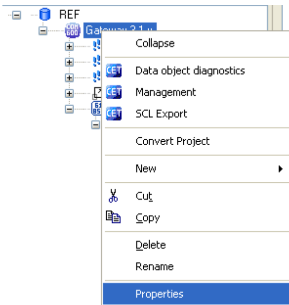
Figure 4-31 SAB600Properties menu
