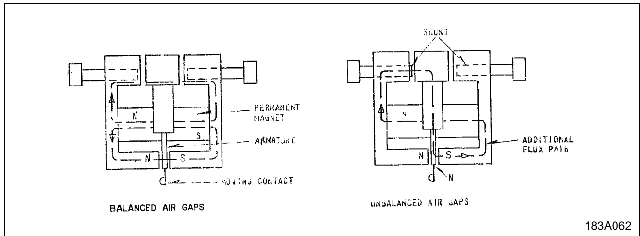
Figure 4 .Polar Unit Perament Magnet Flux Paths
