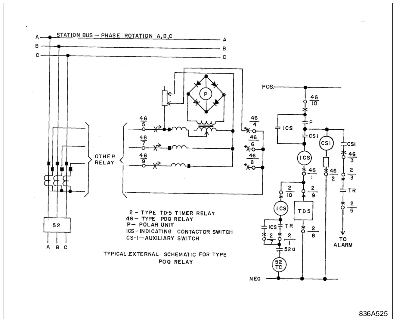
Figure 5. External Schematic for Type POQ Relay
