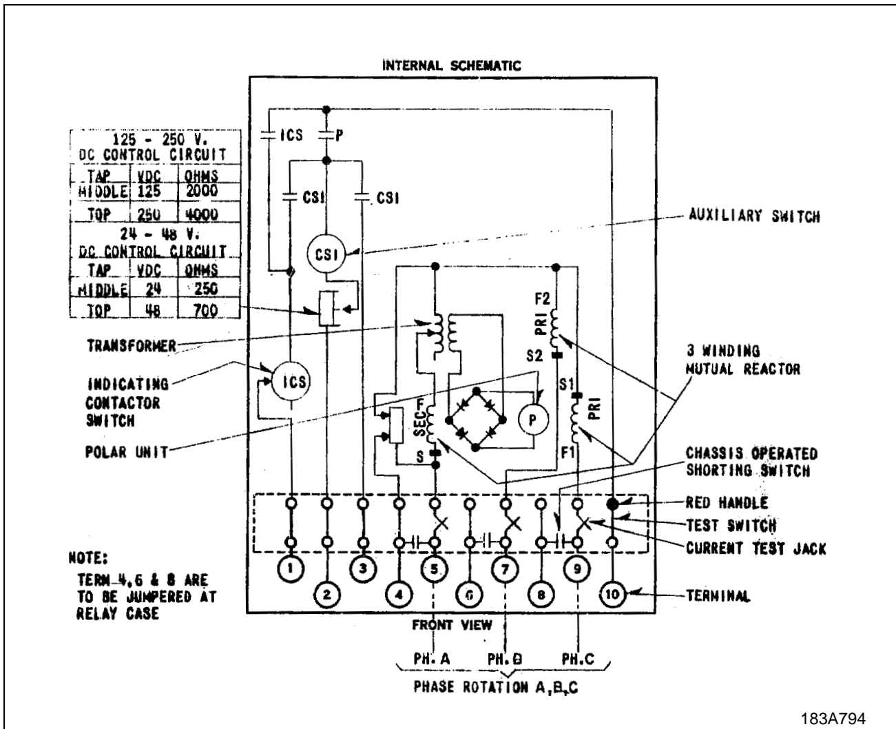
Figure 3. Internal Schematic of the Type POQ Relay in FT-21 Case
