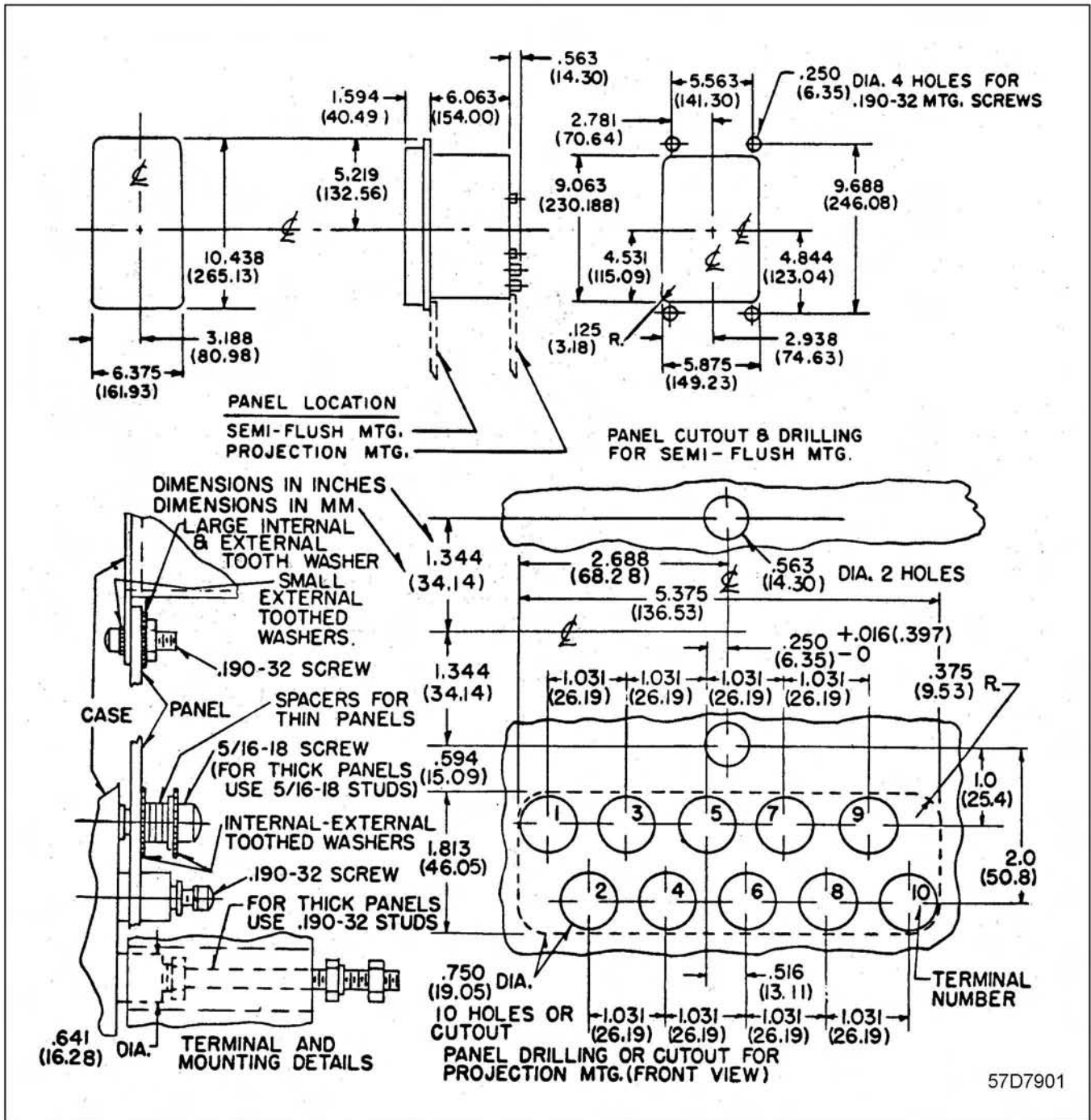
Figure 7 .Outline and Drilling Plan for the Type POQ Relay in the FT-21 Case
