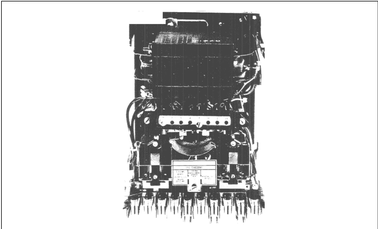
Figure 1 .Type POQ Relay in FT-21 case (Front View)
