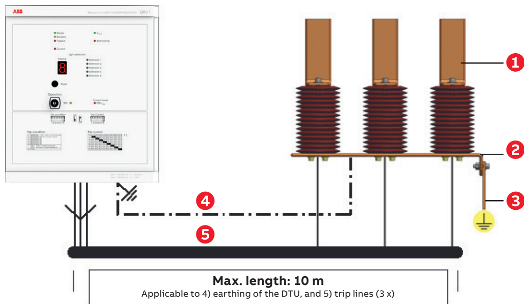
Fig. 5.2-1 System configuration
