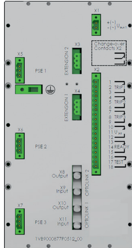
Fig. 3.1.1-2 TU rear view
