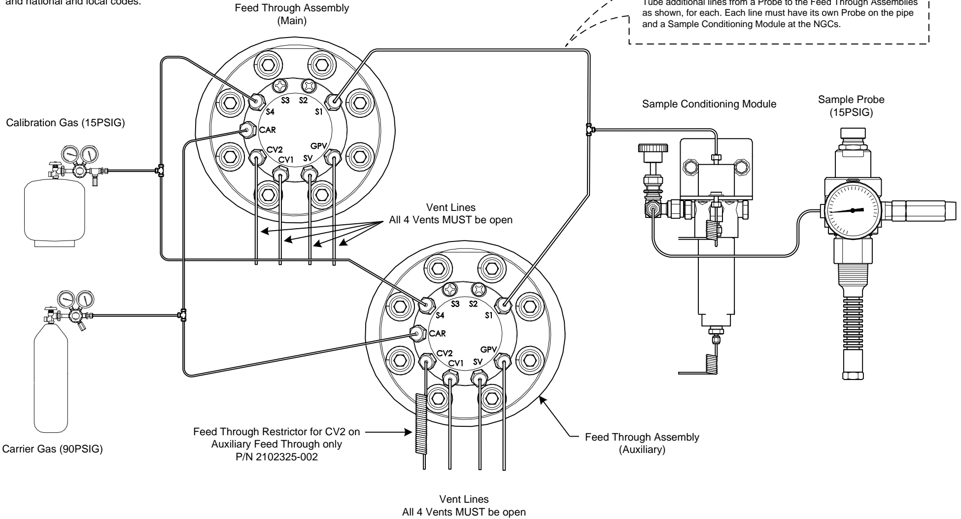
Connecting Lines to Feed Through Assemblies on the NGC8209
