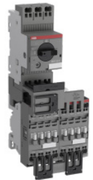
Reversing Starter
