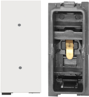
Internal arc shield provided in switch mechanism
