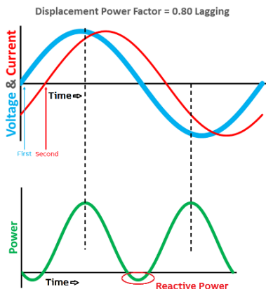
Figure 3 Lagging Power Factor 0.8
