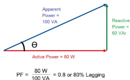
Figure 4 Power Triangle
