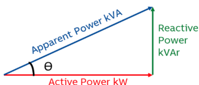
Figure 1 Power triangle
