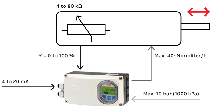
EDP300 control unit for remote sensor
