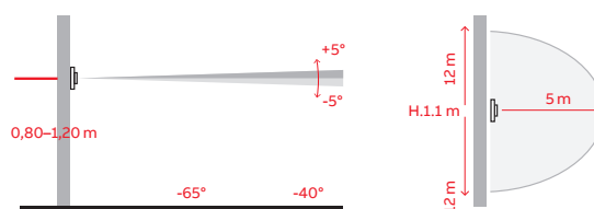
Flex Basic/Comfort 180° tunnistusalue
