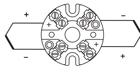
Double sensor
