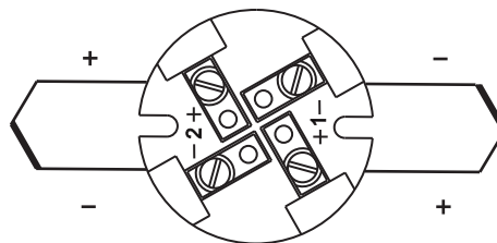
Double sensor
