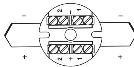
Double sensor
