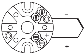
Single sensor
