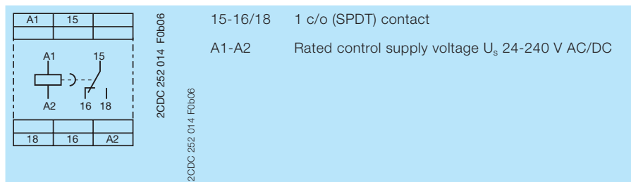
Connection diagram
