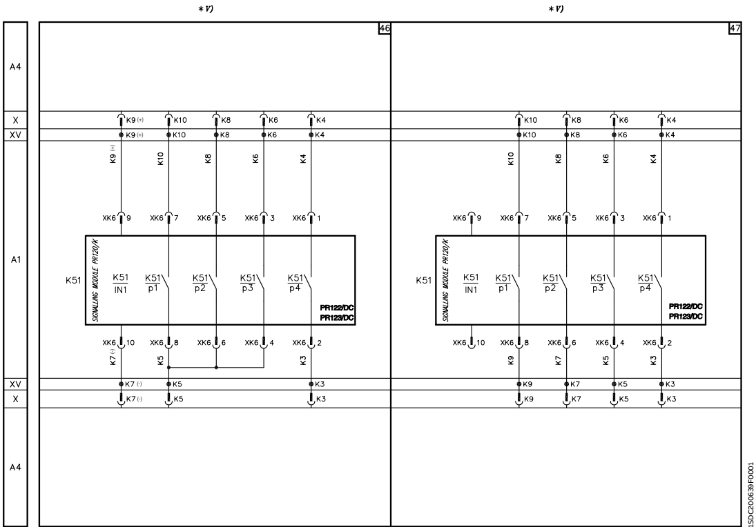
PR120/K信号模块
