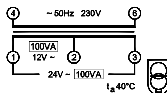
TS100/12-24 C
