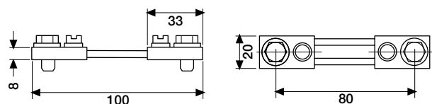
SNT200 ÷ 250 A/60 mV
