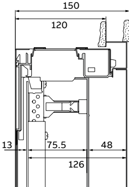
Panel with mounting plate
