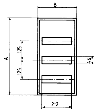
Allowed power loss hood-type consumer units A300
