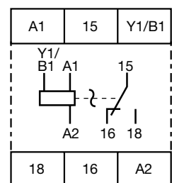
CT-TGD.12
