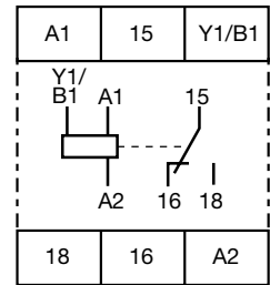
CT-MFD.12
