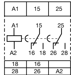
CT-ERD.22
