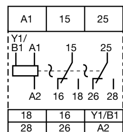
CT-TGD.22
