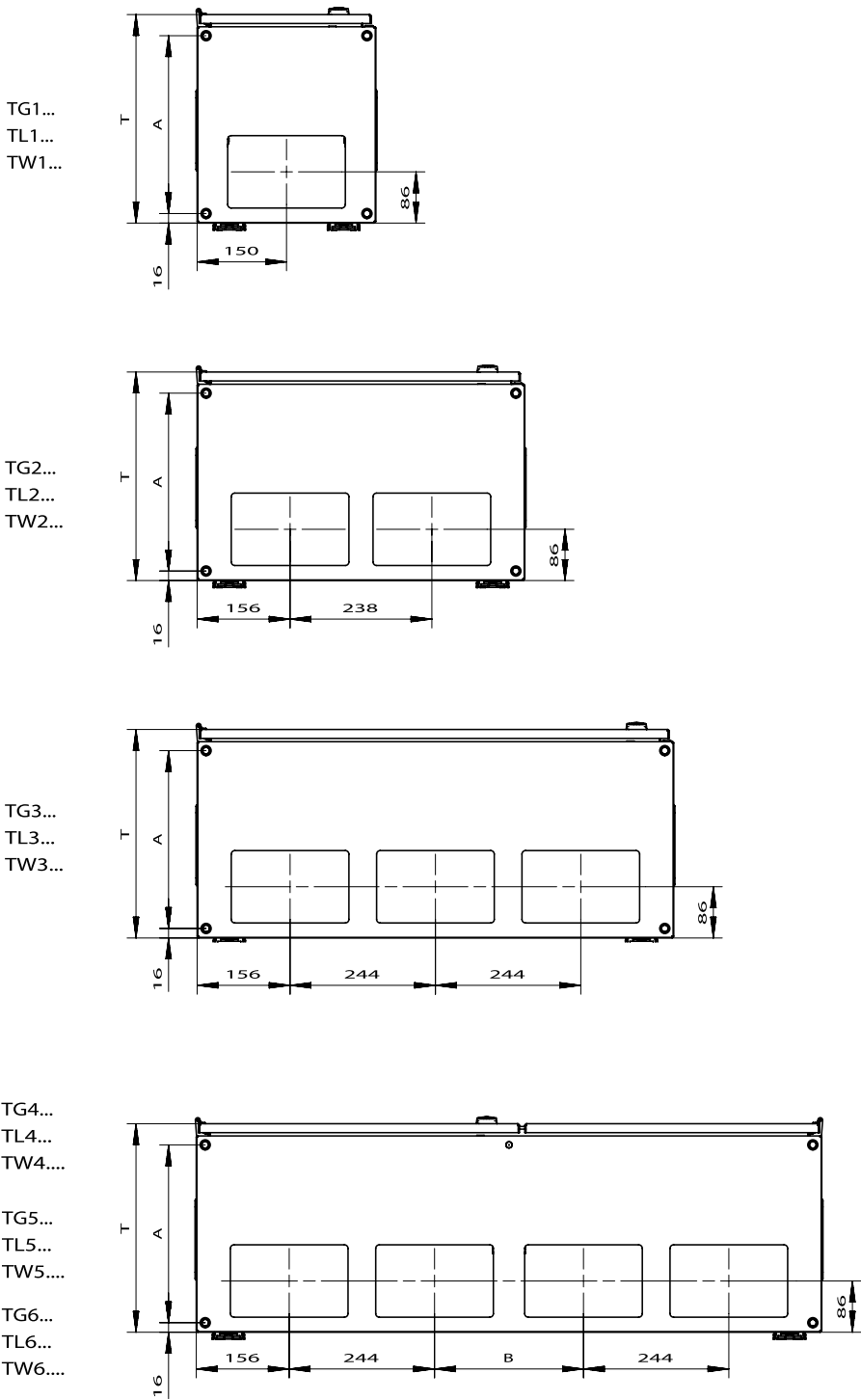
TwinLine Top view / side flange knockout, top and bottom
