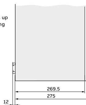
Side view With/without door
