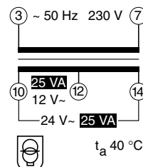
TS100/12-24 C
