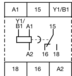
CT-AHD.12
