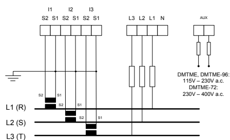
Three-phase with 3 CTs
