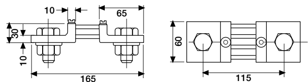
SNT800 ÷ 1000 A/60 mV
