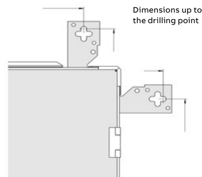
Front view External fastening Detail
