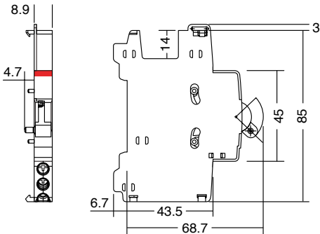
SN201-IH
