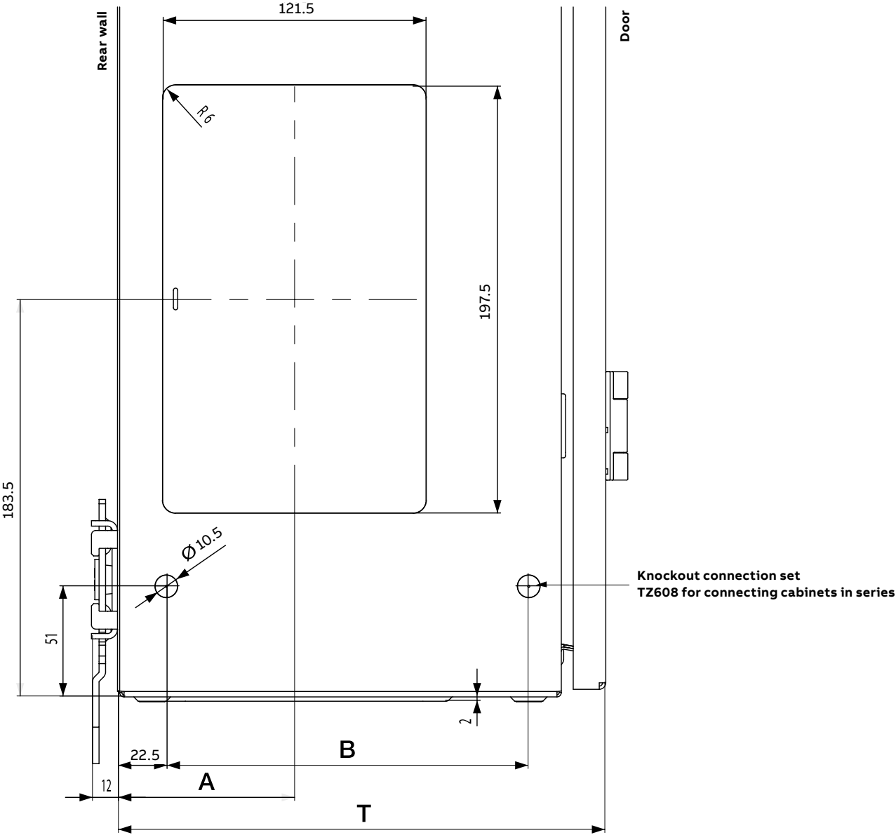
TwinLine Side view / side flange knockout, top and bottom
