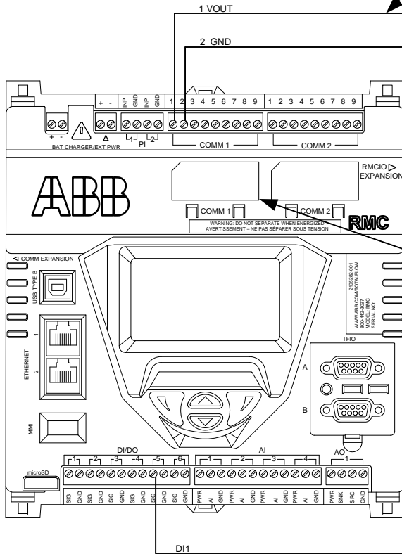
RMC (2105350) Board
