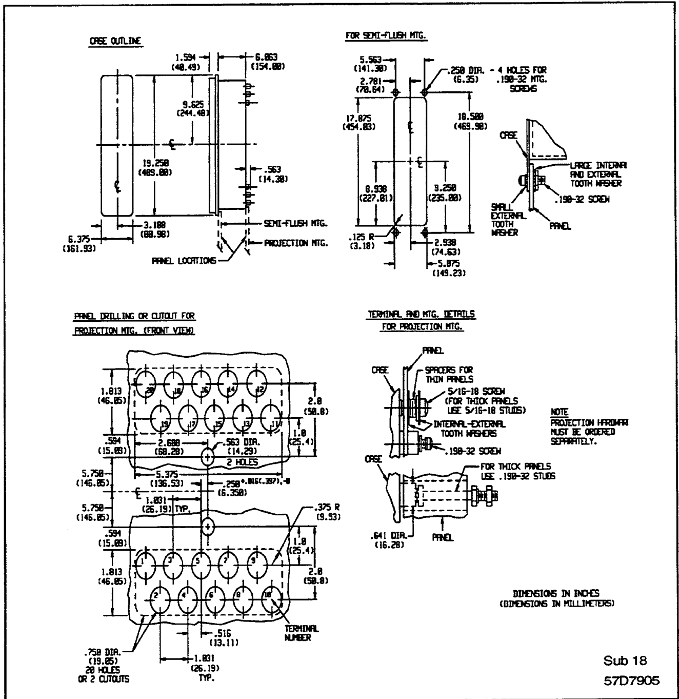
Figure 18. Outline - Drilling Plan for Type KDXG - Relay in FT42 Case
