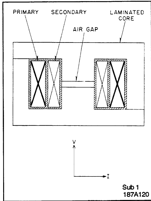
Figure 3. Compensator Construction
