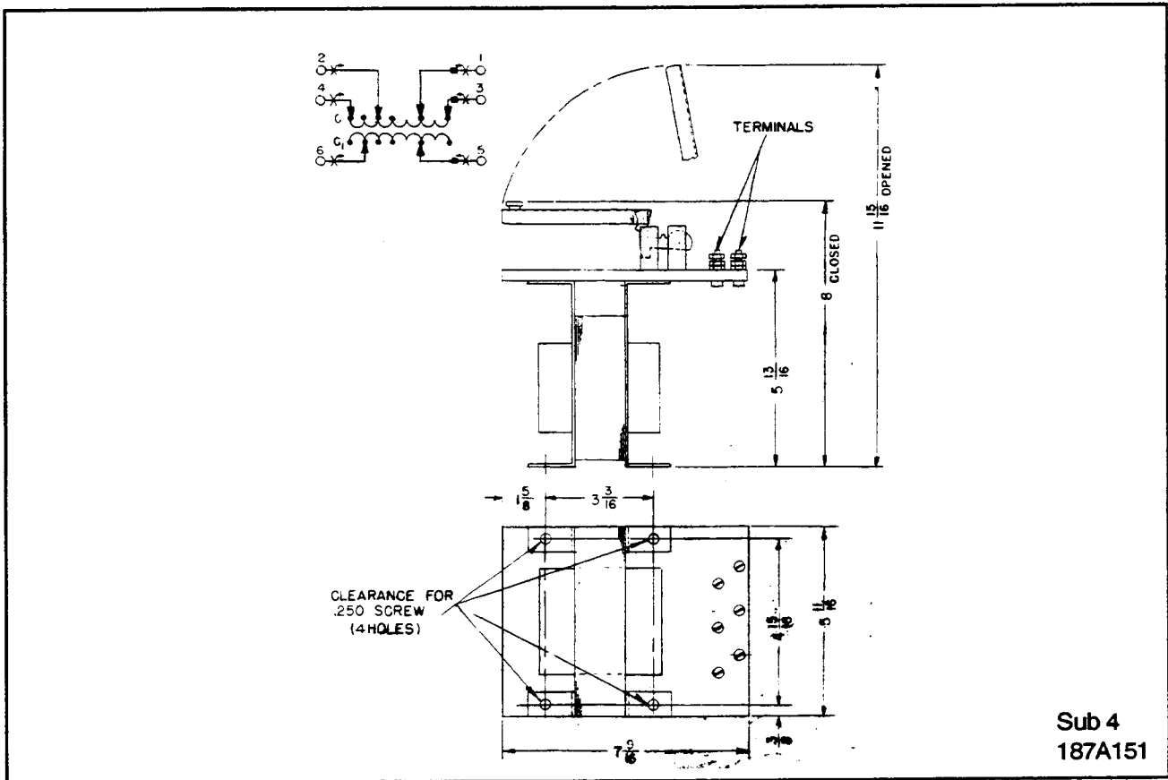
Figure 12. Outline-Drilling Plan for Type IK Auxiliary ct.
