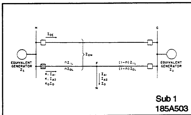
Sub 1 185A503 Figure 7. General System Used for Describing Type KDXG Relay Operations.
