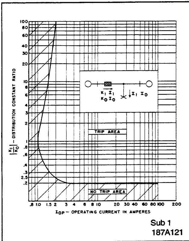
Figure 9. Typical Operating Characteristics of the Ratio Discriminator as a Function of Current Distribution Factor Ratio and Operating Current.
