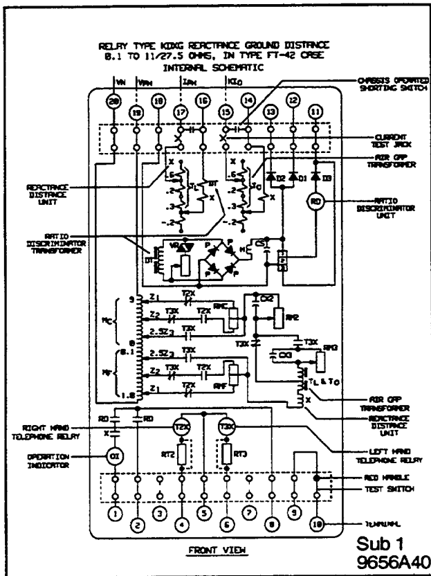
Figure 2. Internal Schematic of the Type KDXG Relay in TF42 Case
