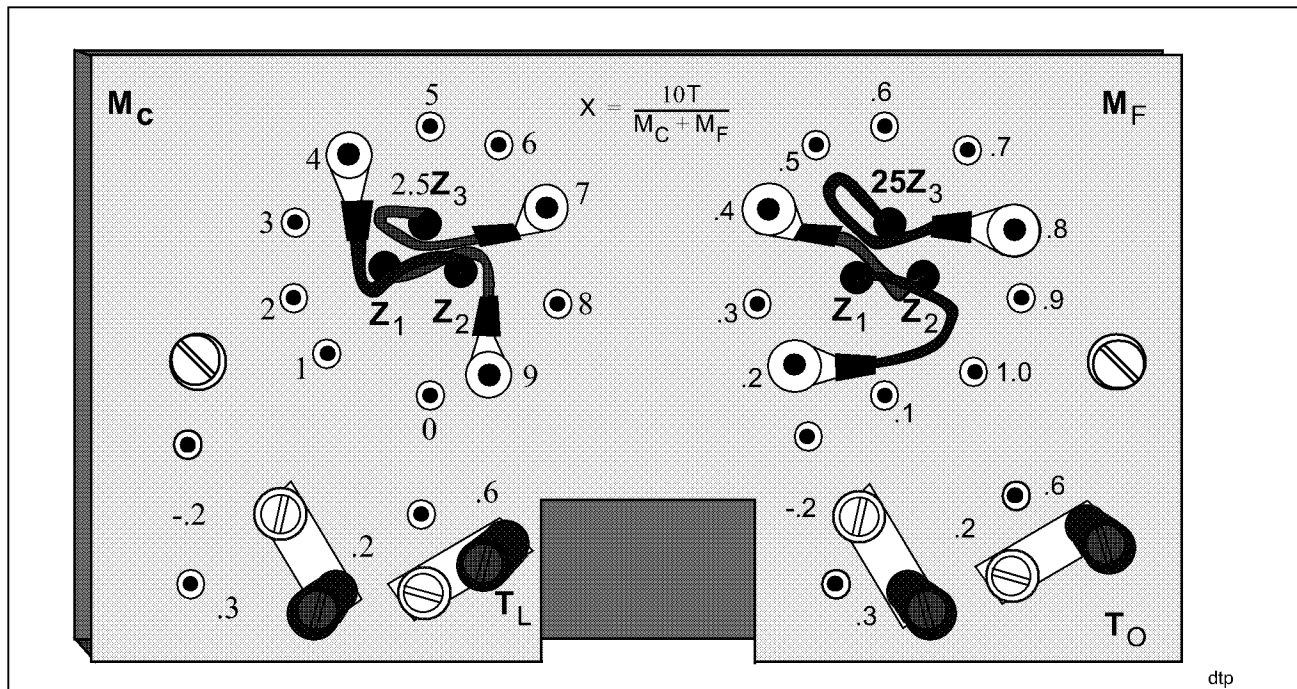
Figure 4. Tap Plate
