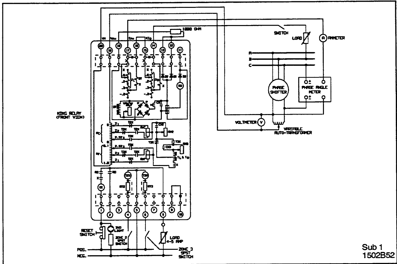
Figure 13. Test Connections for Type KDXG Relay
