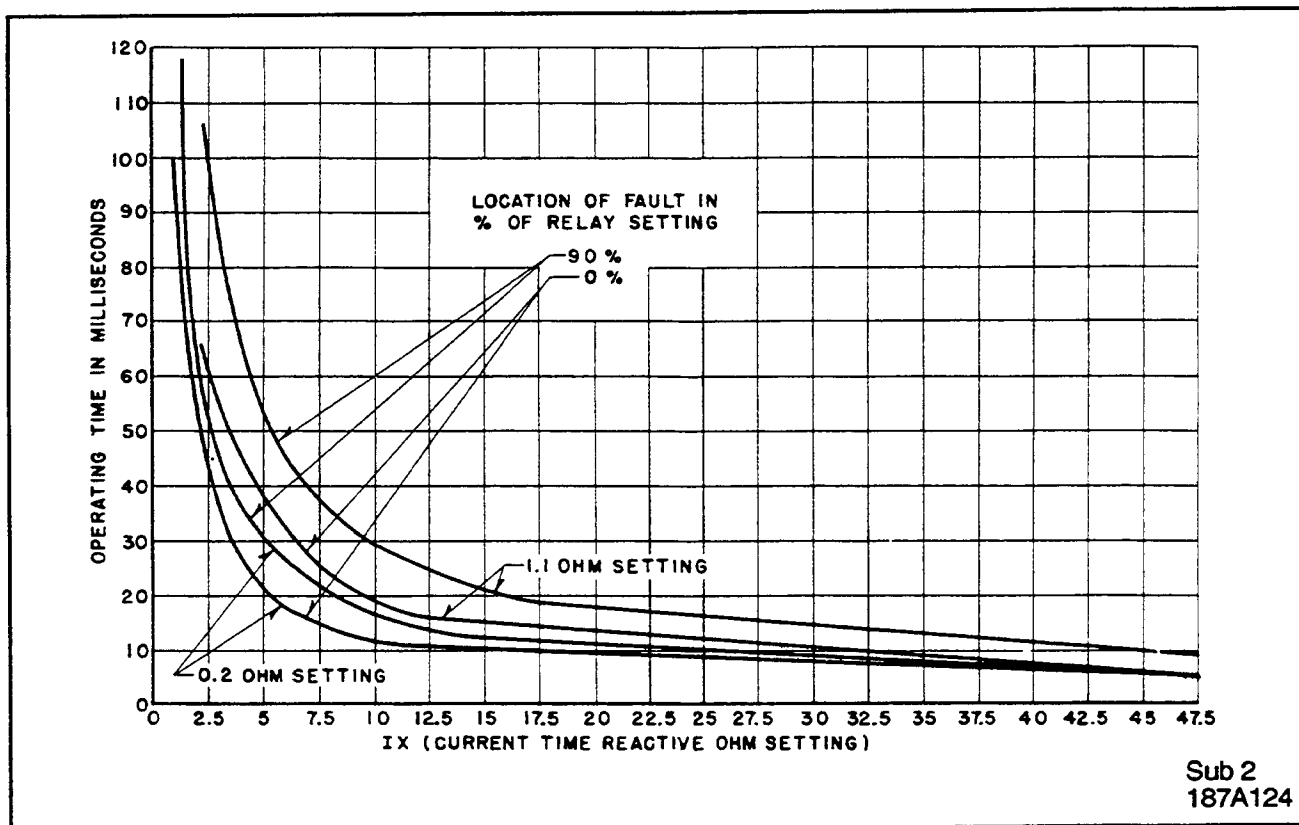
Figure 16. Typical Operating Time Curves of the Reactance Unit
