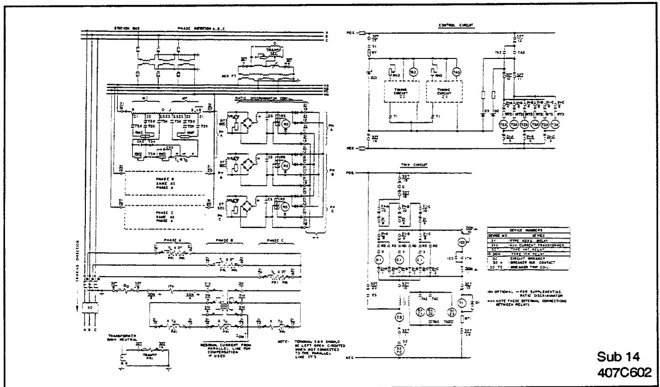
Figure 6. External Schematic for Type KDXG Relay with KRT.
