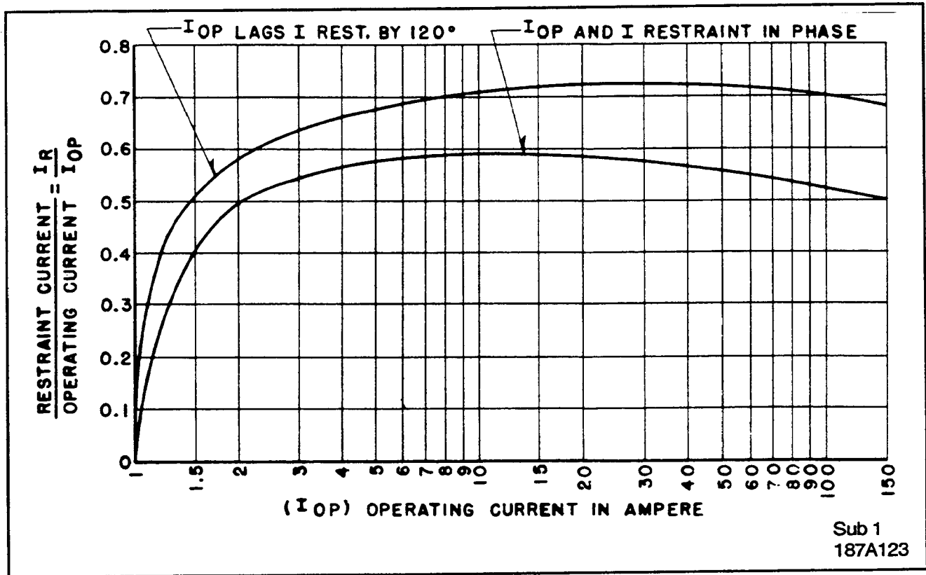
Figure 11. Typical Ratio Discriminator Trip Characteristic ( I_{res}/I_{op} ) as Function of Operating Current I_{op} .
