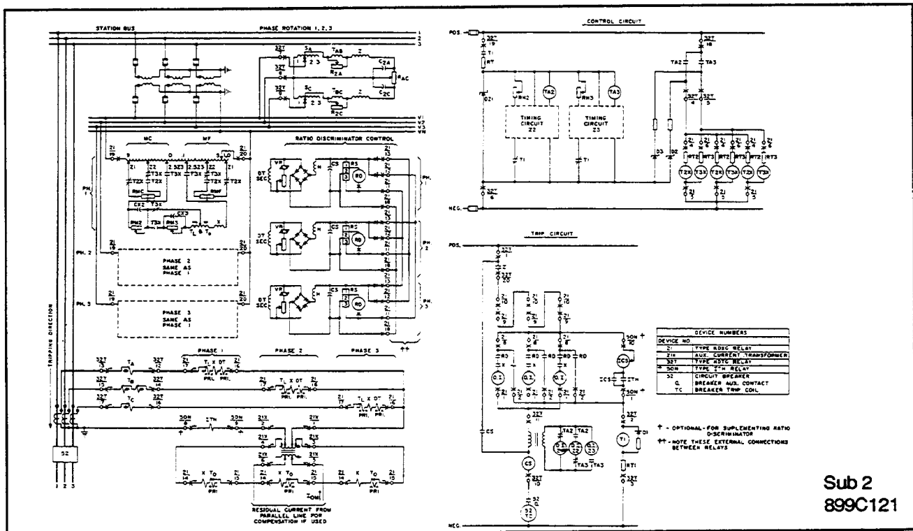
Figure 14. External Schematic for Type KDXG and KDTG Relays
