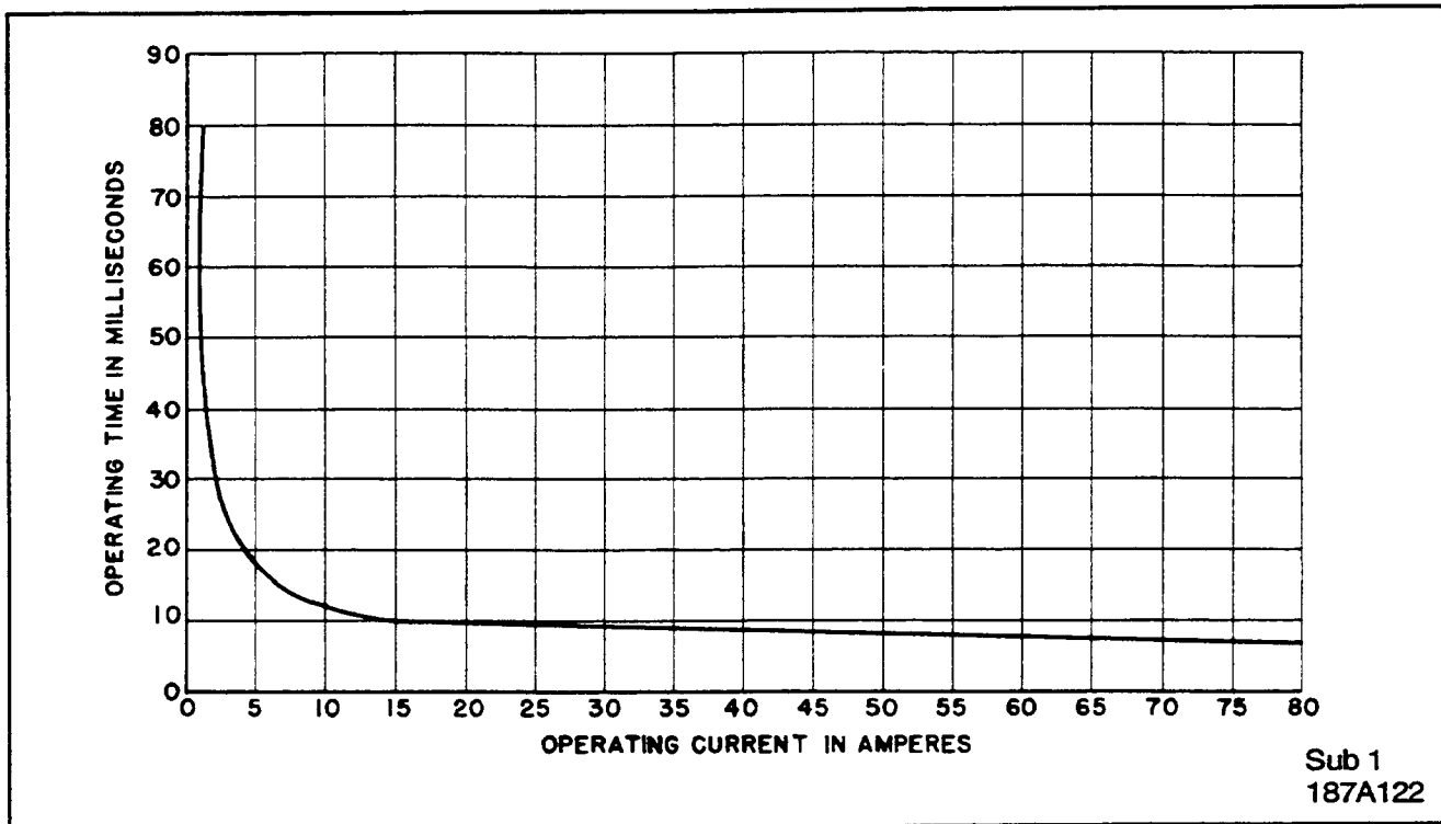
Figure 10. Typical Operating Time Curve of the Ratio Discriminator Unit.
