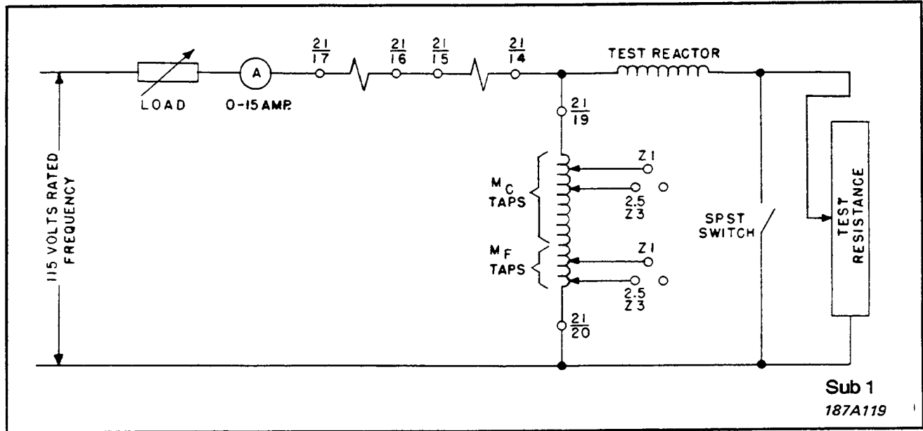
Figure 15. Circuit for Reactance Unit Phase Angle Adjustment
