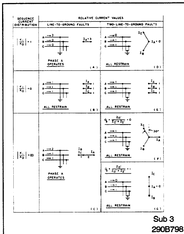
Sub 3 290B798 Figure 8. Response of Ratio Discriminator to Ground Faults, Assuming All Impedances in Phase
