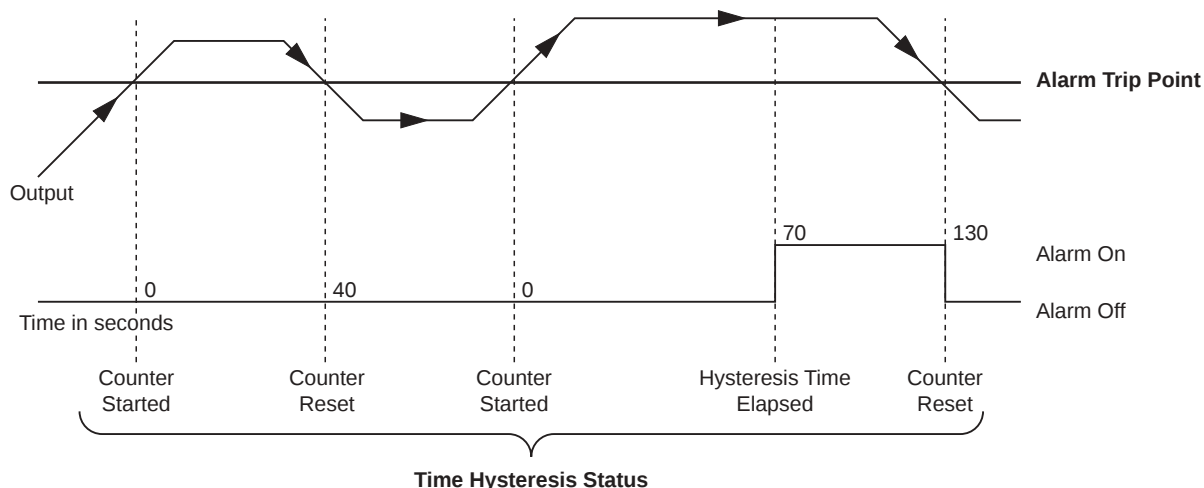
Fig. 3.4 Time Hysteresis Alarm
