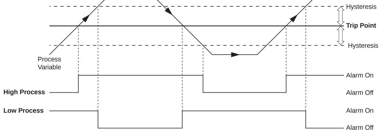
Fig. 3.3 High and Low Process Alarm with Hysteresis
