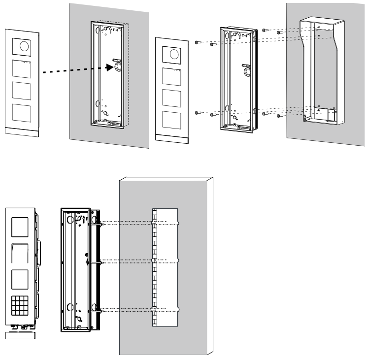
Fig.36 Flush-mounting box installation
