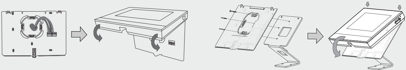
Surface mounted and desktop of 7" video hands-free indoor station
