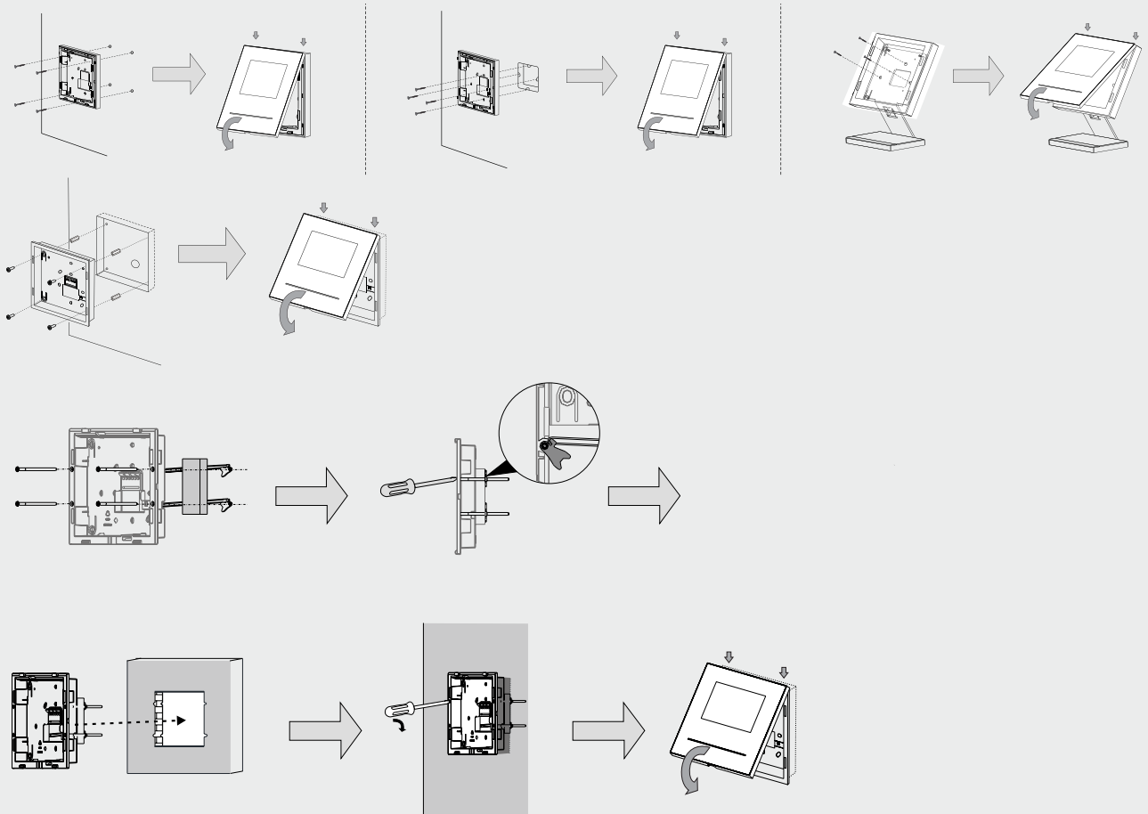
Surface mounted, desktop mounted and flush mounted of 4.3" video hands-free indoor station
