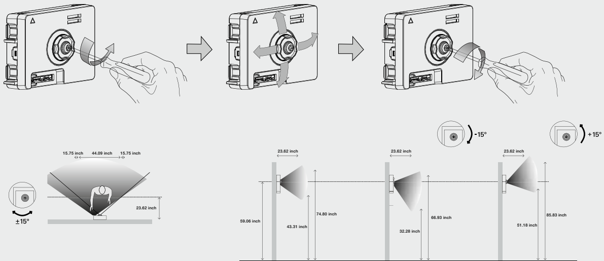
Mechanical adjustment and detection angle of camera
