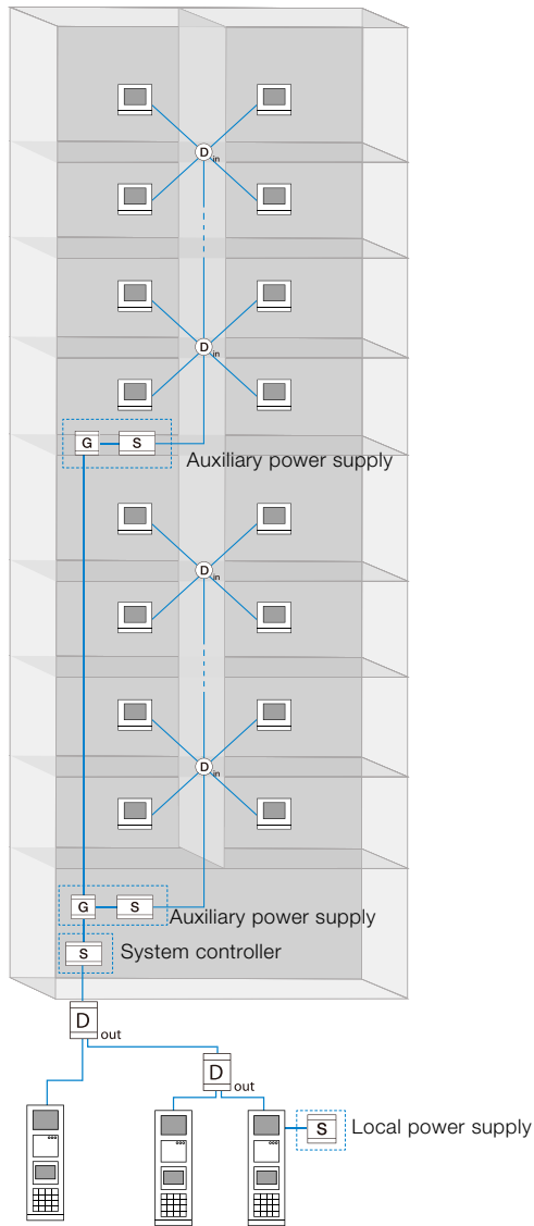
Application of system controller, local power supply and auxiliary power supply
