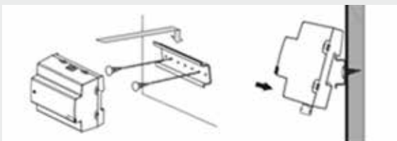
Mounting of the MDRC devices
