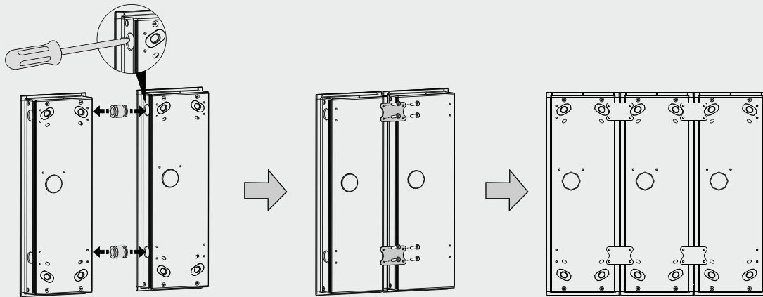
The conjunction of 3 pcs of 4-mould outdoor stations
