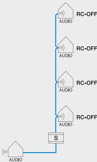
Looping through the indoor station in audio system
