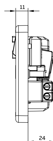
Side view dimensions for 1 gang frames plastic
