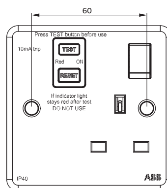
Distance between fixing screws for 1 gang frames
