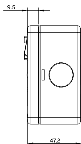
Side view dimensions for 1 gang frames metal
