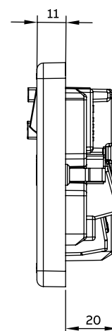
Side view dimensions for 2 gang frames plastic
