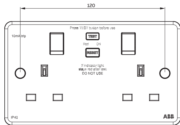
Distance between fixing screws for 2 gang frames
