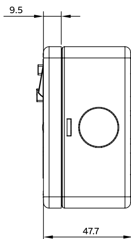
Side view dimensions for 2 gang frames metal
