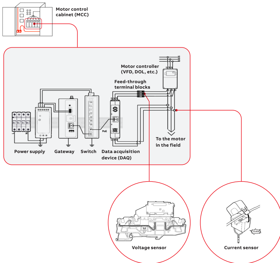
Figure 1. ESA sensors attach to the electrical wires in the motor control cabinet, protected from the hazards of the production floor. Alternatively, it can be embedded directly in the variable frequency drive.
