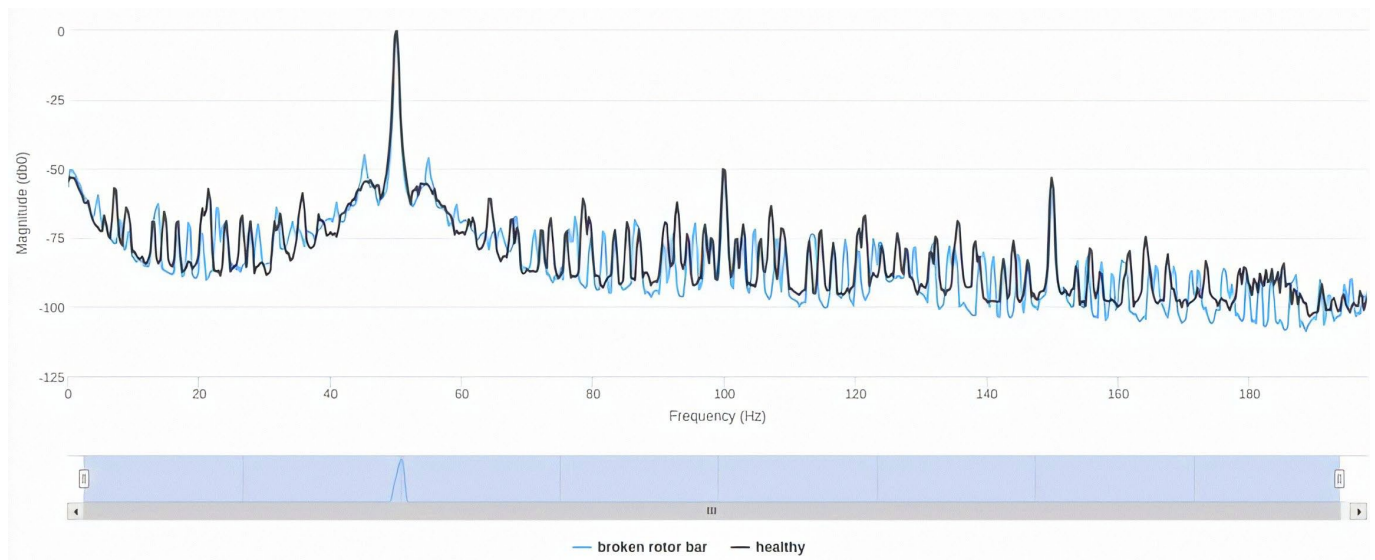
Figure 5. Comparing the spectral energy for a healthy motor (black) and that same motor with a broken rotor bar (blue).
