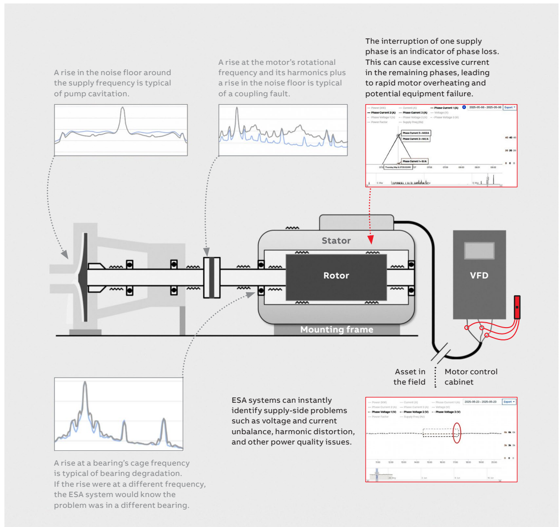
Figure 9. ESA will detect electro-magnetic anomalies earlier than most techniques.
