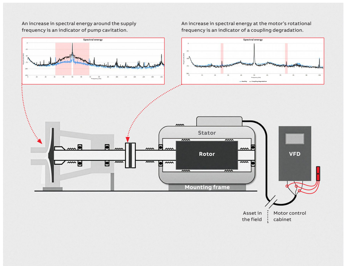
Figure 8. ESA can detect and localize mechanical faults in diverse parts of the connected asset.
