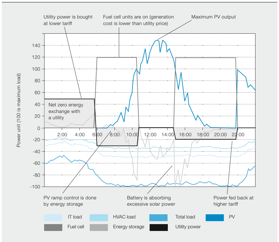
3 A ZNE data center must consume no net energy from the utility grid over a specified time period.
