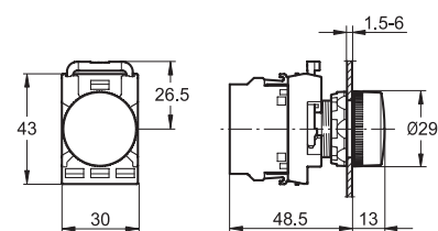
Pilot light
