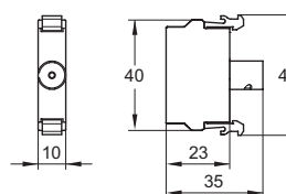
Emergency stop shroud Compact range
