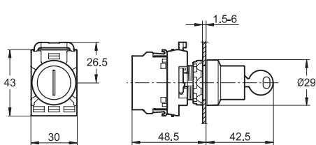
Key-operated selector switch
