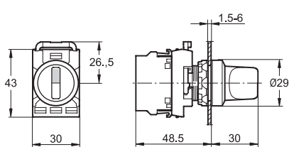
Selector switch
