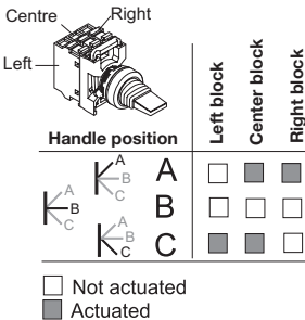
Contacts actuated
