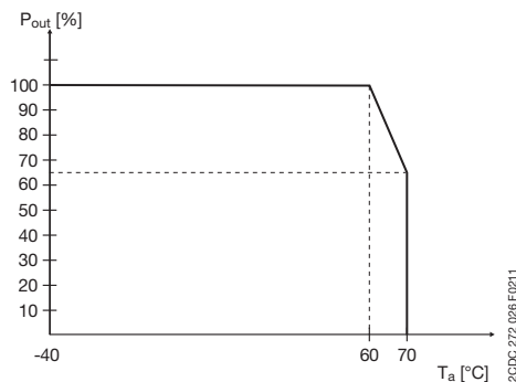
Fig. 5 Derating
