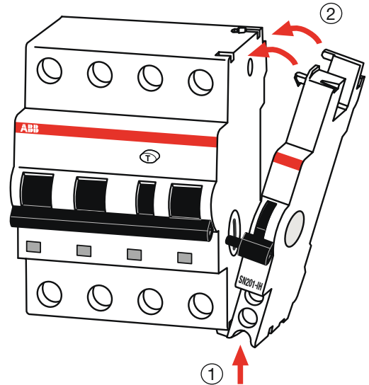
DS203NC + SN201-IH
