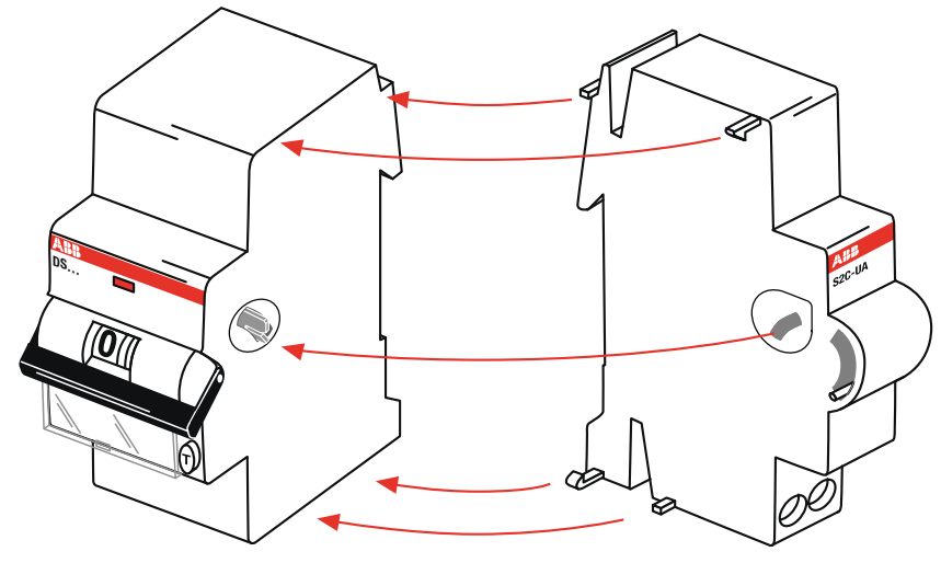
DS202C + S2C-UA
