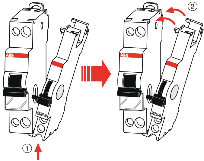
SN201 + SN201-IH
