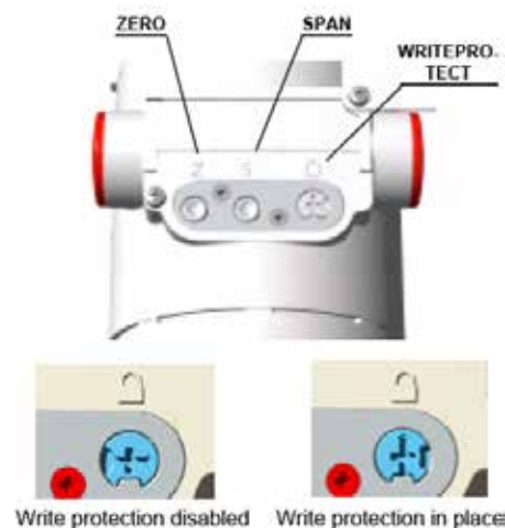
Figure 3: Write-protection pushbutton
