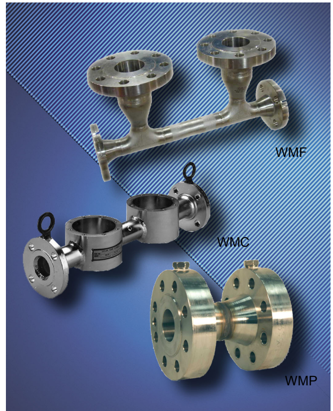
Series WM: C/F/P Wedgemeter
