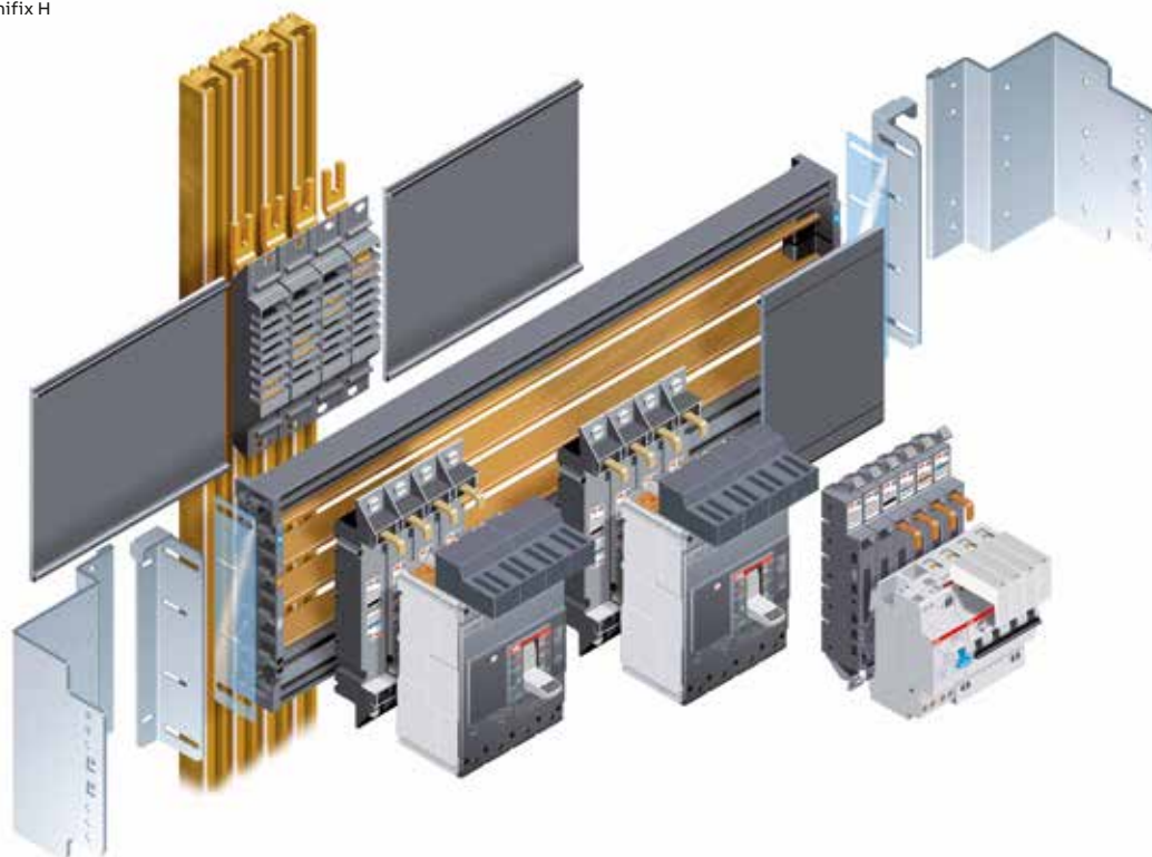
— Unifix H
