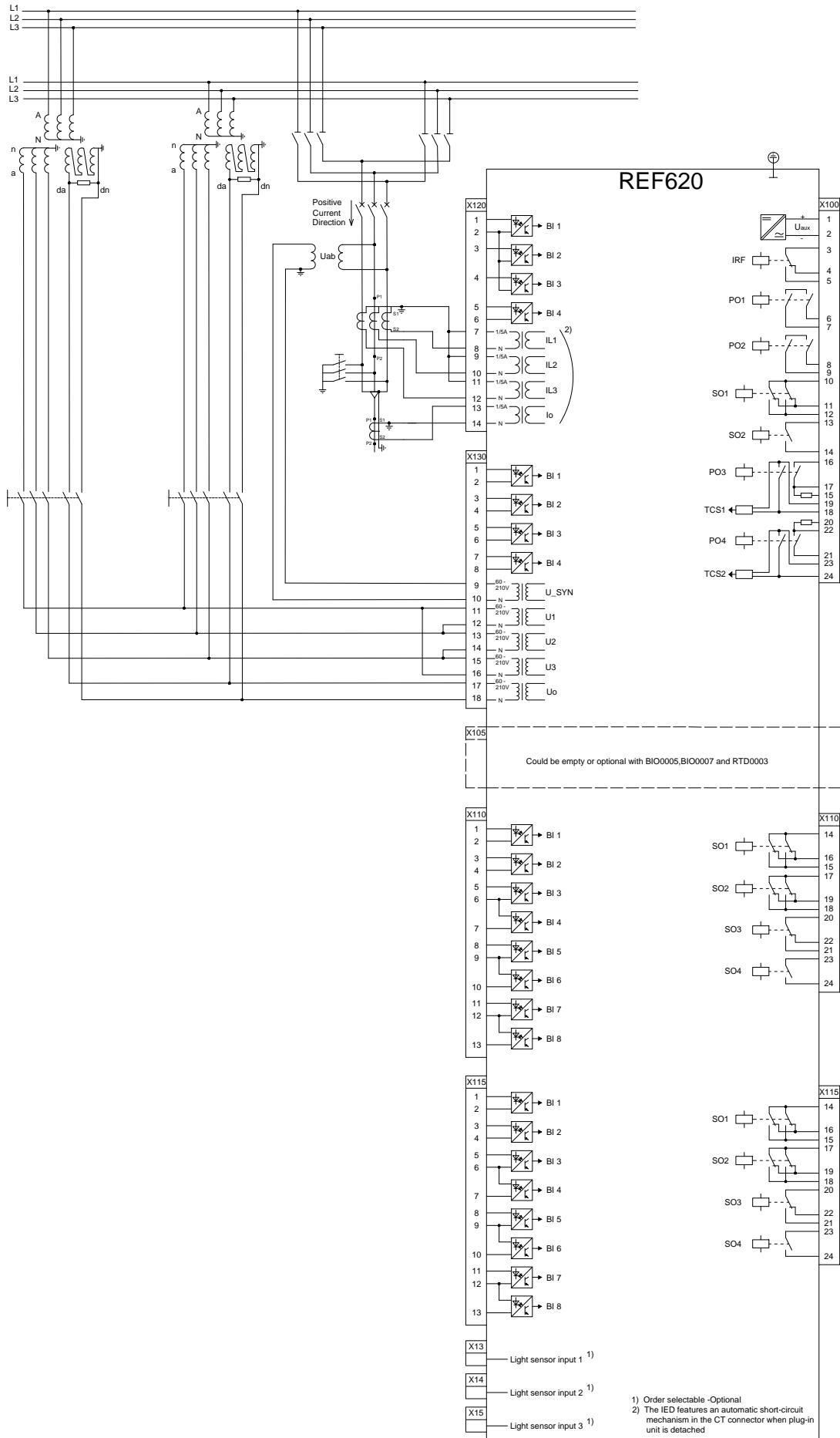
Figure: REF620 FE201 Connection diagram for standard modules
