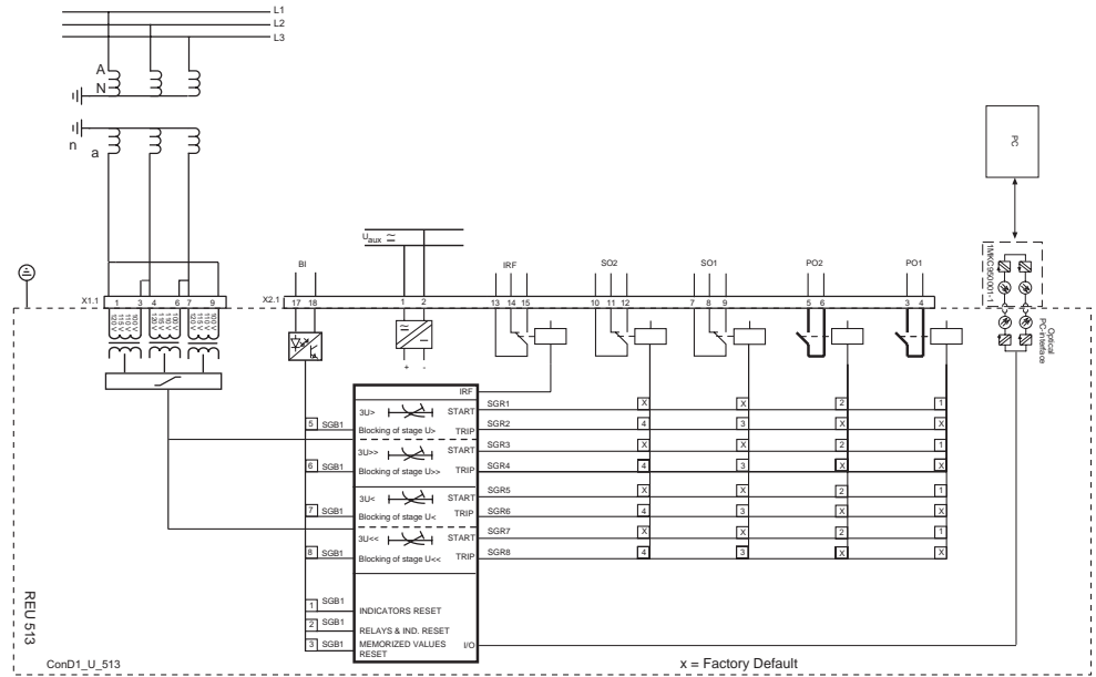
Fig. 1 Block diagram of the combined overvoltage and undervoltage relay
