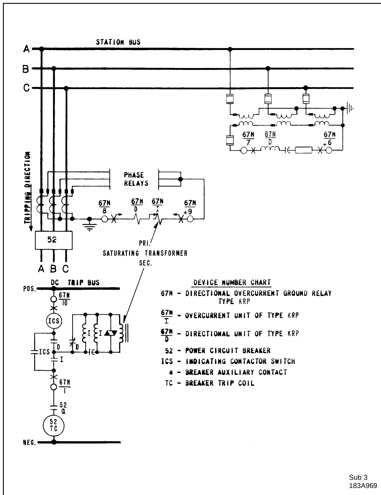
Figure 8: External Schematic of the Type KRP Relay
