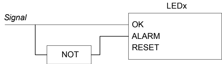
Figure 2: Signal wired to both OK and ALARM inputs – inverted to the other
