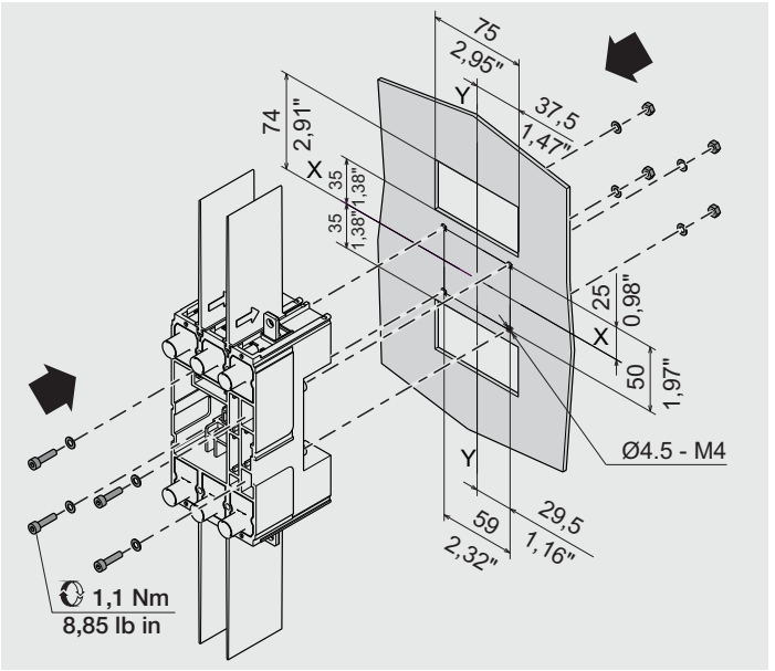
F XT1-UL/III-IV P Fixing at 50mm/1,97"
