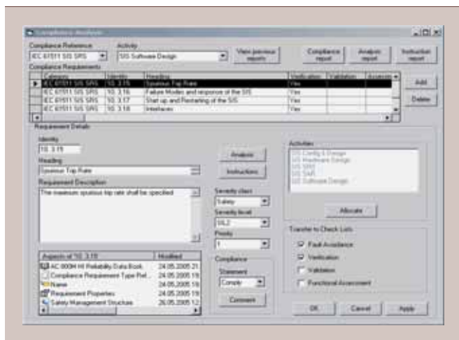
1 Compliance Manger screenshot.
