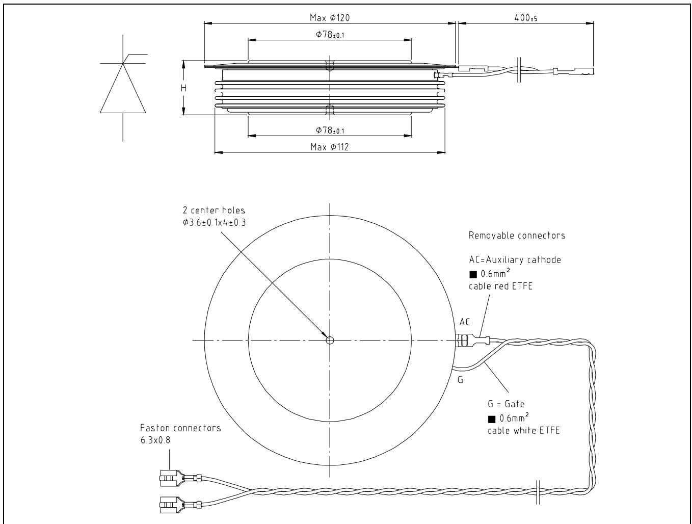
Fig. 10 Device Outline Drawing
