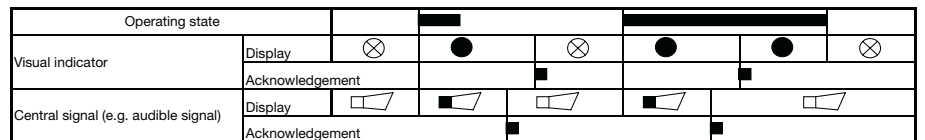
Fig. 5: Function diagram Fault signal with permanent light
