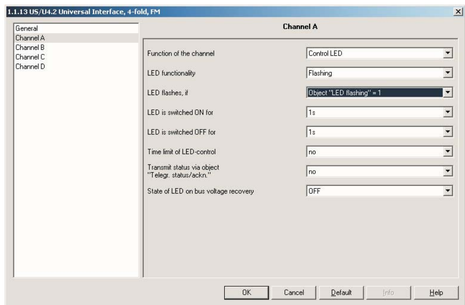
Fig. 27: Parameter window "Channel A of the US/U 4.2"
