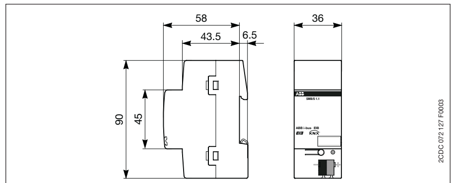
Fig. 3: Dimension drawing of SMB/S 1.1
