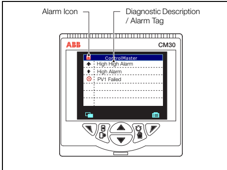
Fig. 5.2 ControlMaster Diagnostic View (ControlMaster CM30 Shown)
