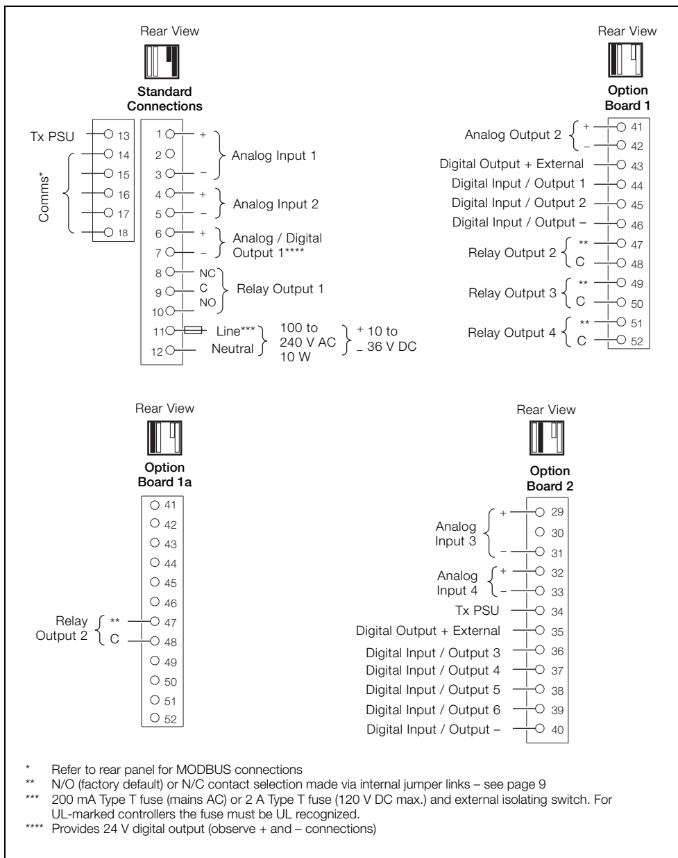
Fig. 4.8 CM30 Electrical Connections
