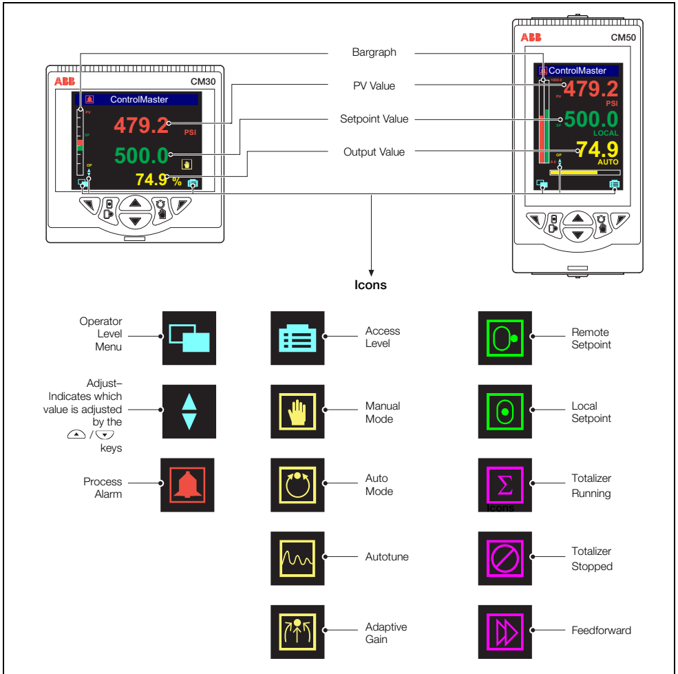
Fig. 3.1 ControlMaster CM30 and CM50 Displays and Icons
