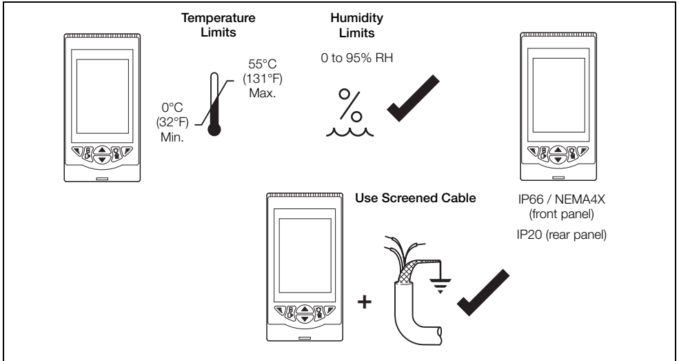
Fig. 4.2 Environmental Requirements
