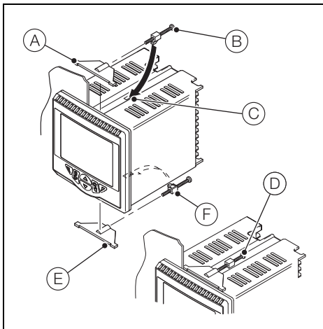
Fig. 4.5 Mounting Details
