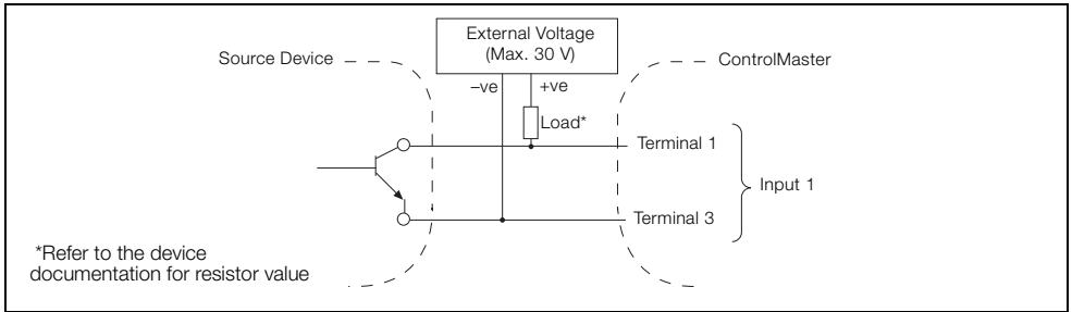
Fig. 4.12 Frequency / Pulse Input
