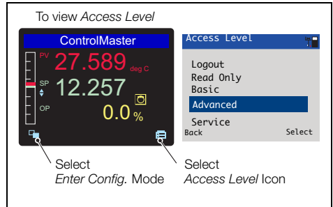
Fig. 5.3 Access Level
