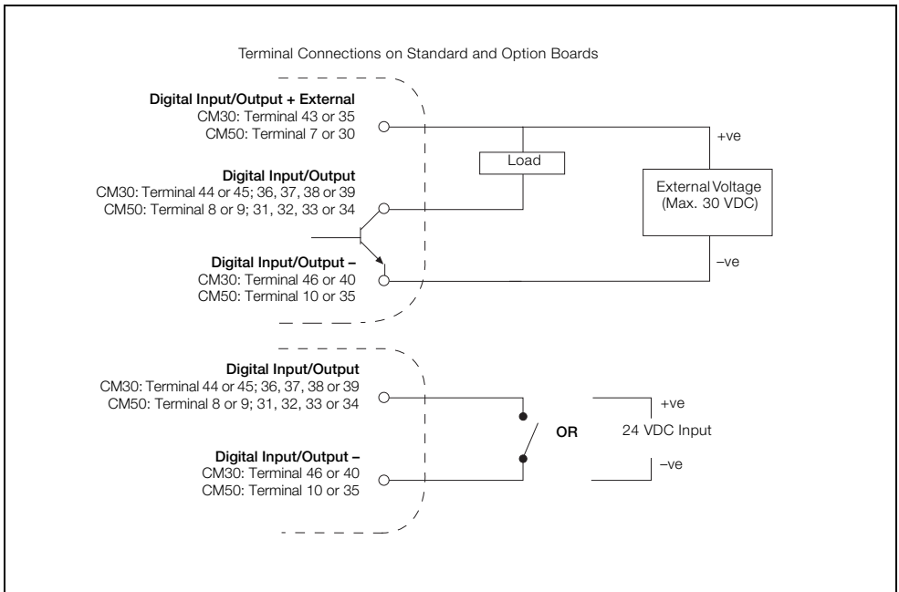
Fig. 4.13 Digital Input and Open Collector Digital Output Connections
