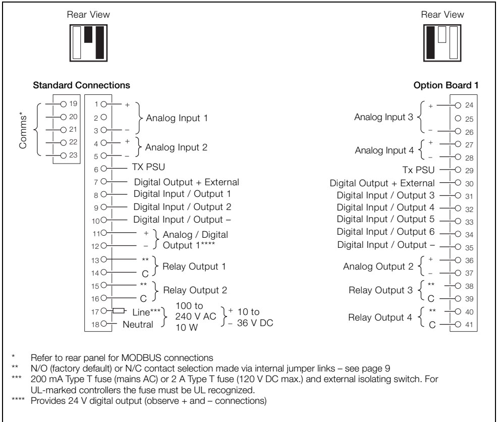
Fig. 4.9 CM50 Electrical Connections
