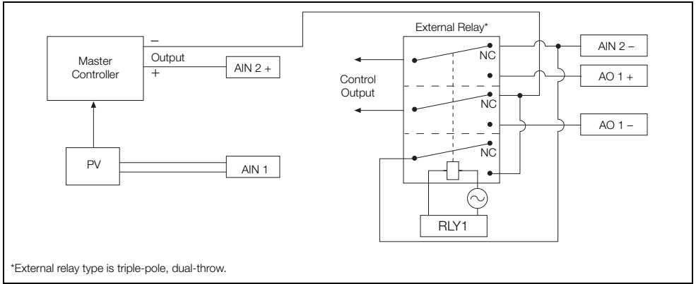
Fig. 8.1 Parallel Connection
