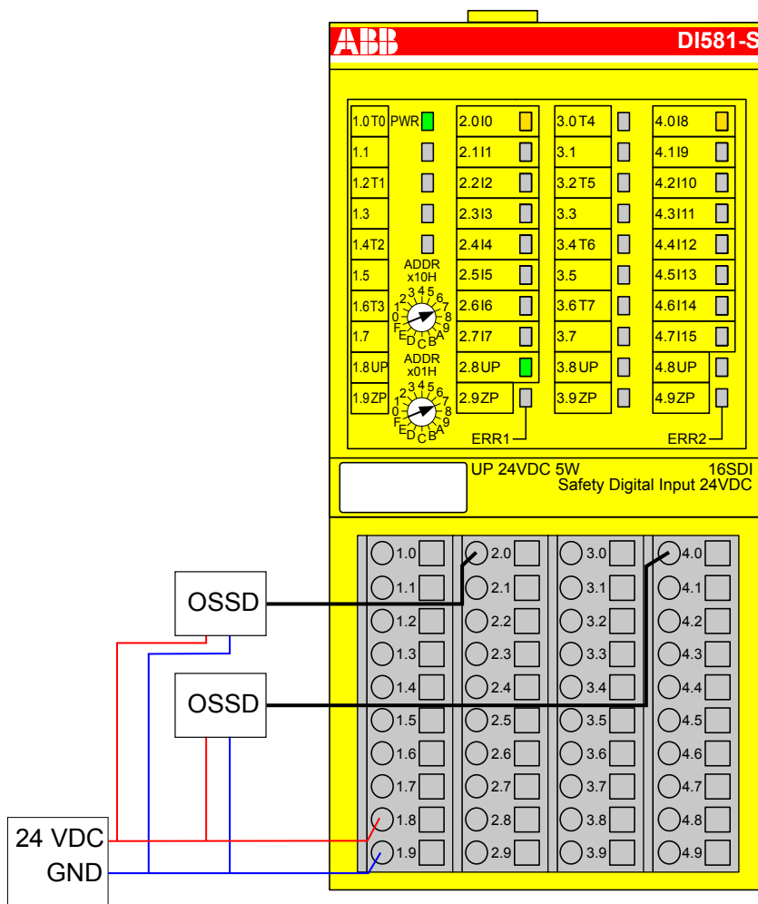
Fig. 33: Circuit example DI581-S, 2 x OSSD output (with internal tests), external sensor power supply
