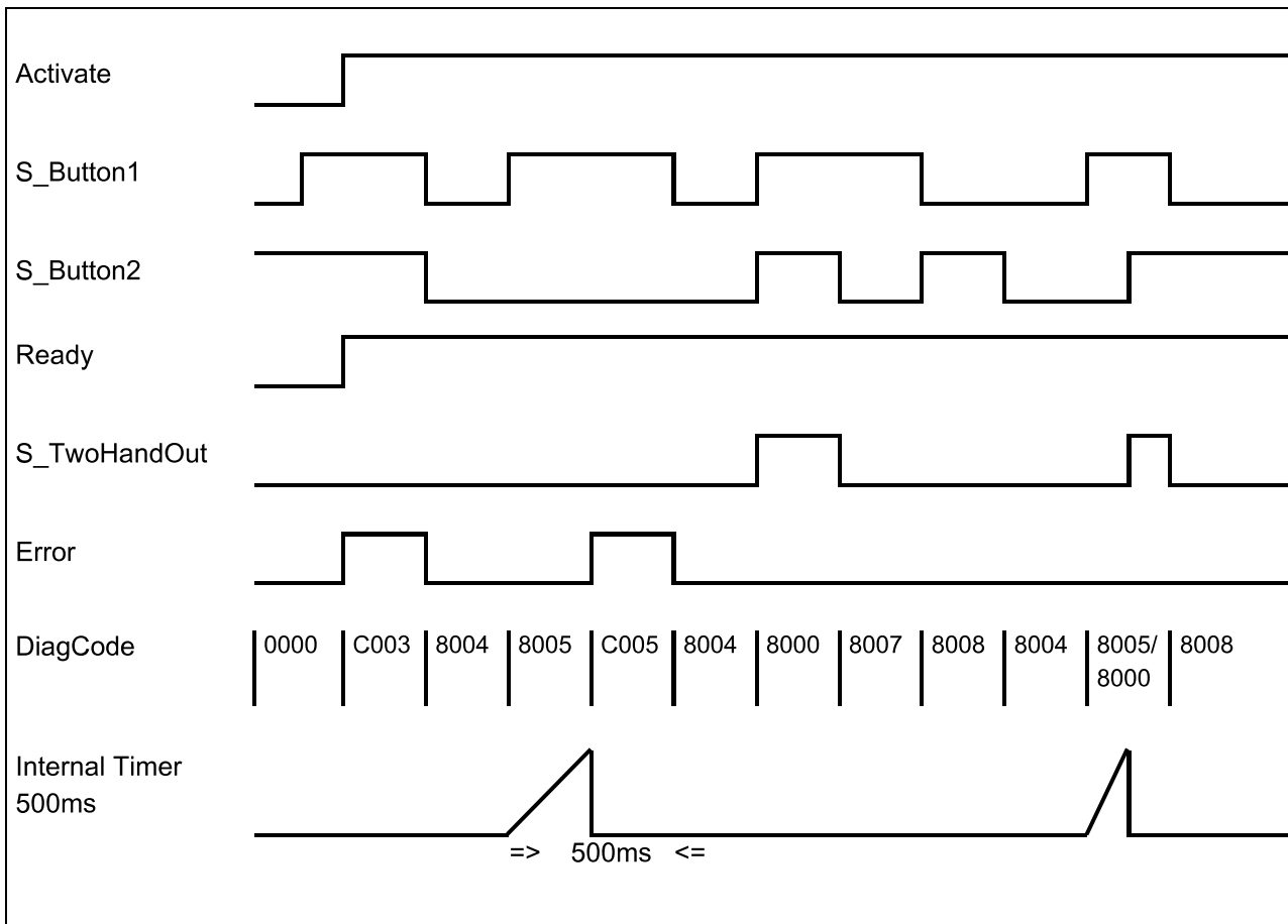
Fig. 97: Timing diagram for SF_TwoHandControlTypeIII
