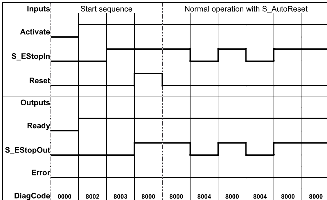
Fig. 91: Timing diagram for SF_EmergencyStop: S_StartReset = FALSE, S_AutoReset = TRUE, Start, normal operation, safety demand, restart
