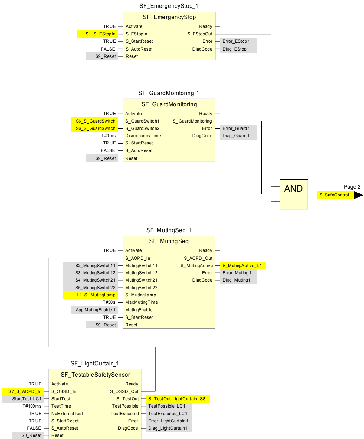
Fig. 125: Access protection at a material gate - Application Program Page 1
