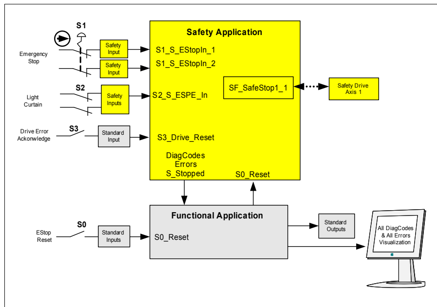
Fig. 122: Graphical overview of the example with emergency stop
