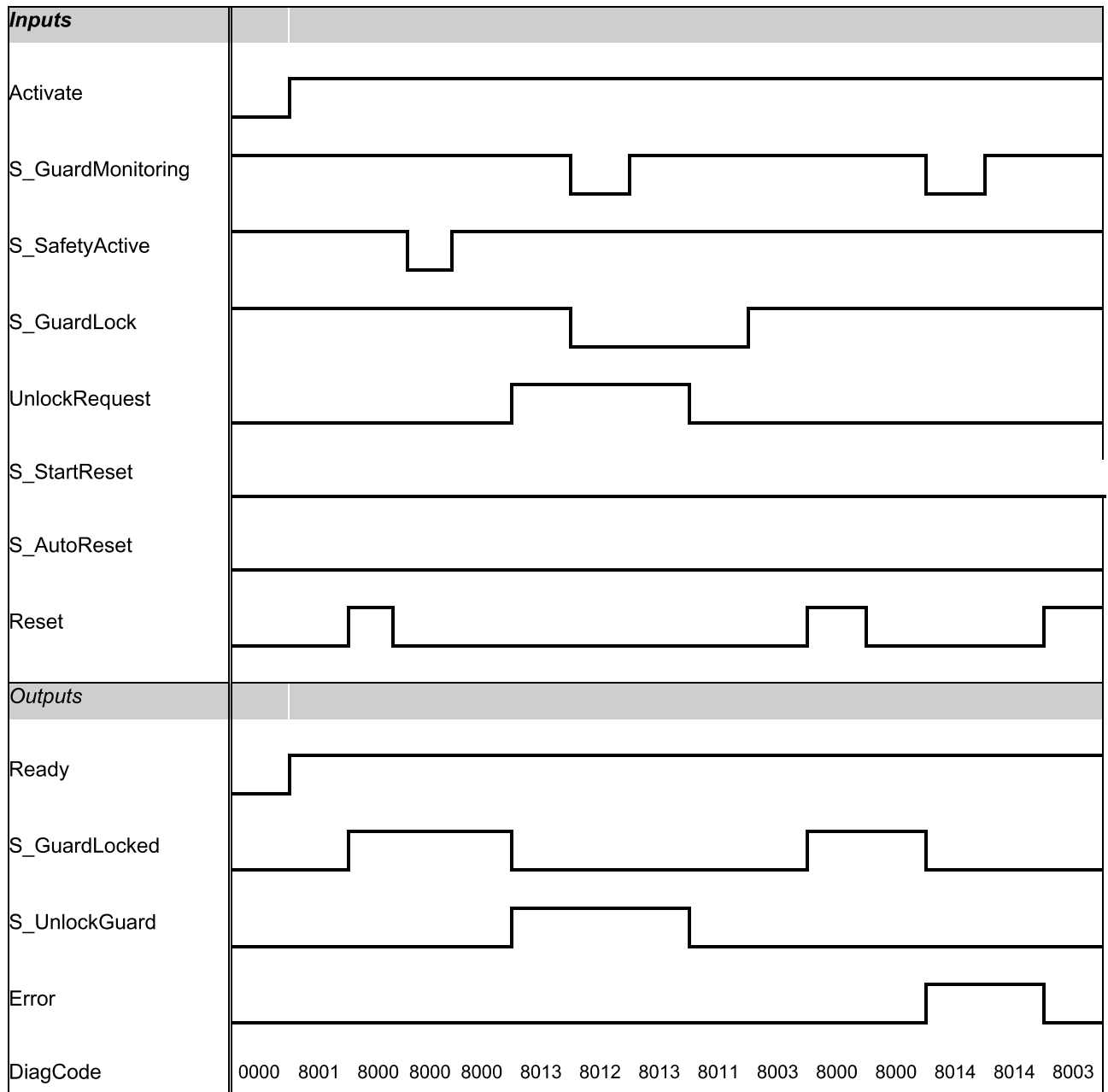
Fig. 98: Timing diagram for SF_GuardLocking
