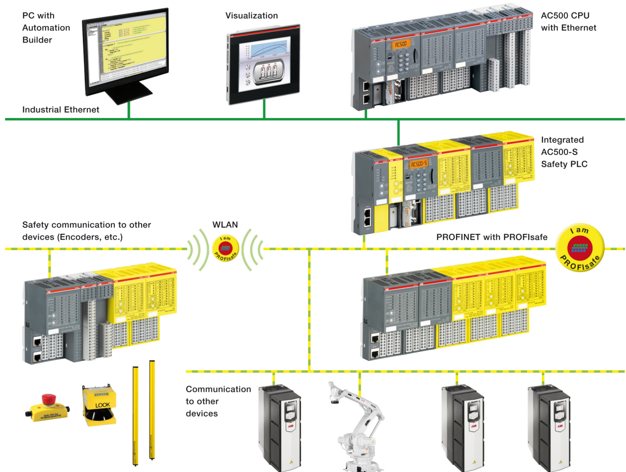
Fig. 3: AC500-S system setup with PROFINET / PROFIsafe
