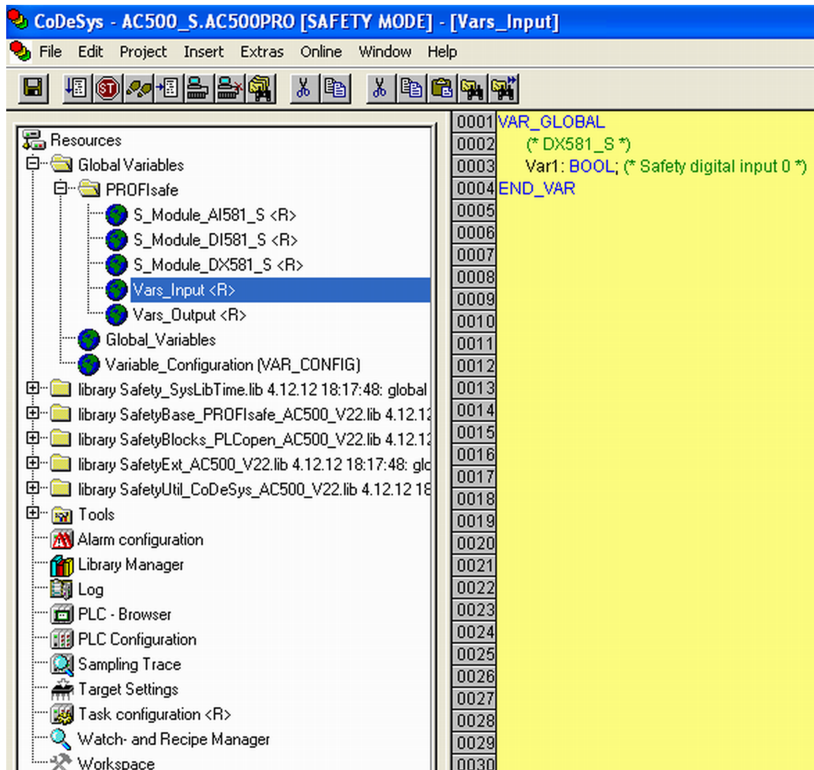
Fig. 75: Global variable list in CODESYS Safety V2.3
