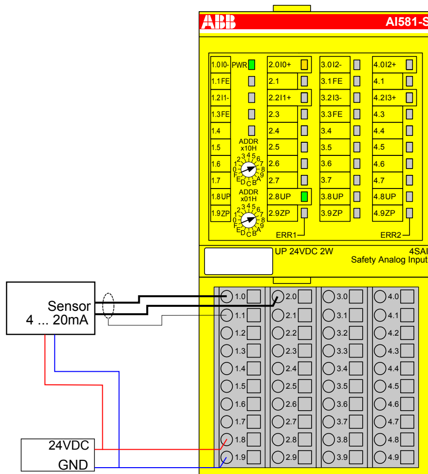
Fig. 58: Circuit example AI581-S, analog sensor (4 ... 20 mA)
