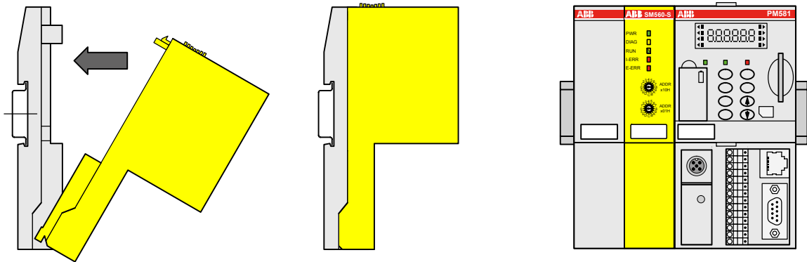
Fig. 7: Assembly instructions
