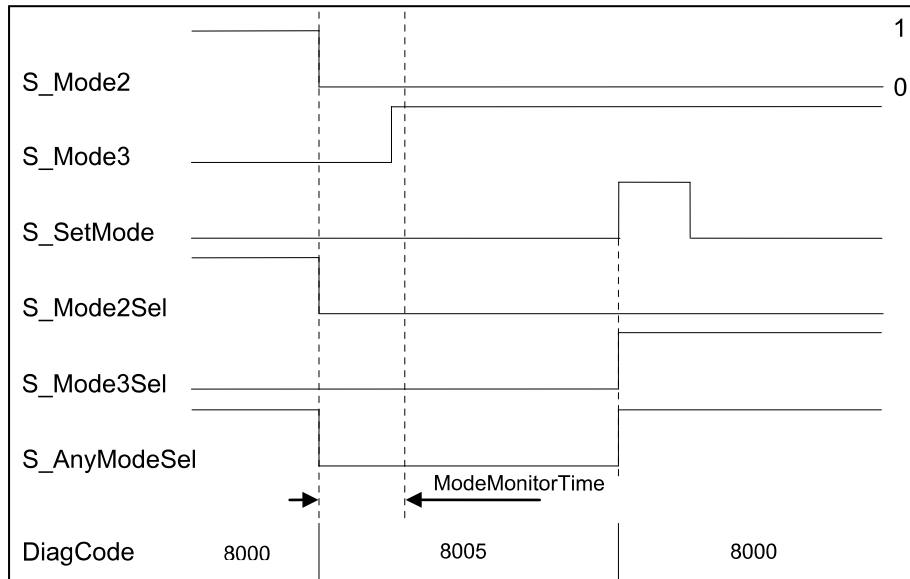
Fig. 86: Timing diagram for SF_ModeSelector, valid change in Mode input with acknowledgment
