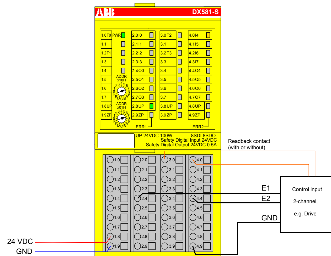
Fig. 48: Circuit example DX581-S, Transistor input (2-channel)
