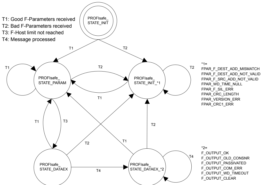
Fig. 112: PROFIsafe F-Device state diagram
