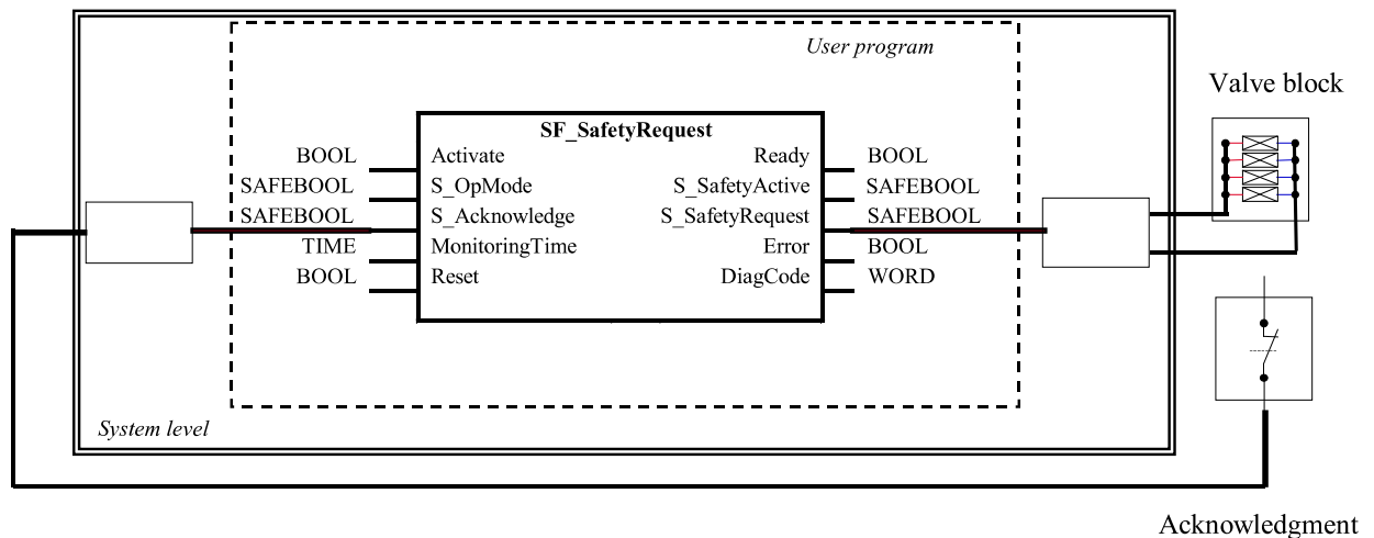
Fig. 106: Example of SF_SafetyRequest
