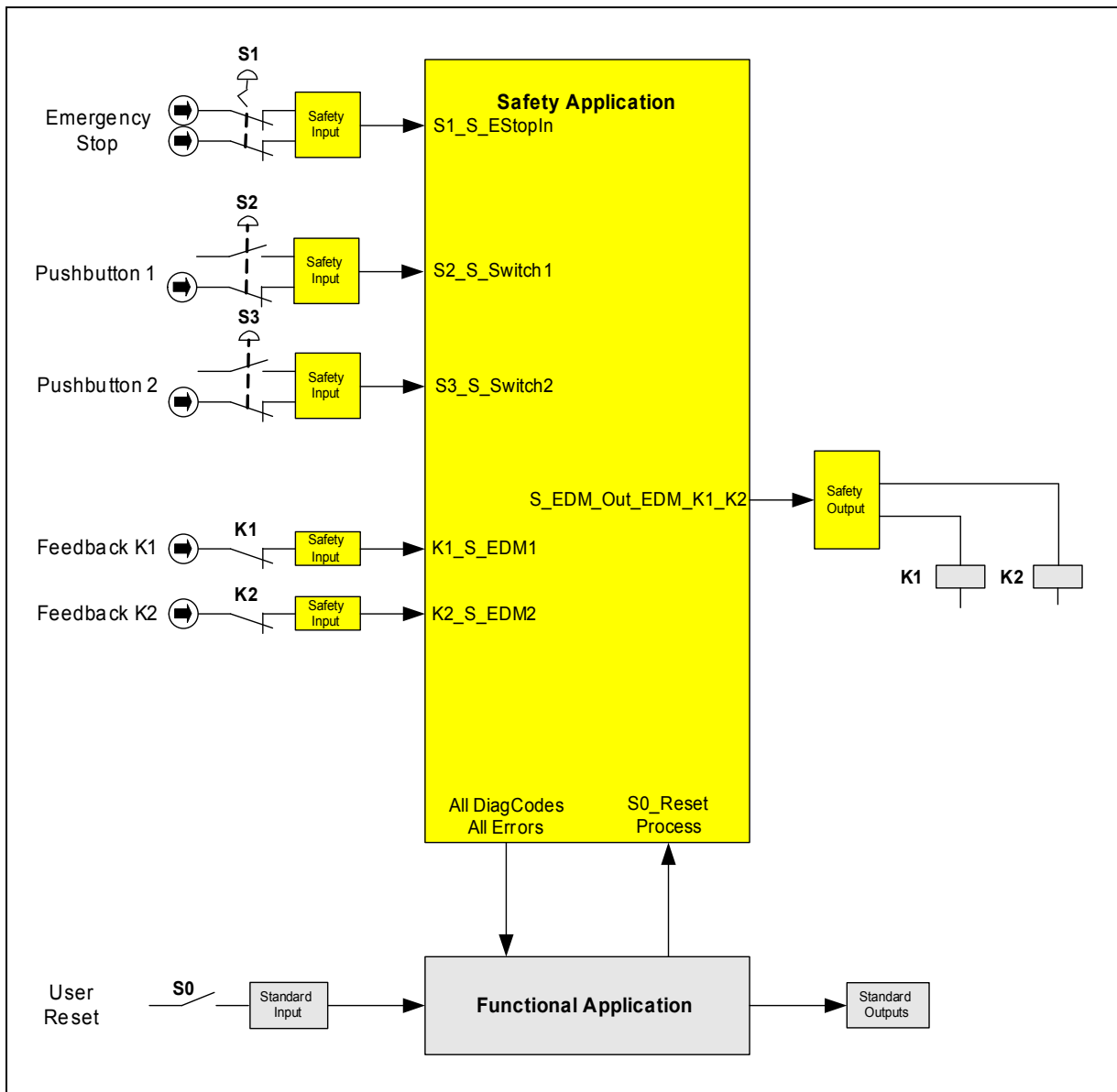
Fig. 127: Graphical overview of the example TwoHand Control with EDM
