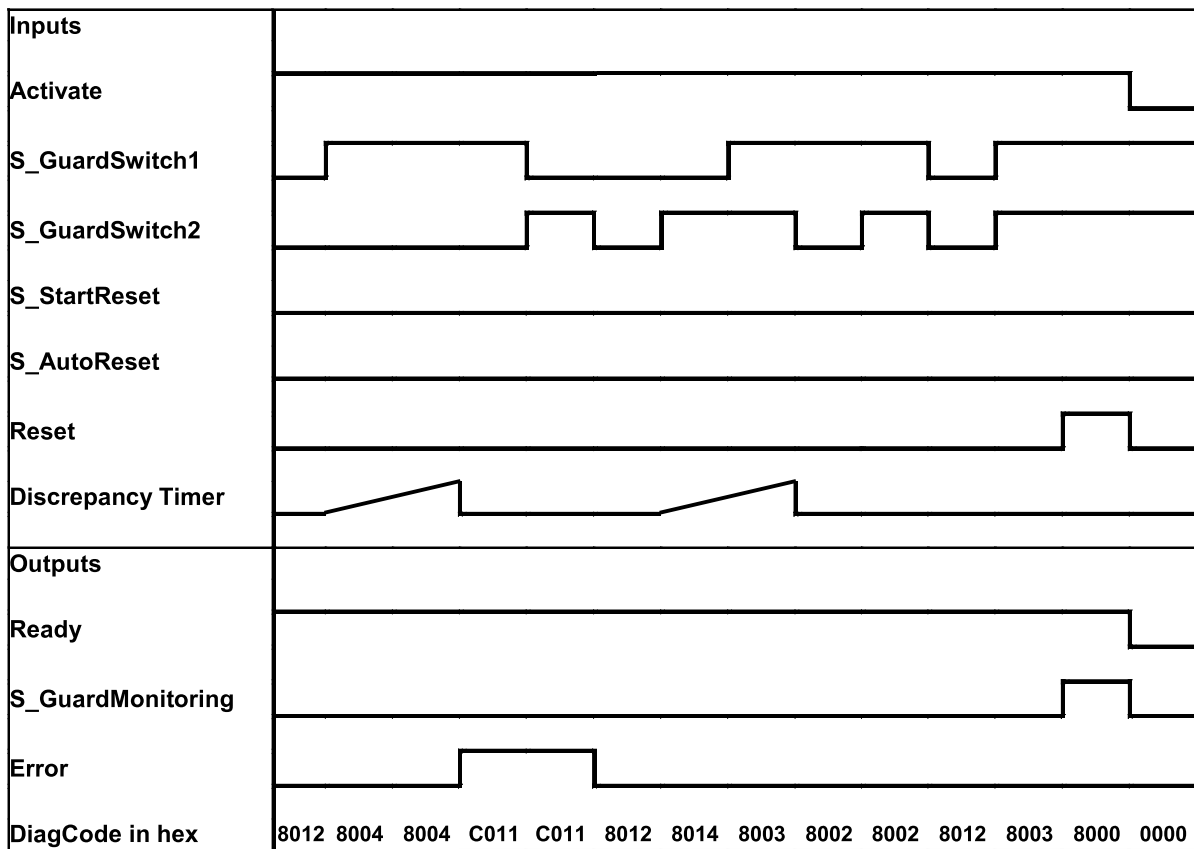
Fig. 95: Timing Diagrams for SF_GuardMonitoring
