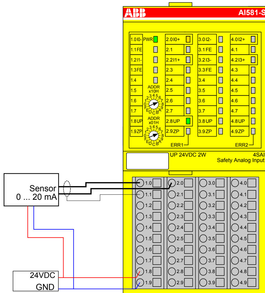
Fig. 56: Circuit example AI581-S, analog sensor (0 ... 20 mA)
