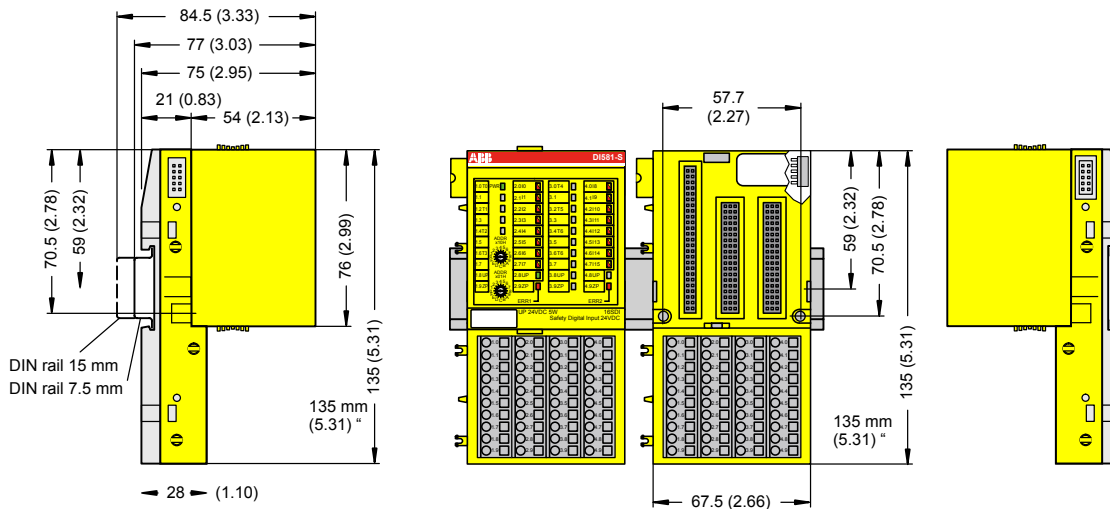
Fig. 22: Dimensions of DI581-S Safety I/O module
