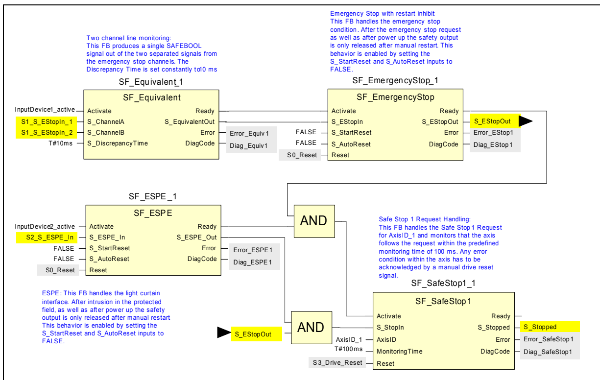
Fig. 123: Program example – Emergency stop with safe stop & equivalent monitoring
