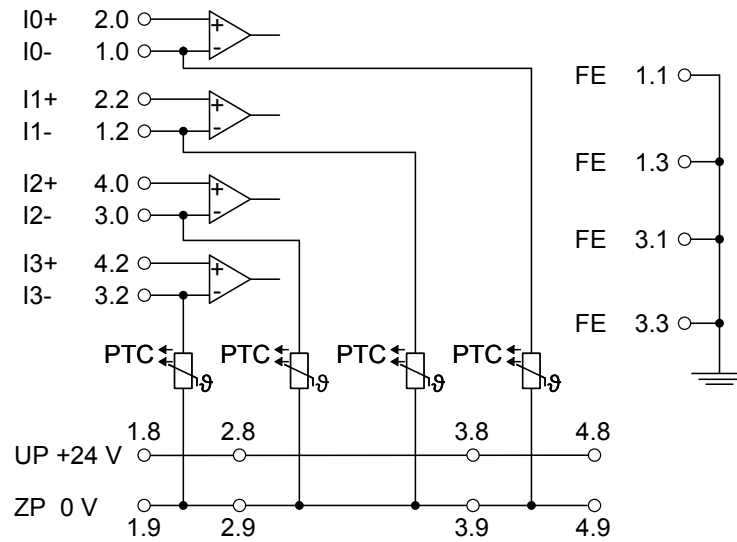
Fig. 54: Example of electrical connections with AI581-S
