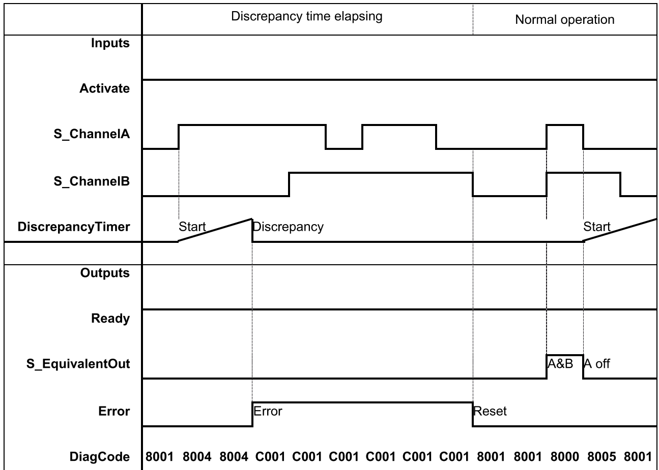
Fig. 84: Typical Timing Diagram for SF_Equivalent
