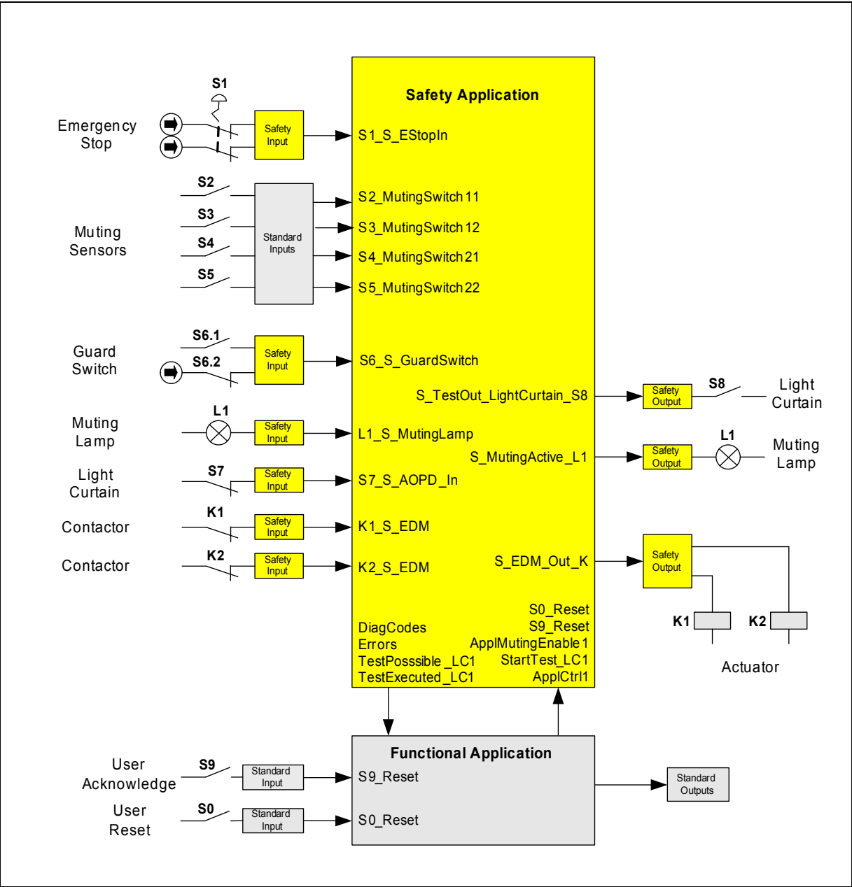
Fig. 124: Graphical overview of the example access protection at a material gate
