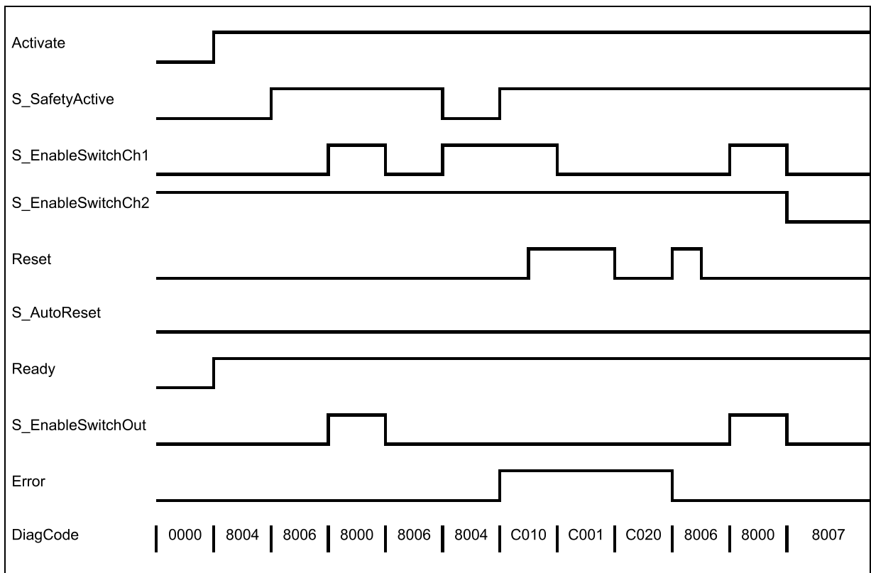
Fig. 104: Timing diagram for SF_EnableSwitch: S_AutoReset = FALSE
