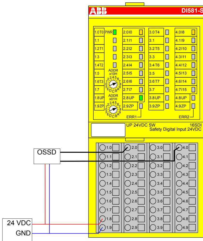
Fig. 29: Circuit example DI581-S, 2-channel OSSD output (with internal tests), external sensor power supply
