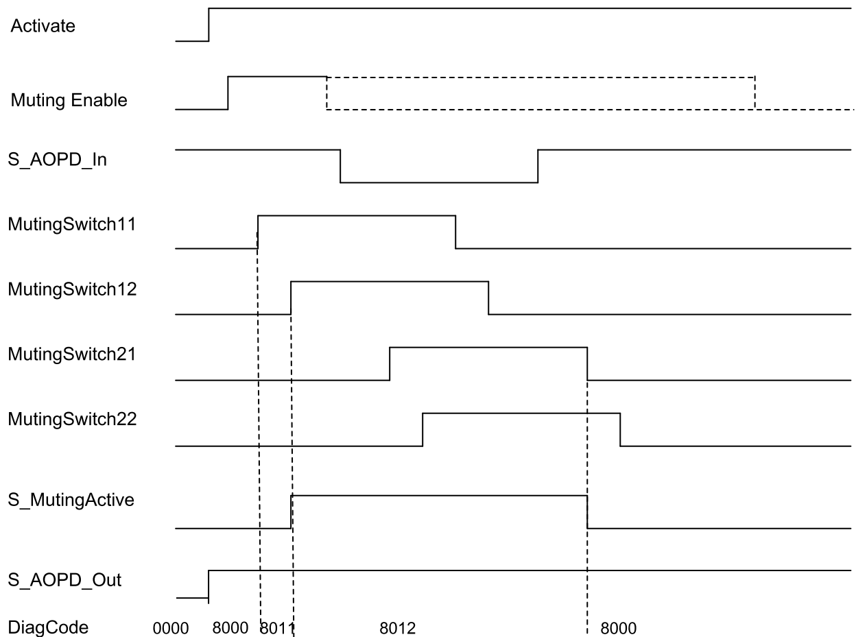
Fig. 100: Timing diagram for SF_MutingSeq with S_StartReset = TRUE
