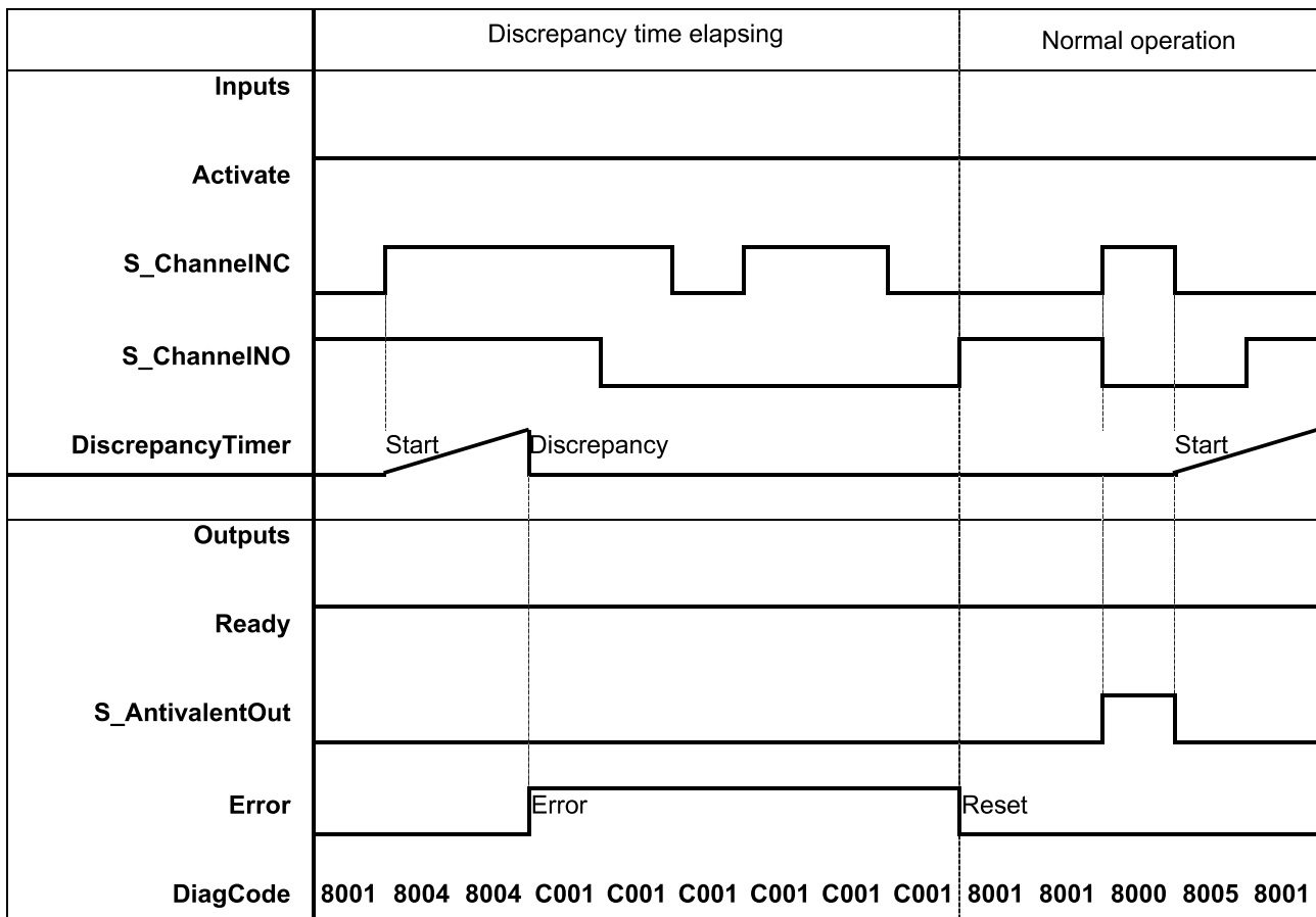
Fig. 85: Typical Timing Diagram for SF_Antivalent
