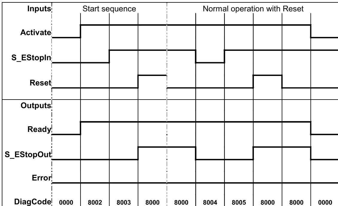
Fig. 89: Timing diagram for SF_EmergencyStop: S_StartReset = FALSE; S_AutoReset = FALSE; Start, reset, normal operation, safety demand, restart
