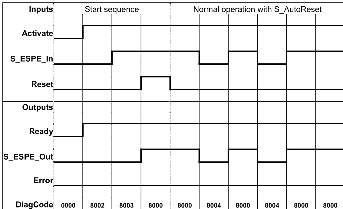
Fig. 94: Timing diagram for SF_ESPE: S_StartReset = FALSE, S_AutoReset = TRUE, Start, normal operation, safety demand, restart
