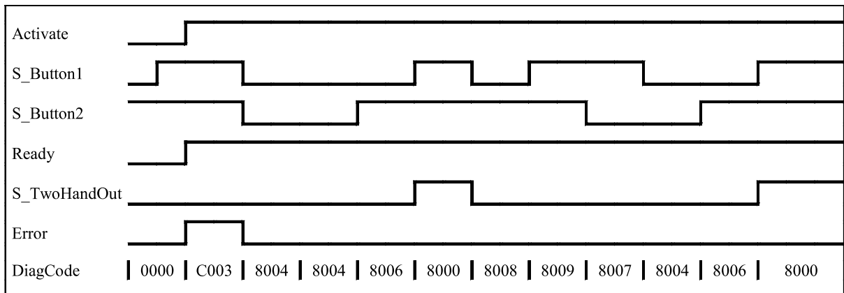
Fig. 96: Timing diagram for SF_TwoHandControlTypell
