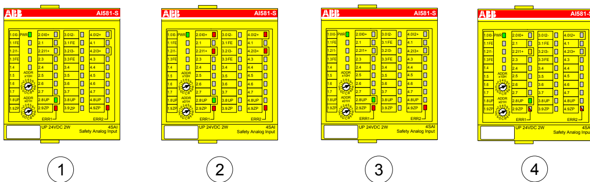
Fig. 16: LED states of Safety I/O modules during start-up (example with AI581-S module)
