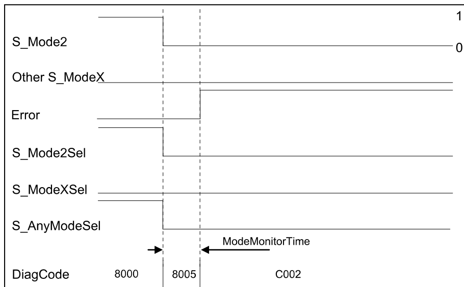
Fig. 87: Timing diagram for SF_ModeSelector, error condition 2 at Mode inputs
