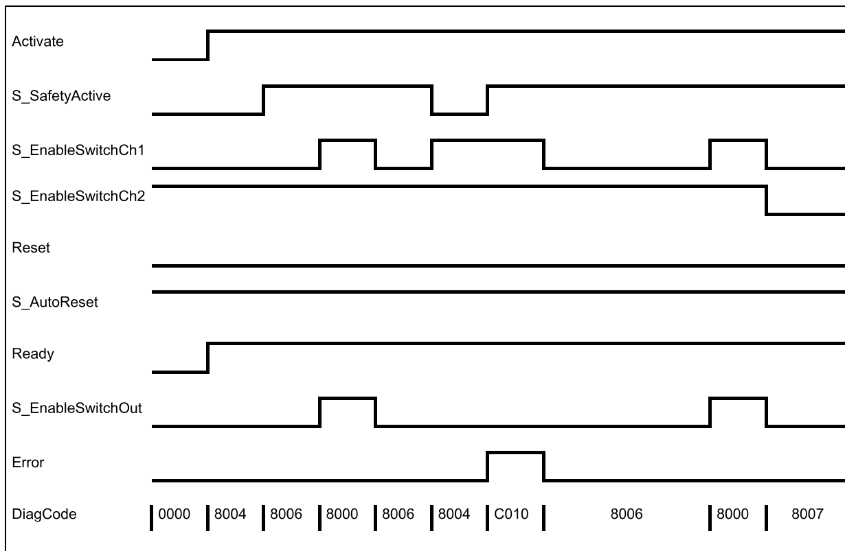
Fig. 105: Timing diagram for SF_EnableSwitch: S_AutoReset = TRUE
