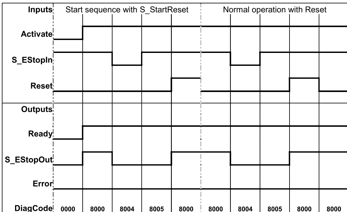
Fig. 90: Timing diagram for SF_EmergencyStop: S_StartReset = TRUE, S_AutoReset = FALSE; Start, normal operation, safety demand, restart
