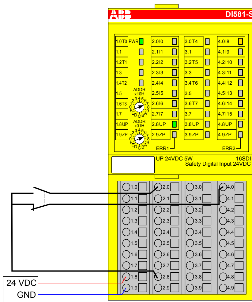
Fig. 28: Circuit example DI581-S, 2-channel sensor (antivalent), 24 V DC
