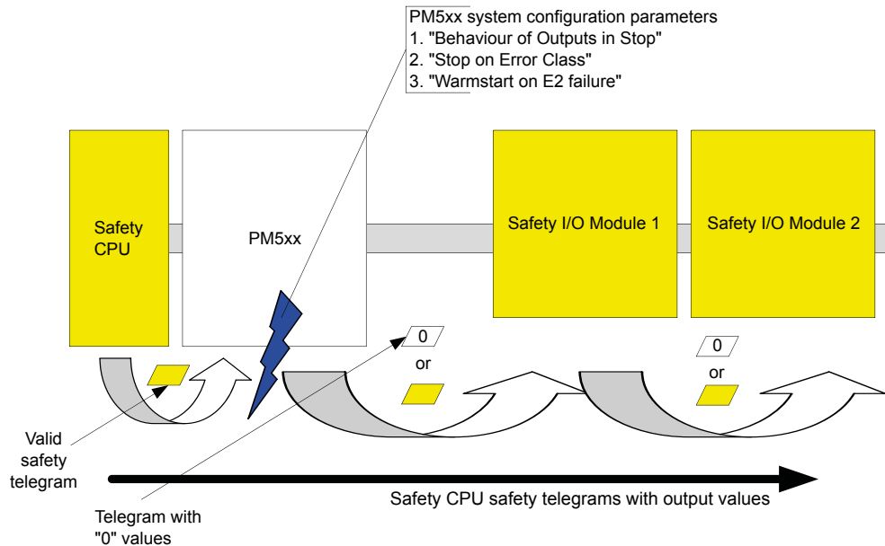
Fig. 13: Overview on how PM5xx system parameter setting influences Safety CPU safety telegram flow
