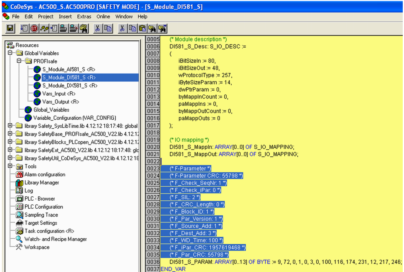
Fig. 74: F-Parameter values in CODESYS Safety V2.3
