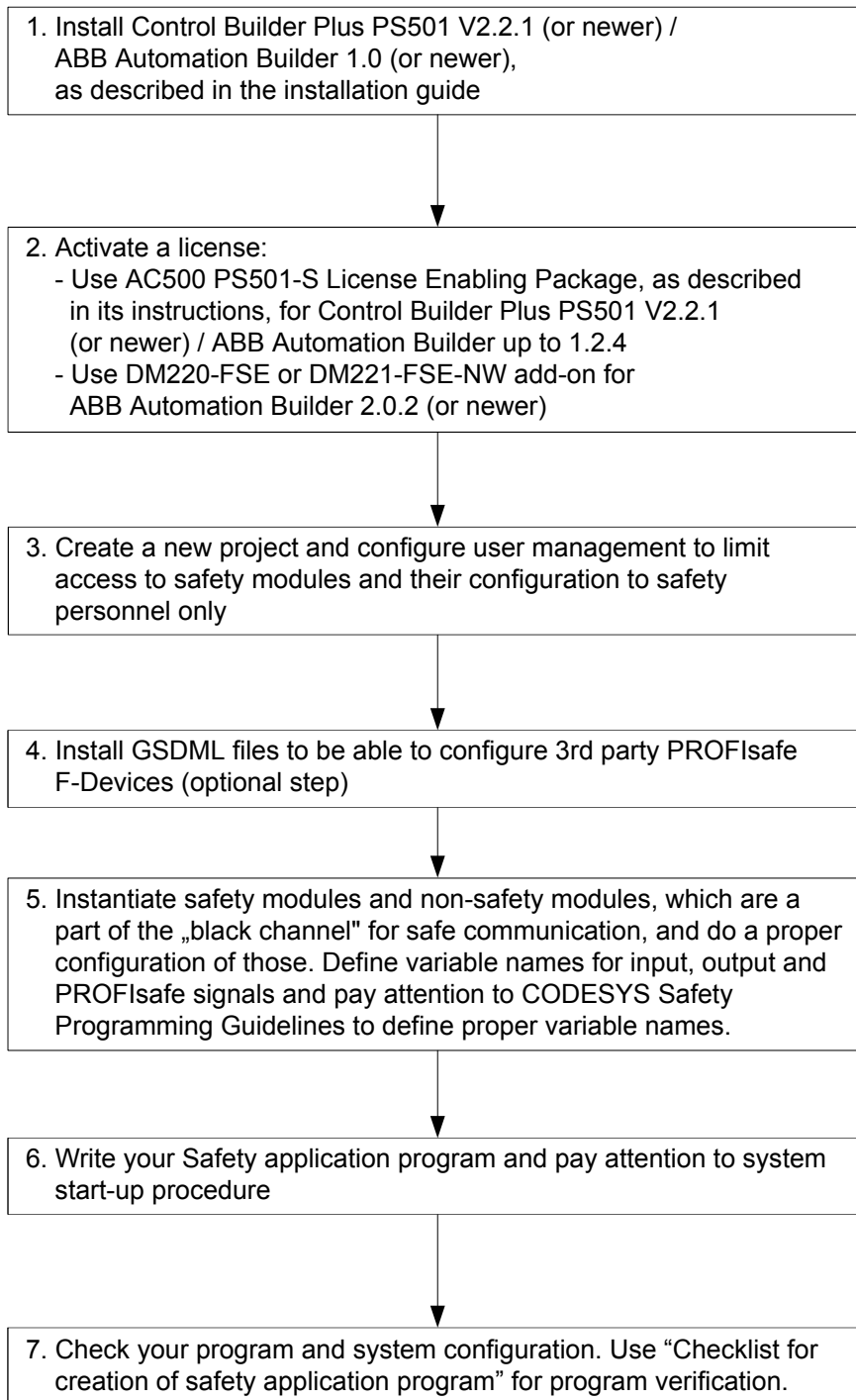
Fig. 64: AC500-S system configuration and programming workflow
