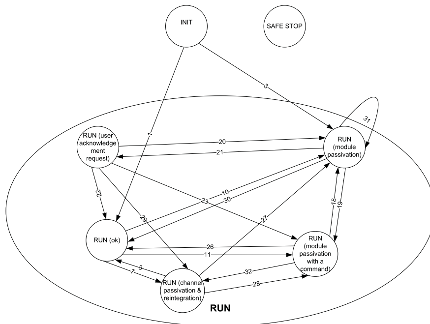
Fig. 15: Overview of transitions in Safety I/O modules (except powering off/on and fatal errors)
