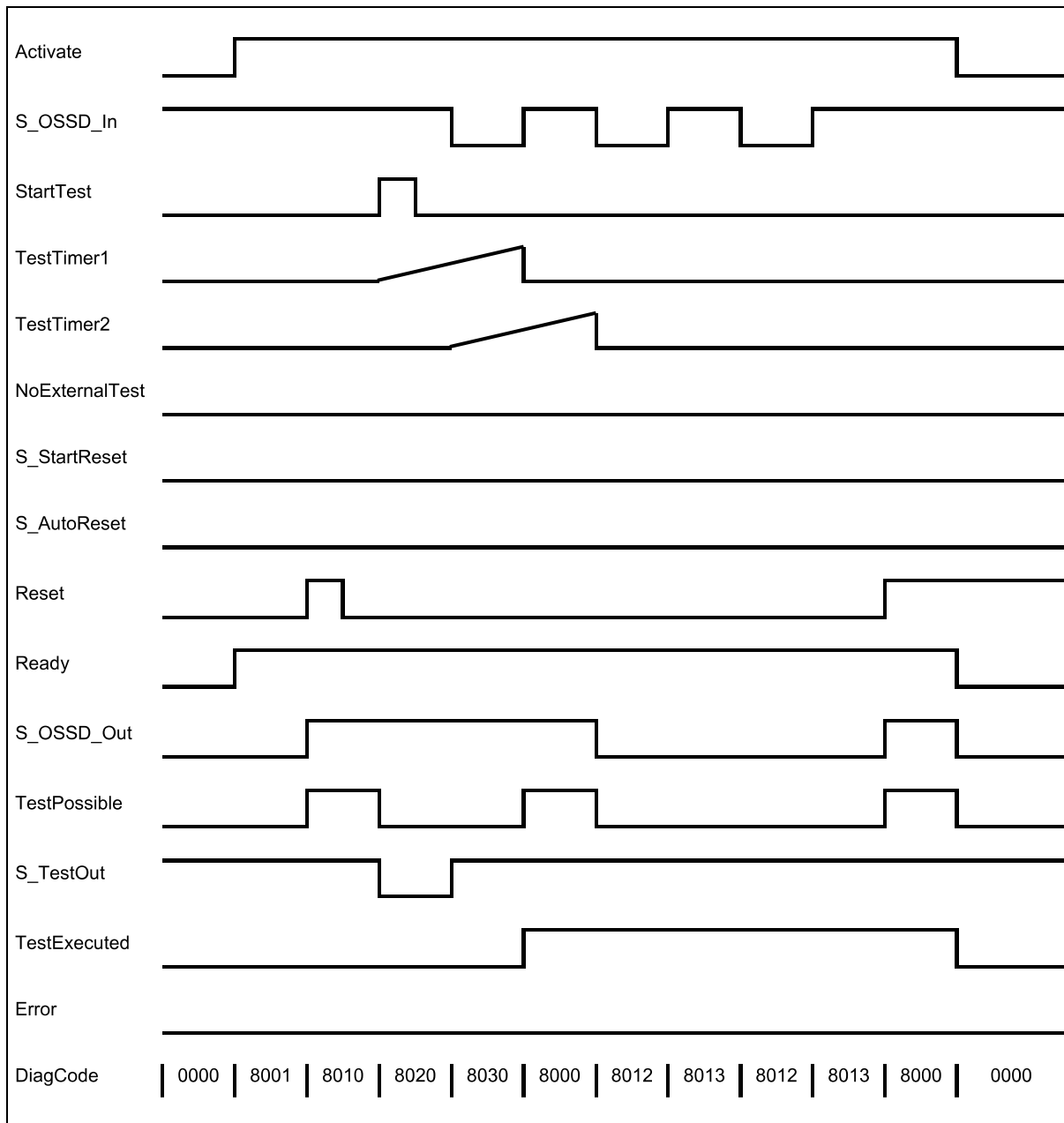
Fig. 99: Timing diagram for SF_TestableSafetySensor
