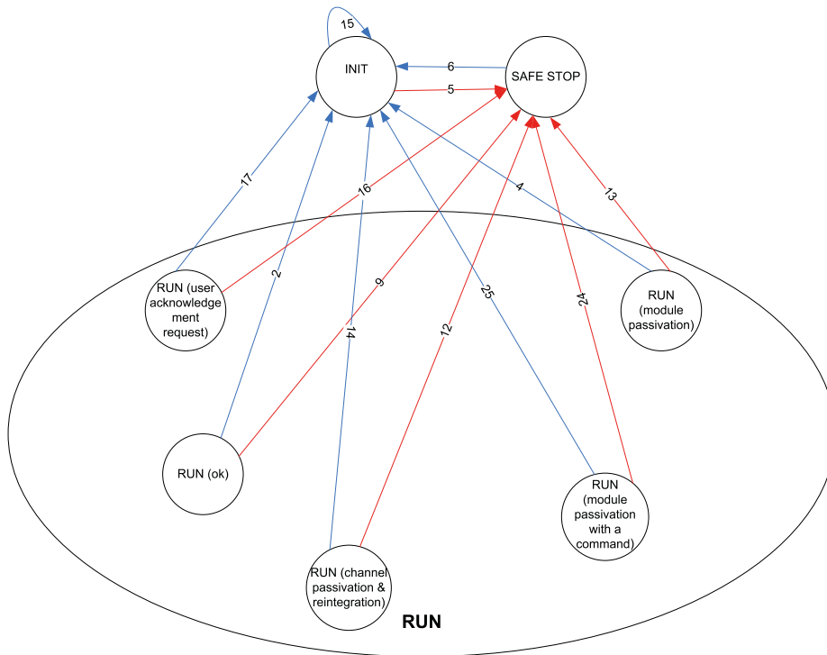
Fig. 14: Overview of transitions related to powering off/on and fatal errors in Safety I/O modules
