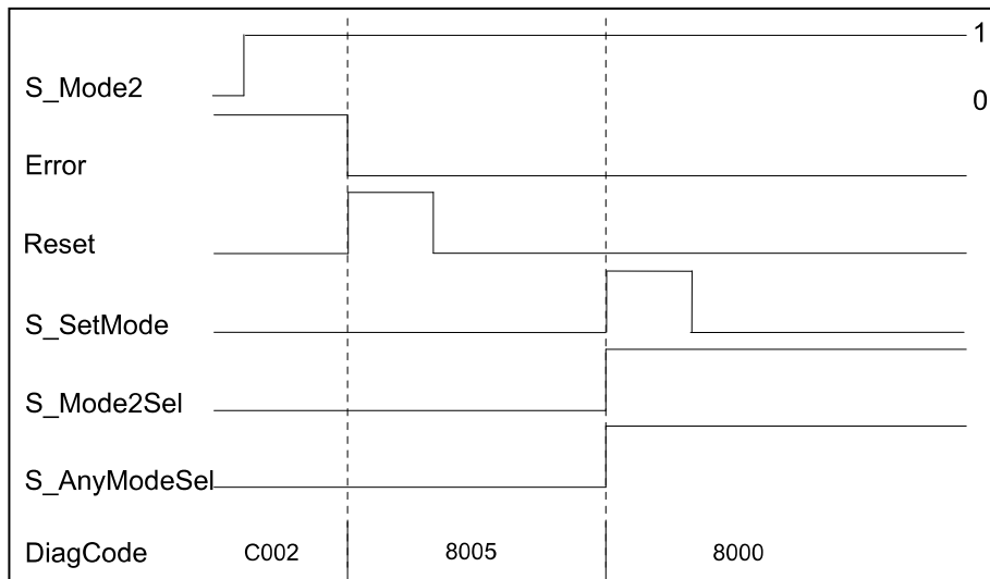
Fig. 88: Timing diagram for SF_ModeSelector, reset of error condition
