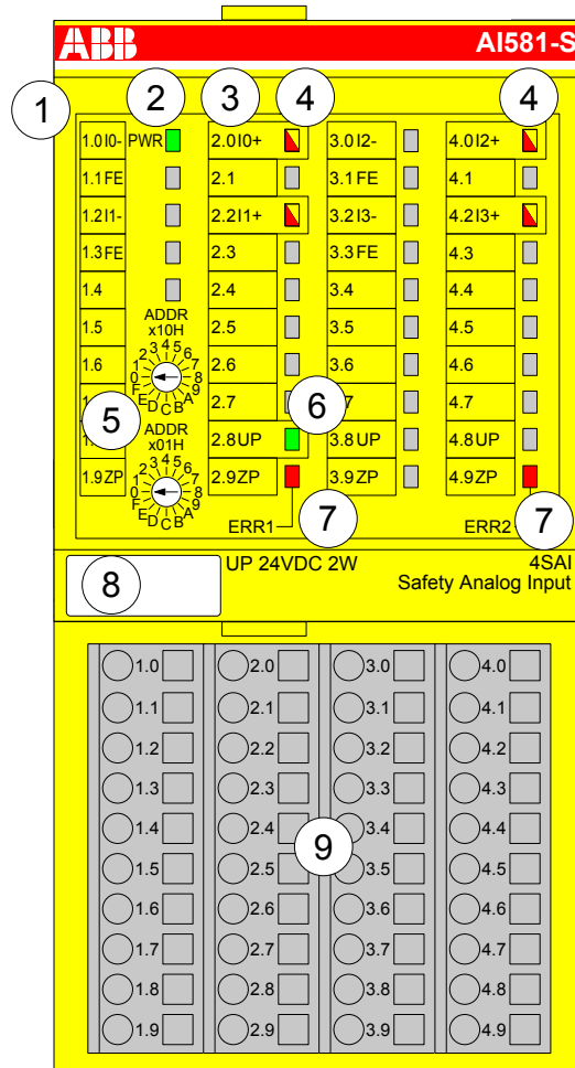
Fig. 50: Safety analog input module AI581-S, plugged on Terminal Unit TU582-S
