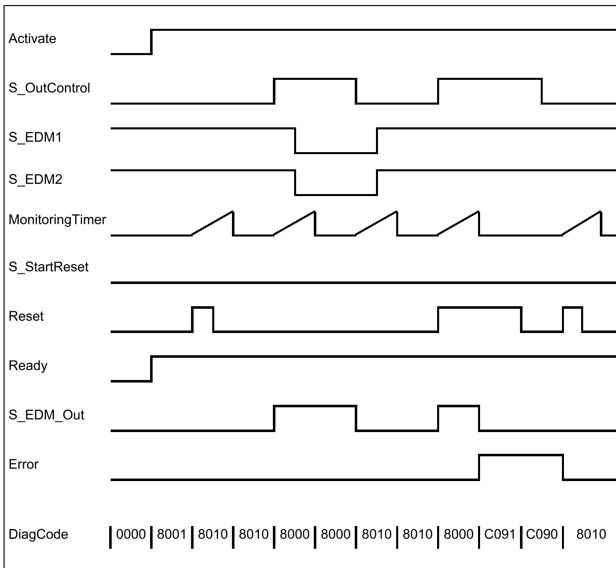
Fig. 110: Timing diagrams for SF_EDM: S_StartReset = FALSE
