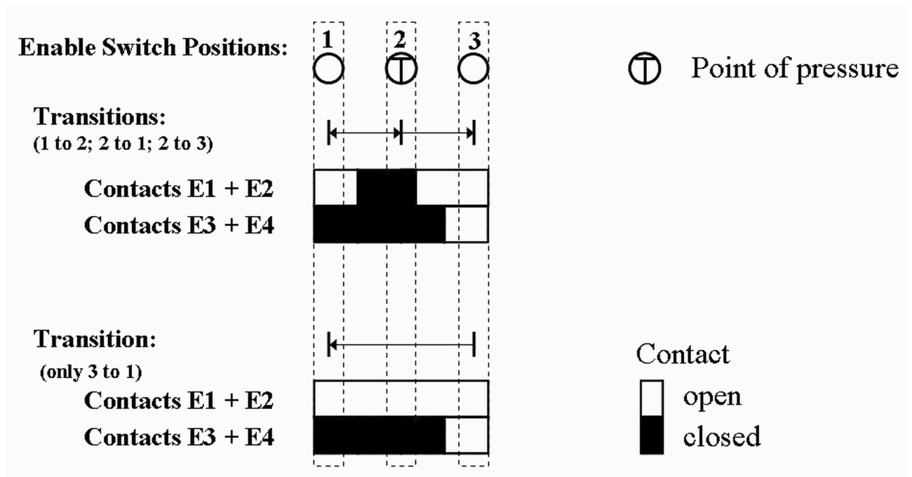
Fig. 103: Switch positions
