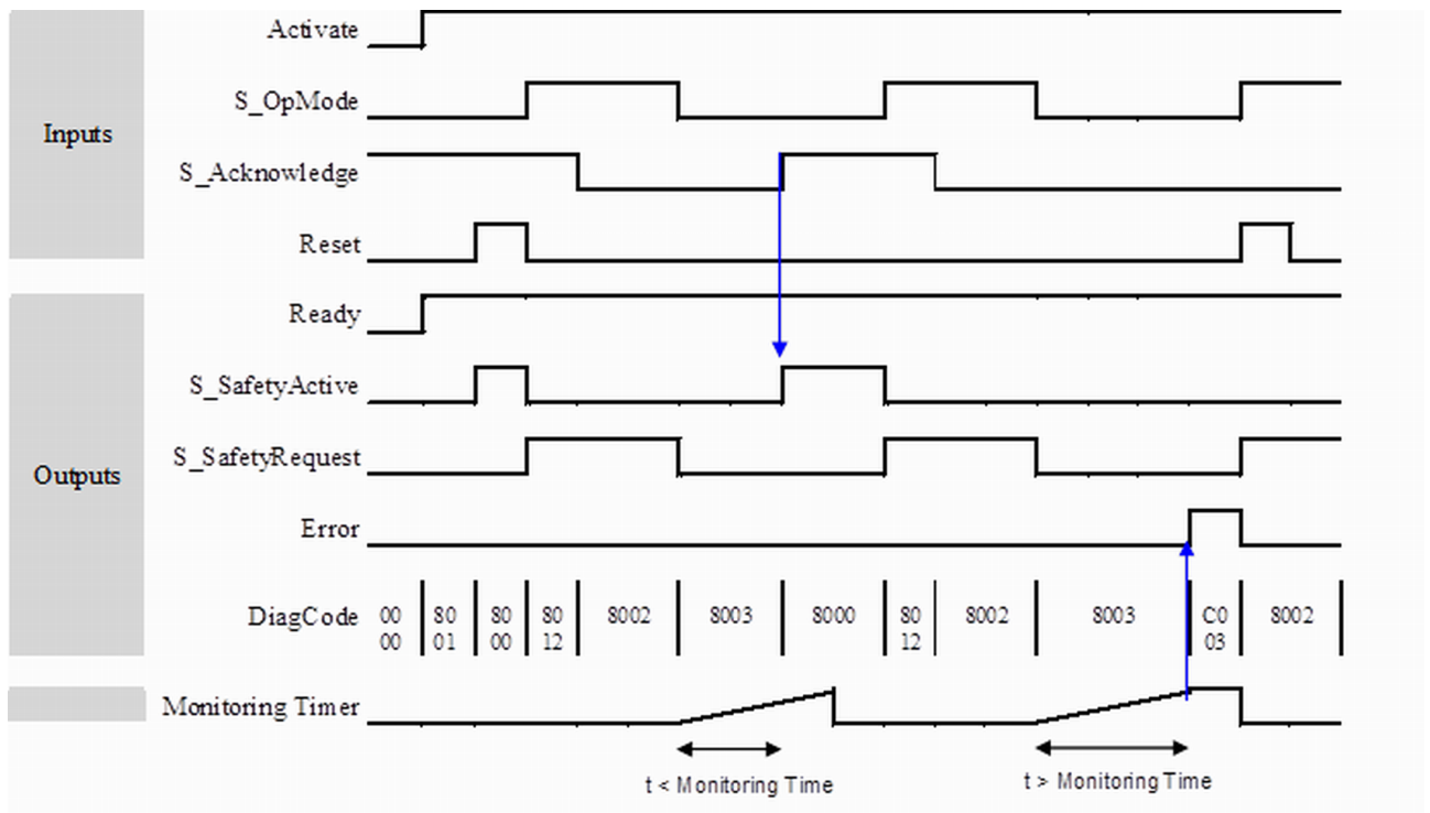
Fig. 107: Timing diagram for SF_SafetyRequest
