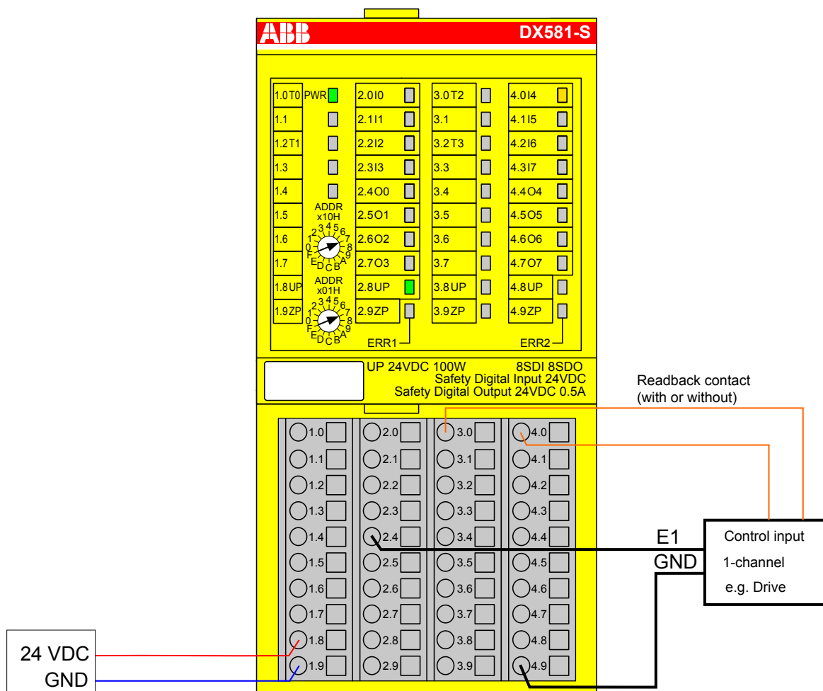
Fig. 47: Circuit example DX581-S, Transistor input (1-channel)
