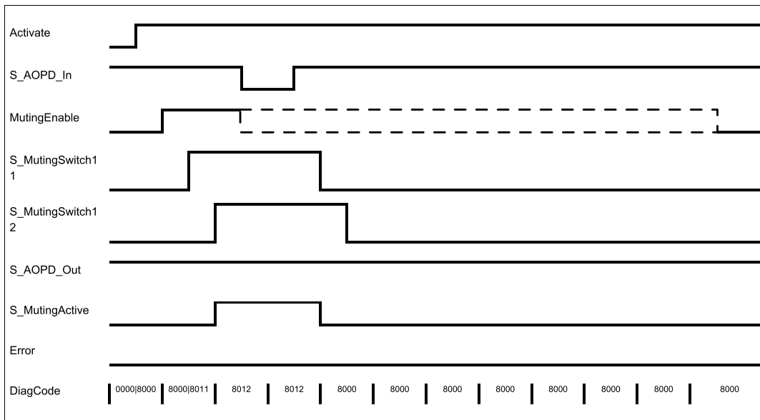
Fig. 102: Timing diagram for SF_MutingPar_2Sensor ( S\_StartReset = TRUE , Reset = FALSE , S\_MutingLamp = TRUE )
