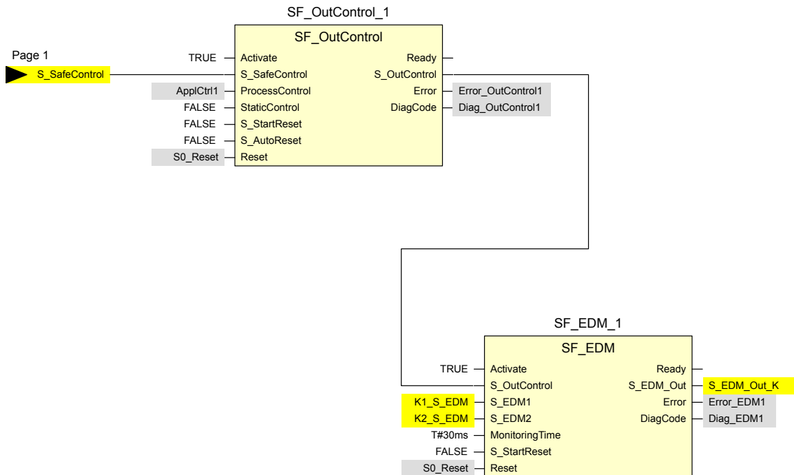
Fig. 126: Access protection at a material gate - Application Program Page 2
