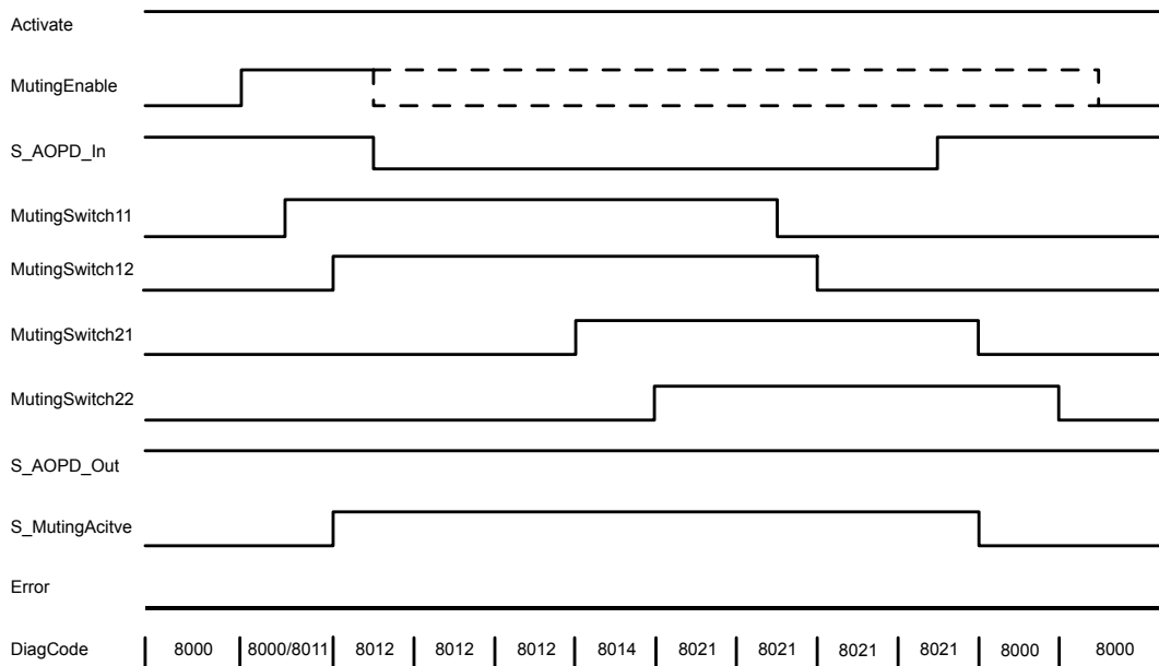
Fig. 101: Timing diagram for SF_MutingPar
