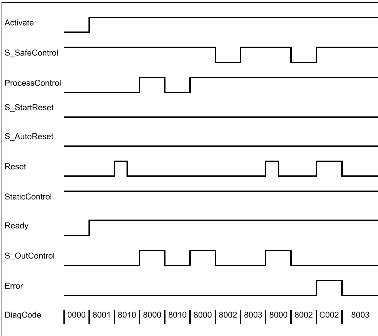
Fig. 108: Timing diagram for SF_OutControl: S_StartReset = FALSE
