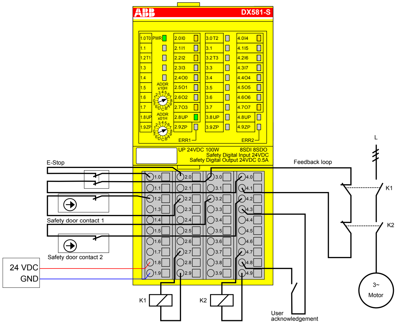
Fig. 49: Application example with DX581-S
