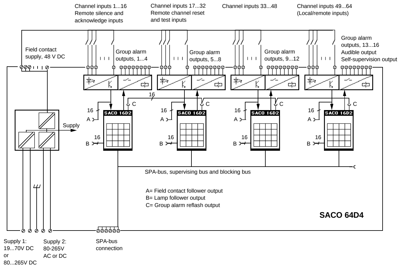
Fig. 1 Block diagram
