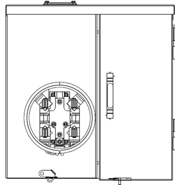
FRONT LAYOUT VIEW (DOORS CLOSED CONDITION)
