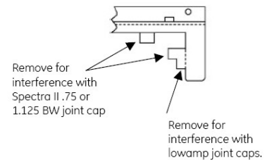
Figure 2. Break-Off Tabs
