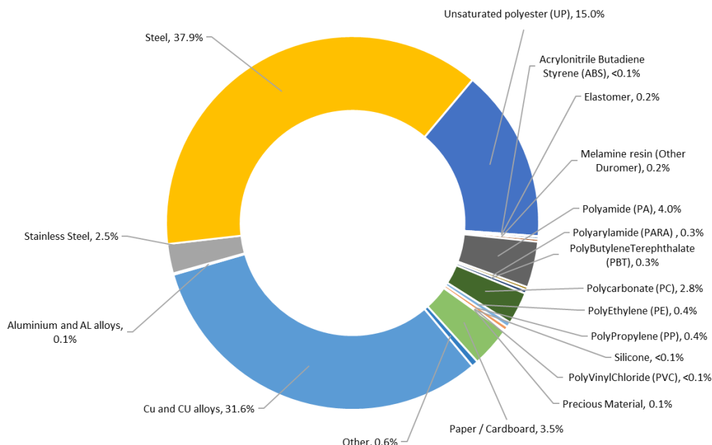
Figure 1: Composition of E1.2 B-A/N-A/S-A 1200A-3P Circuit Breaker
