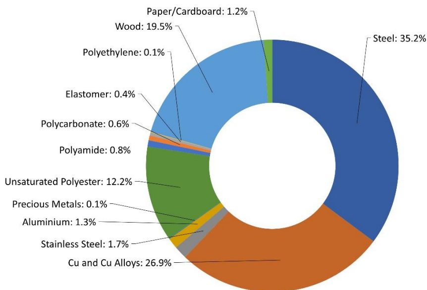
Figure 1: Composition of DR EGL F1 65 kA 3P to E2.2 IEC
