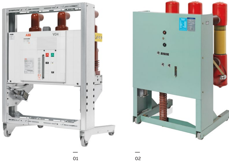
— 01 VD4 circuit breaker installed on the new A-truck
