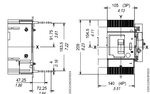
Rear flat horizontal - HR
