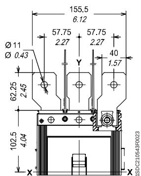
Front extended spread - ES
