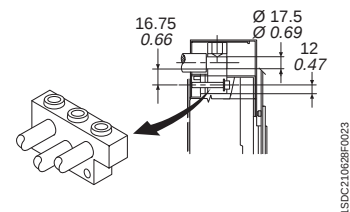
For rear Cu/Al cables - FCCuAl (IP20 high terminal covers included in the supply)
