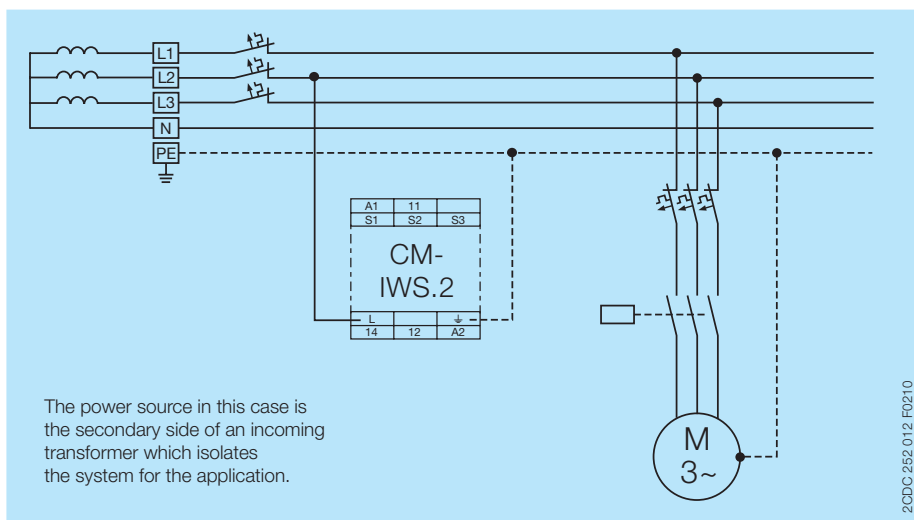
Earth fault / insulation resistance monitoring of a 4-wire IT AC system
