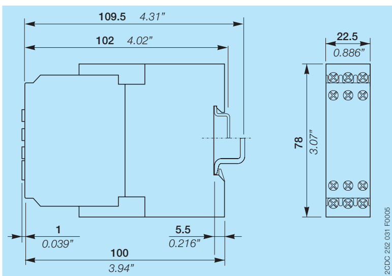
CM-IWS.2 - Insulation monitoring relay
