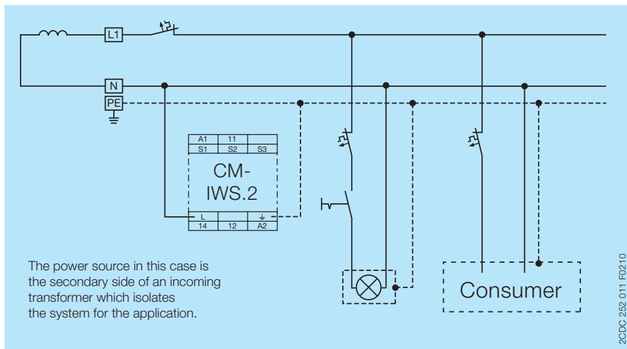
Earth fault / insulation resistance monitoring of an unearthed 2-wire IT AC system
