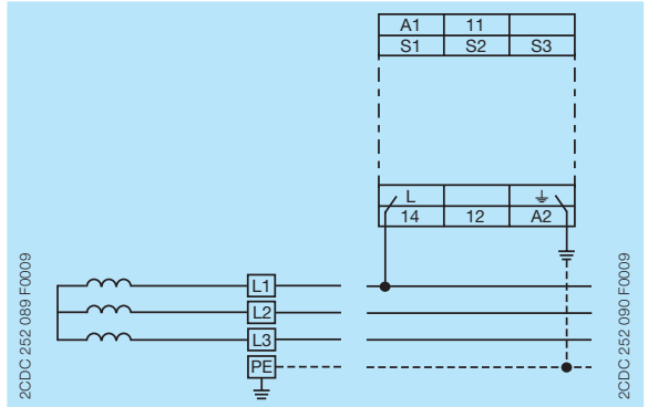
3-wire AC system
