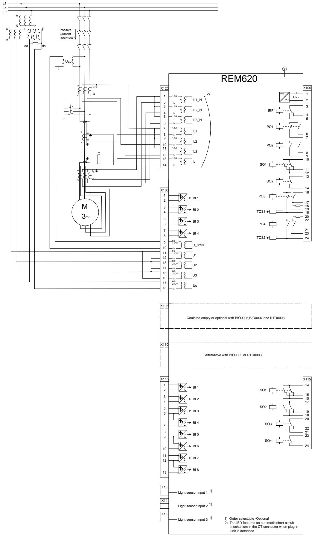
Figure: REM620 ME201 Connection diagram for standard modules ( For Flux-balance based differential protection)
