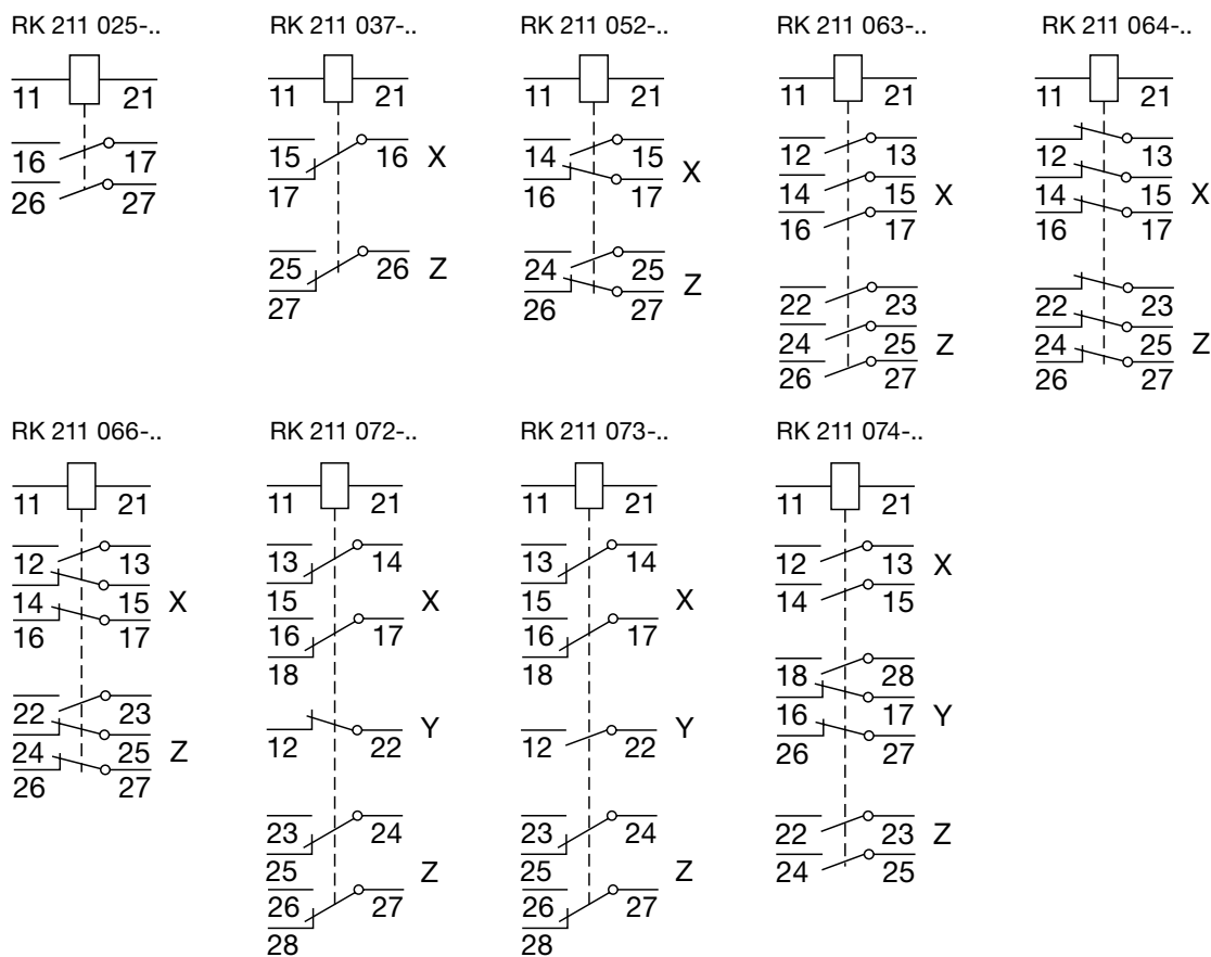
Letter selection table, DC rated voltage V
