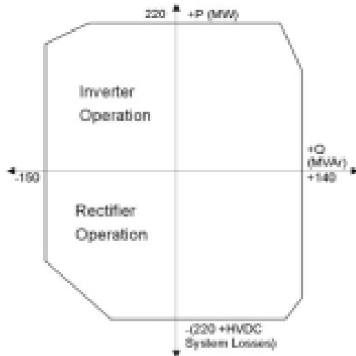
Figure 4 Active and Reactive Control Range
