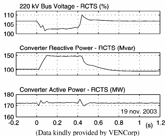
Figure 13 AC fault on Victorian network
