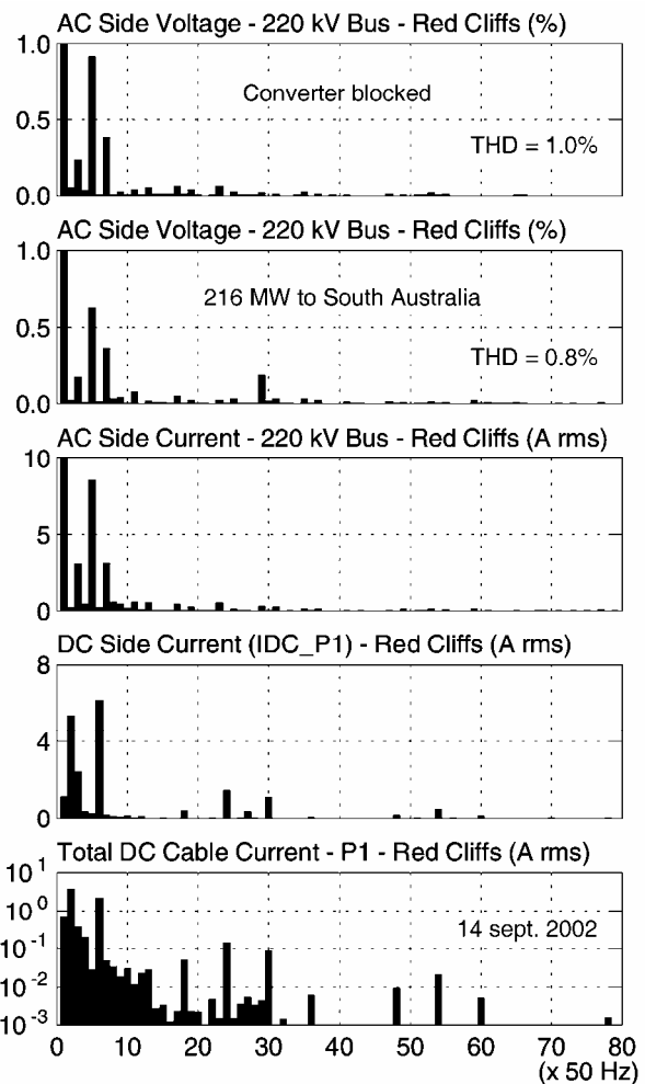
Figure 8 Typical spectra for AC side and DC side harmonics
