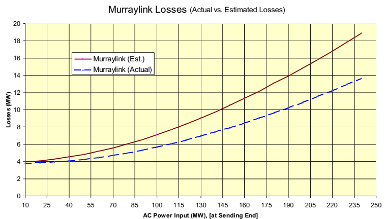
Figure 9. Murraylink Actual and Estimated Losses
