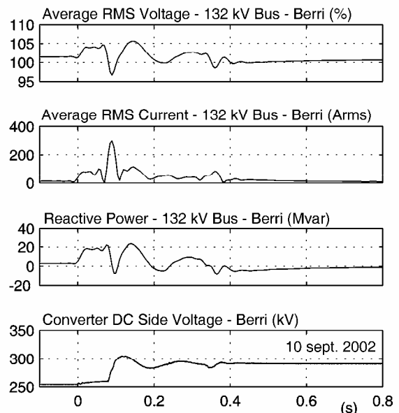
Figure 11 Converter deblocking
