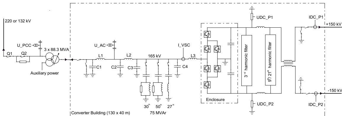
Figure 5. Single Line Diagram of Murraylink
