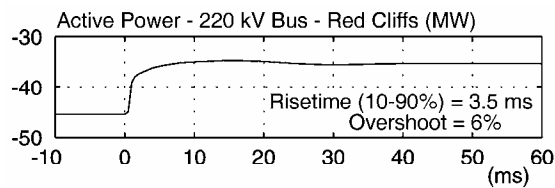
a) Step response of the active power controller
