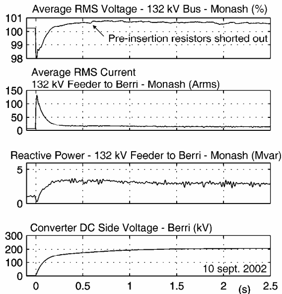
Figure 10 Converter energisation
