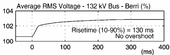
b) Step response of the AC voltage controller
