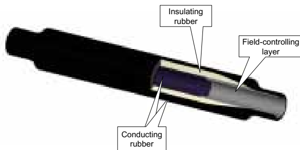
Figure 6. Prefabricated DC joint
