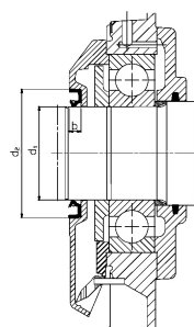
Radial seal
