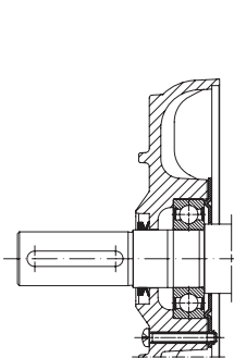
Motor sizes 71 - 132
