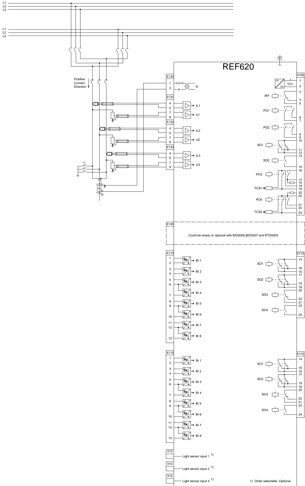
Figure: REF620 FE202 Connection diagram for standard modules
