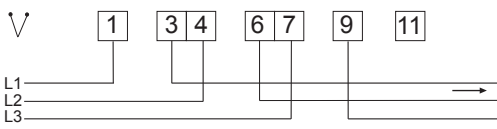
Terminal block B23
