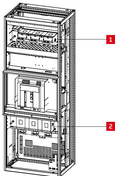
Figure 2-48 Positions for optional earthing switch solutions 1 Position shown for upper earthing switch 2 Position shown for lower earthing switch
