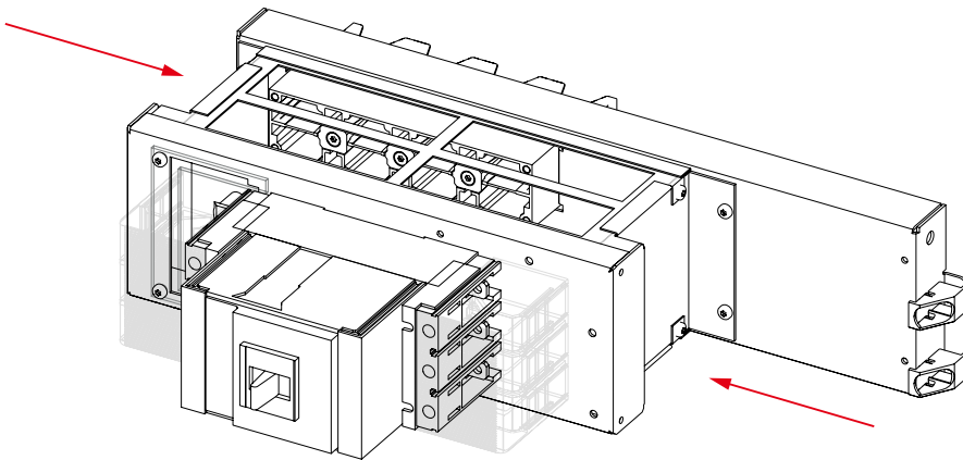
Figure 10-01 Plug-in modules integrated handles
