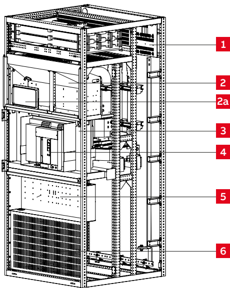
Figure 2-53 MNS Rear ACB section with tubular copper bar
