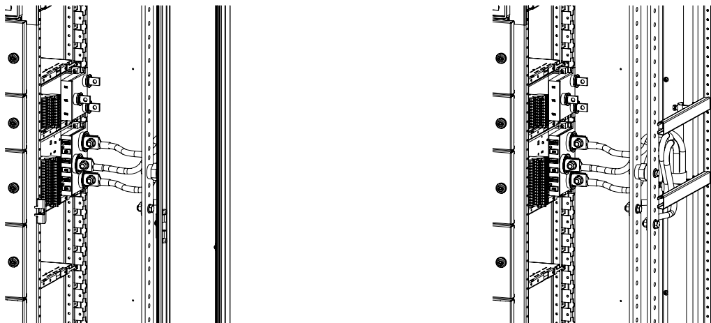
Figure 4-65 Example of cable runs, withdrawable module size ≥ 4E
