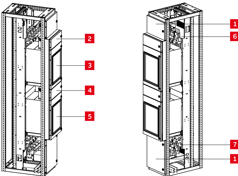
Figure 2-51 MNS Front access switchgear with double stacked circuit breakers (CB)
