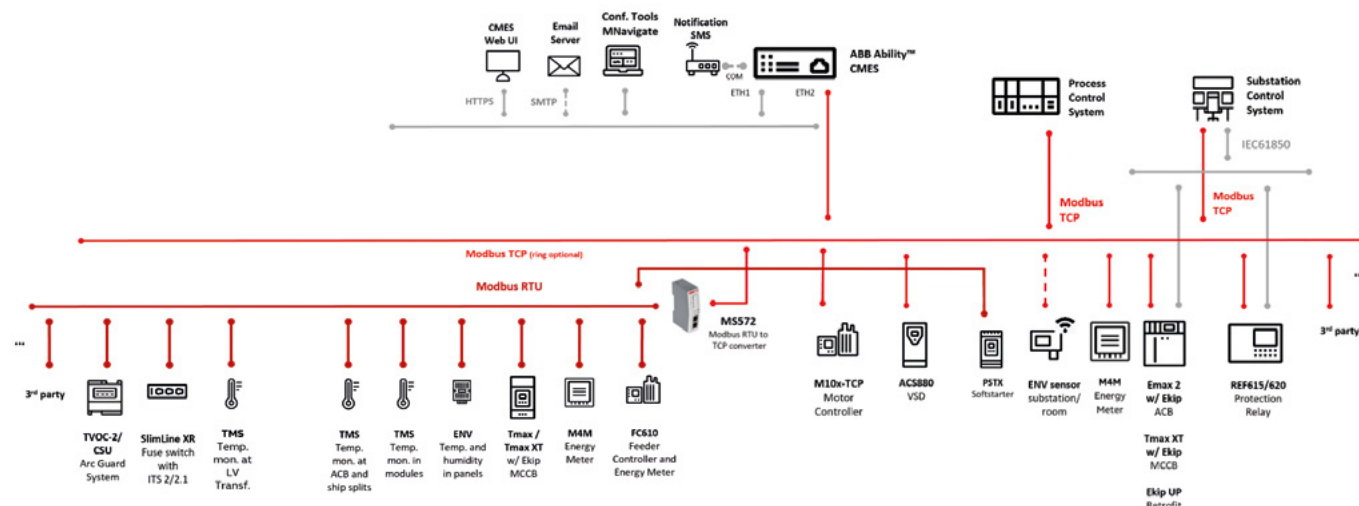
Figure 7-03 MNS condition monitoring with ABB Ability™ CMES
