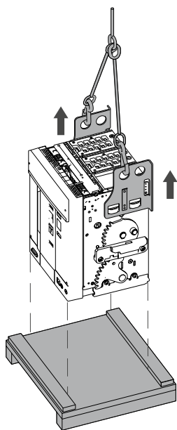
Figure 4-80 Top lifting of ACB withdrawable part
