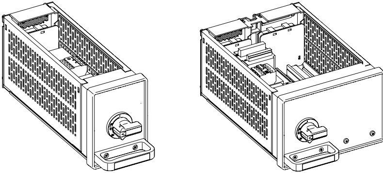
Figure 2-84 Examples of 8E/4 and 8E/2 modules
