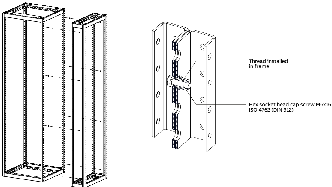
Figure 4-16 Connection points (threads installed in frame) with detail of connection
