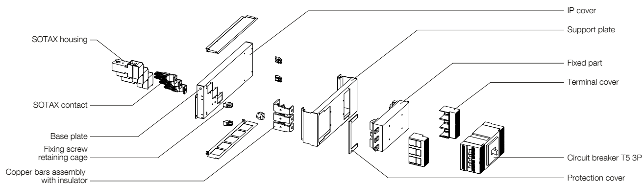
Figure 2-72 Exploded view of plug-in module with copper connection to main contacts
