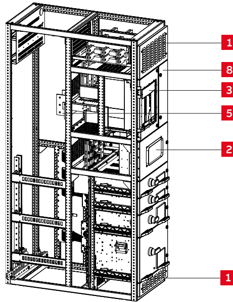
Figure 2-57 MNS Rear access combined ACB and withdrawable modules
