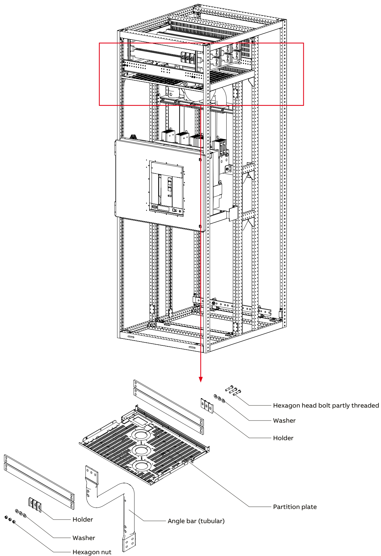
Figure 2-31 MNS Rear ACB tubular copper bar connection to main busbar
