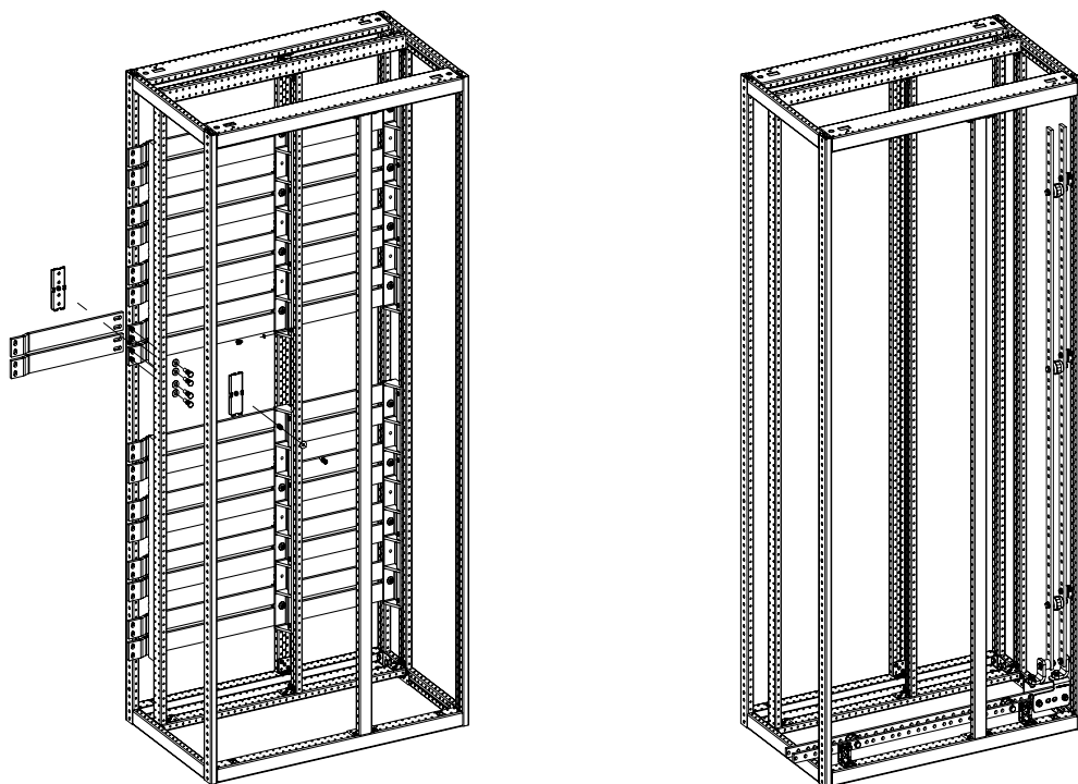
Figure 2-27 Main busbar arrangement (left), N/PEN front distribution (right)
