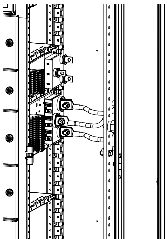
Figure 4-74 Example of cable runs, withdrawable module size \geq 4E
