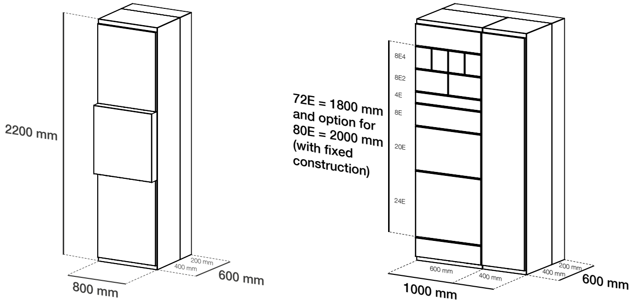
Figure 2-15 Incoming / outgoing circuit breaker section (left), outgoing section (right)
