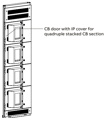
Figure 2-25 MNS Rear quadruple stacked section (example)
