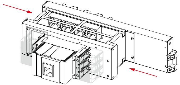
Figure 2-75 Ergonomic design for improve module handling. The module support plate is designed with handles on both sides.
