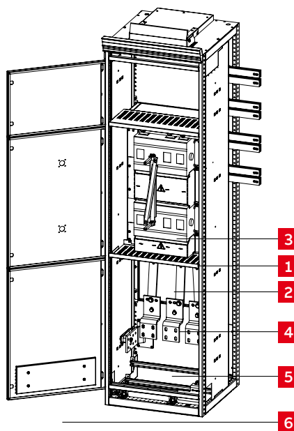
Figure 2-59 Switch-disconnector with earthing switch
