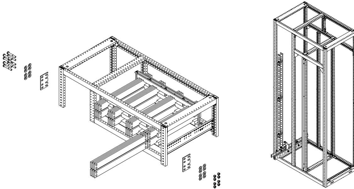
Figure 2-29 MNS Rear main busbar arrangement (left), PE/N/PEN rear distribution (right)
