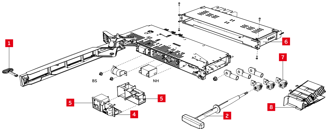
Figure 2-80 Exploded view and optional accessories of XR00
