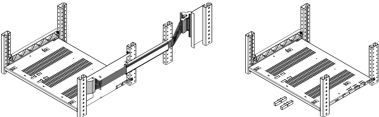
Figure 2-89 MNS Rear withdrawable module compartment for unit size 4E...24E (right), with control plug system (left)
