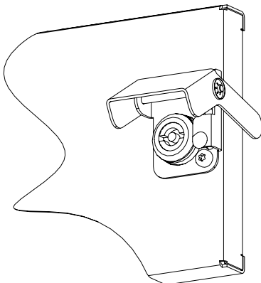
Figure 6-33 Lock covers for full size withdrawable modules
