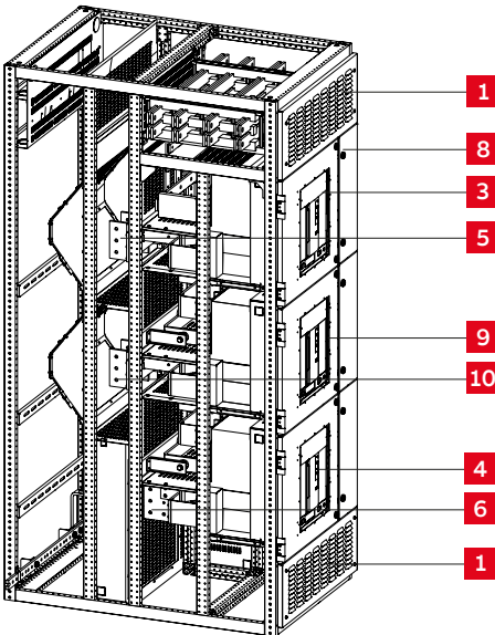
Figure 2-55 MNS Rear access triple stacked ACB
