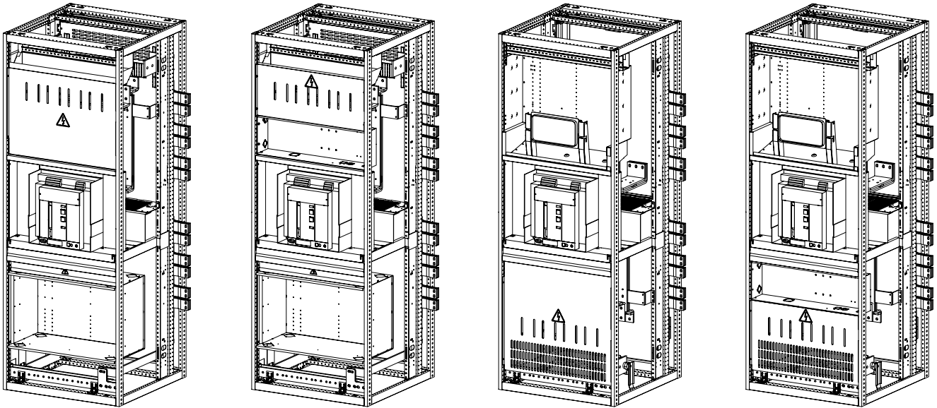
Figure 2-49 Sections with cable top entry (left) and bottom entry (right)
