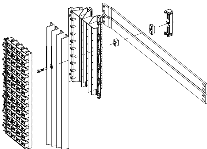
Figure 2-36 Distribution bars. The right hand side shows a detailed view
