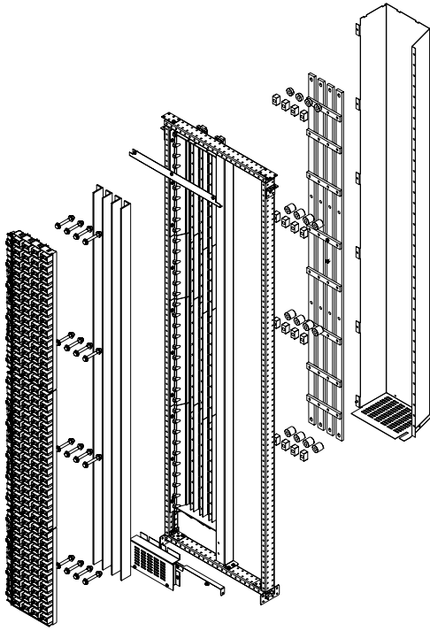
Figure 2-40 MNS Rear distribution bars with MFSW
