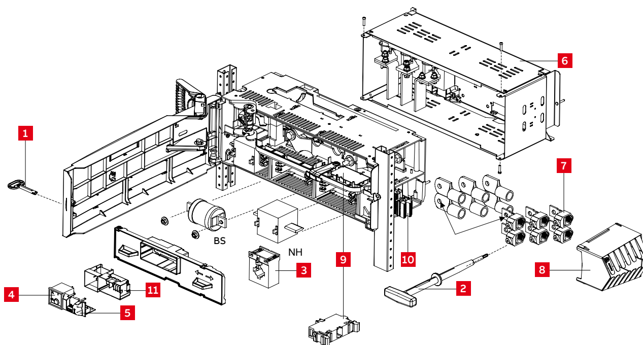
Figure 2-82 Exploded view and optional accessories of XR2-3
