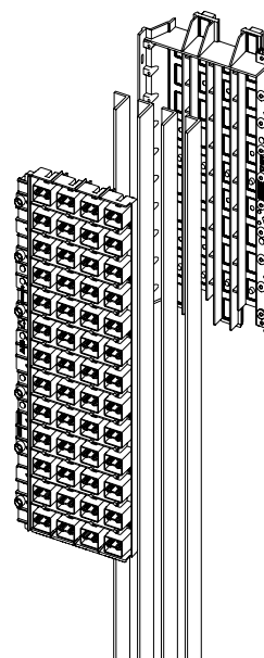
Figure 2-35 Exploded view with front and rear MFSW components and the distribution bars
