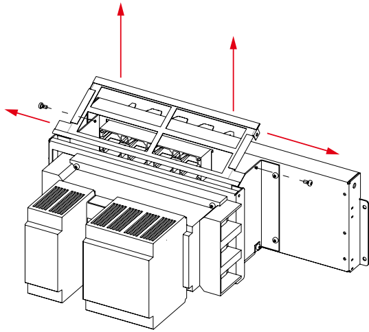
Figure 2-74 IP cover clip for all modules up to 250 A. To remove undo screws on left and right side and flip cover up, same is applicable for lower cover. Re-fitting is the reverse procedure.
