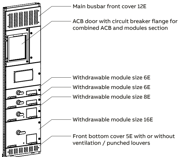
Figure 2-26 MNS Rear combined ACB and withdrawable module section (example)
