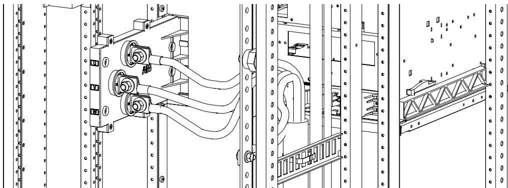
Figure 4-76 Example of MNS Rear cable runs, module size \geq 4E
