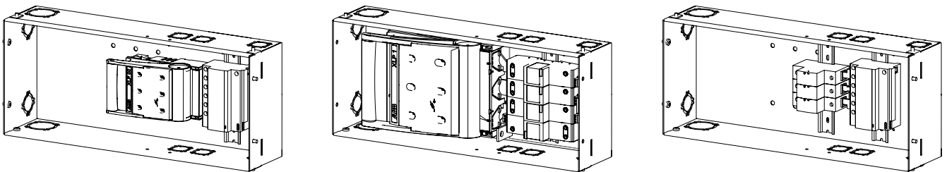
Figure 2-50 SPD with fuse backup protection XLP0 (left), XLP1 (middle) and MCB backup protection (right)
