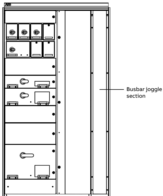
Figure 8-05 Switchgear extension with busbar joggle section
