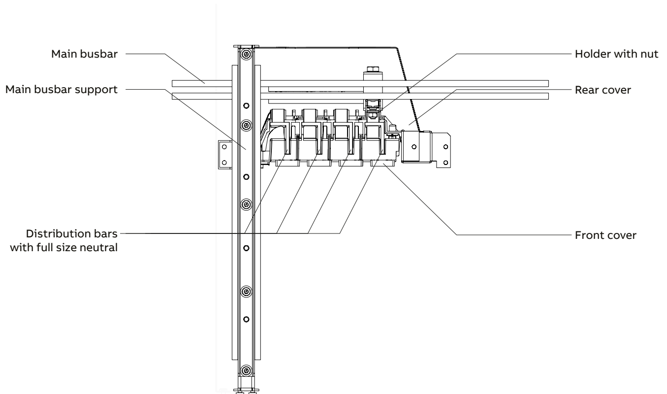
Figure 2-40 MNS Rear distribution bars with MFSW
