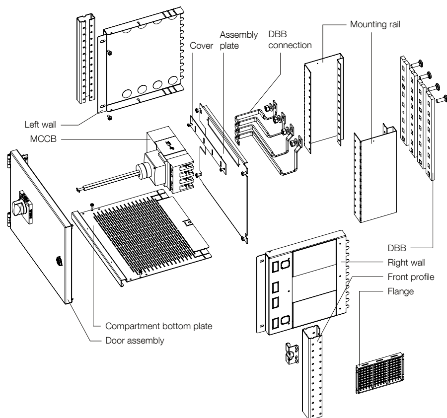
Figure 2-60 Fixed module size 12E
