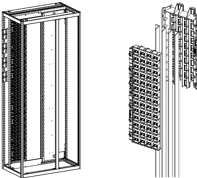
Figure 2-68 Multi-Function Separation Wall (MFSW) in section
