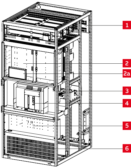
Figure 2-52 MNS Rear ACB section configuration
