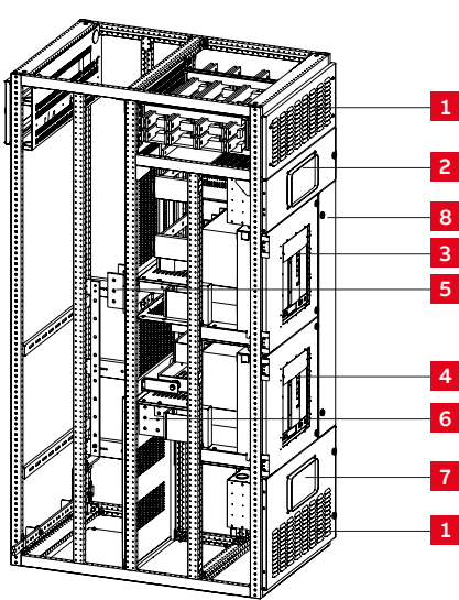
Figure 2-54 MNS Rear access double stacked ACB
