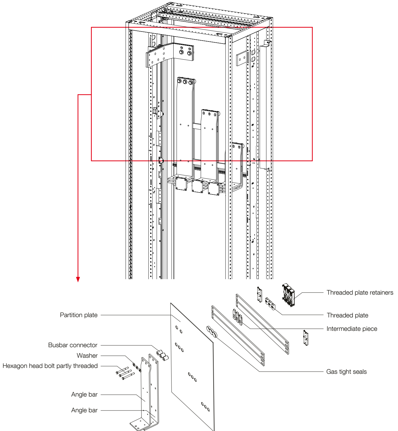
Figure 2-28 ACB copper connetion to main busbar
