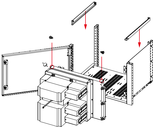
Figure 2-76 Module location guides and rails for larger modules. Larger modules can be equipped with location guides fixed to the top of the base plate. Guide rails are then mounted in the section.
