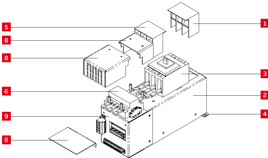
Figure 2-67 Compact module exploded view
