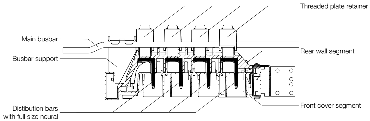
Figure 2-37 Top view of distribution bars
