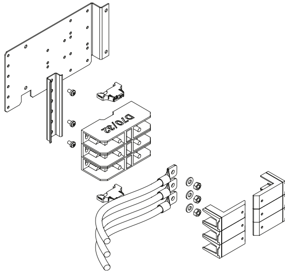
Figure 4-69 Example of MNS Rear fixed module cable connection with terminal blocks
