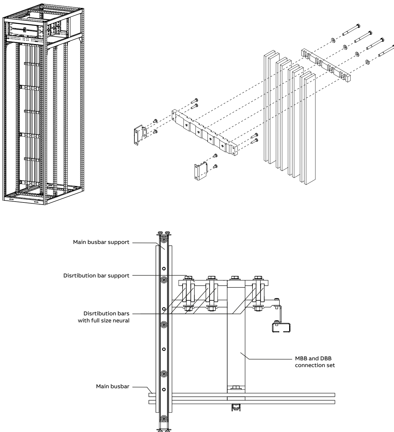
Figure 2-42 MNS Rear fixed distribution bars system
