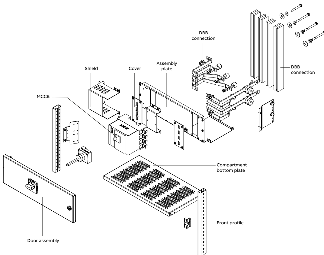
Figure 2-63 MNS Rear fixed module size 8E
