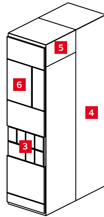
Figure 2-12 Rear combined ACB and withdrawable modules section
