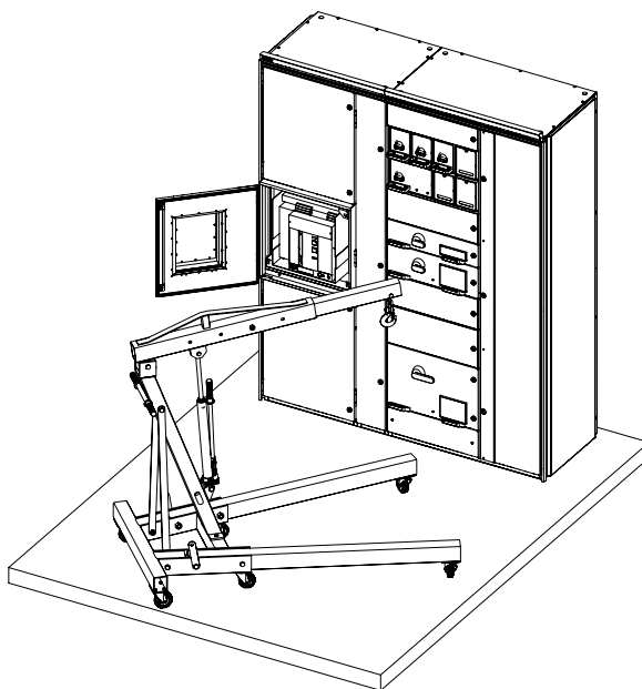
Figure 4-81 Installation of ACB using lifting truck
