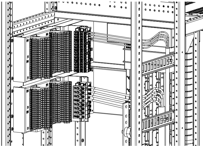
Figure 4-73 Example of MNS Rear cable runs, module sizes 8E/4 and 8E/2
