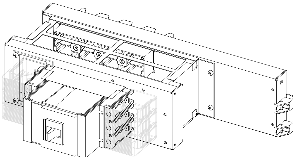
Figure 2-69 Basic plug-in energy distribution module
