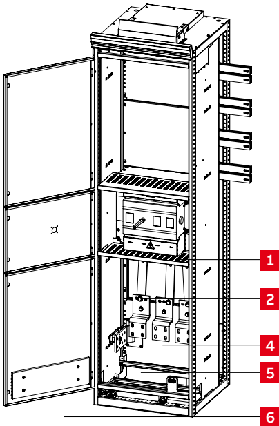
Figure 2-58 Switch-disconnector
