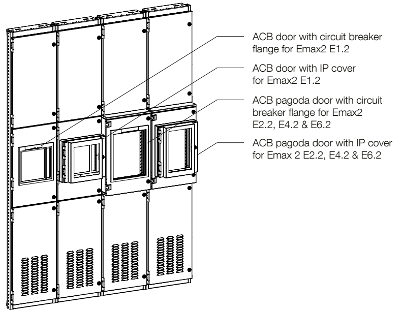
Figure 2-23 Air circuit breaker sections (example)
