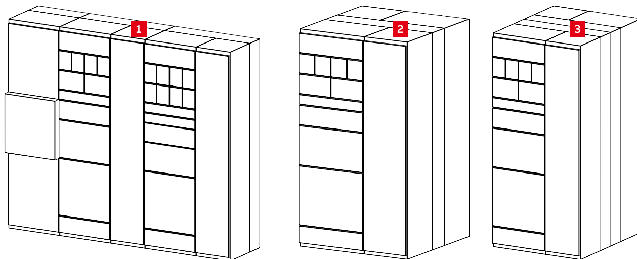
Figure 2-13 Assembly arrangements (from left): standard / duplex / back to back arrangement
