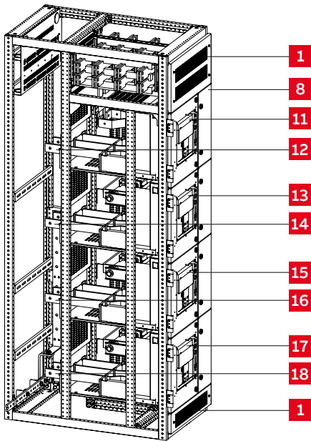
Figure 2-56 MNS Rear access quadruple stacked CB
