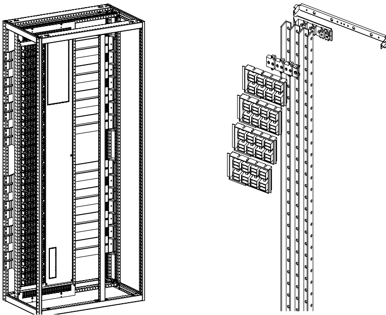
Figure 2-38 Metal separation wall MSW
