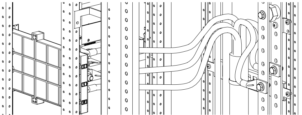
Figure 4-79 Example of MNS Rear access protection and neutral conductor connection
