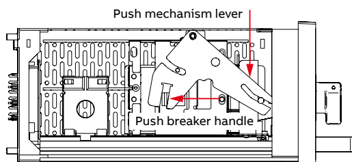
Figure 6-28 Reset operation in small modules, size 8E4 and 8E2, module drawn out
