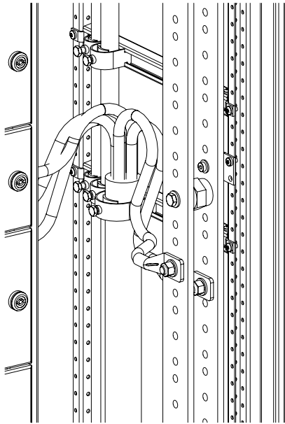
Figure 4-72 Example of front access protection and neutral conductor connection
