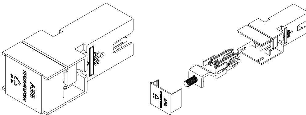
Figure 2-45 Sotax contacts are used for higher current application
