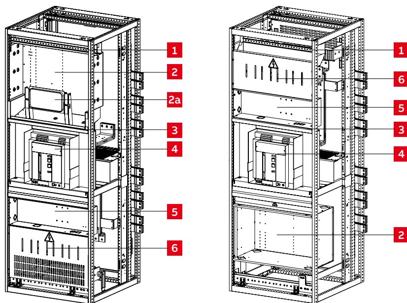
Figure 2-47 Circuit breaker section bottom entry configuration (left), top entry configuration (right)
