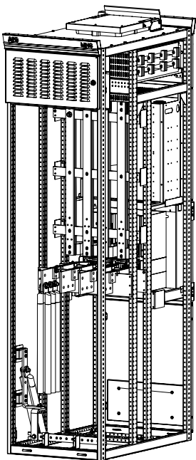
Figure 4-58 Example of cable connection in incoming / outgoing MNS Rear ACB unit
