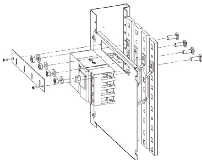
Figure 2-61 DBB connection with busbars
