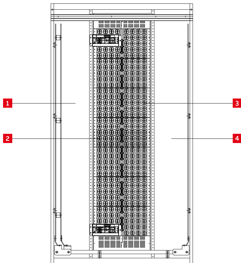
Figure 2-65 Multi-Function Separation Wall (MFSW) in section
