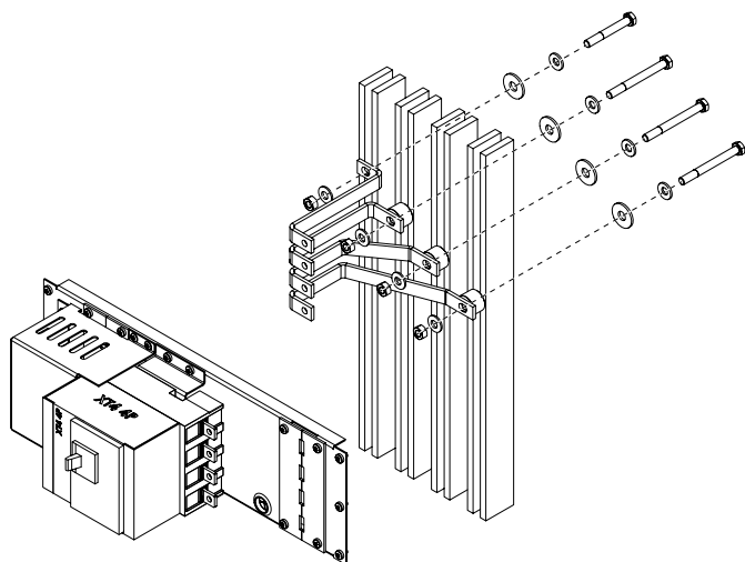
Figure 2-64 MNS Rear fixed DBB connection with busbars
