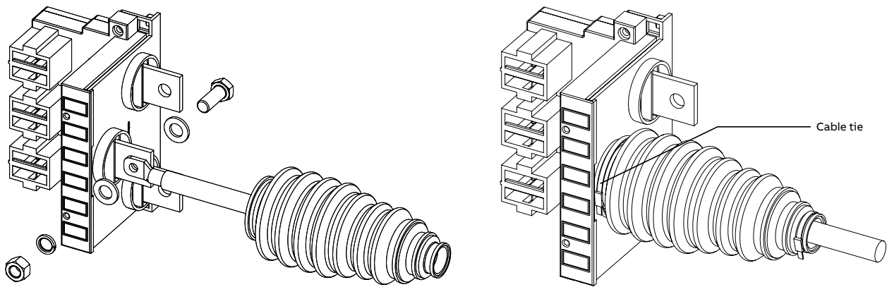
Figure 4-75 MNS Rear cables provided with bellows for \geq 4E modules and fixing material (1 spring lock washer and 2 plain washers)
