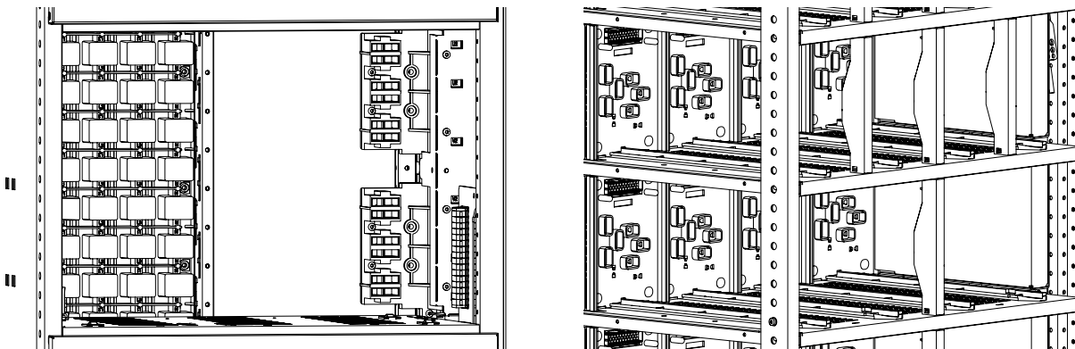
Figure 10-03 Withdrawable module compartment size 8E with outgoing cable connection unit (left) Conversion to withdrawable module compartments size 8E/4 and 8E/2 (right)
