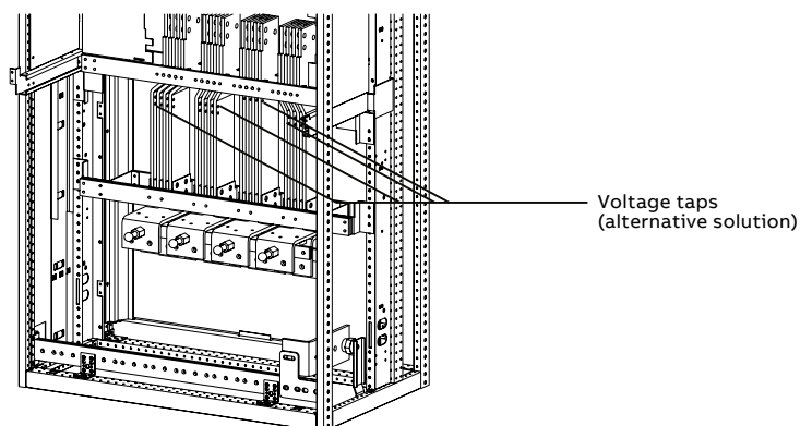
Figure 4-55 Location of voltage tape
