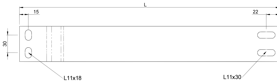
Figure 4-19 Generic busbar dimension in mm
