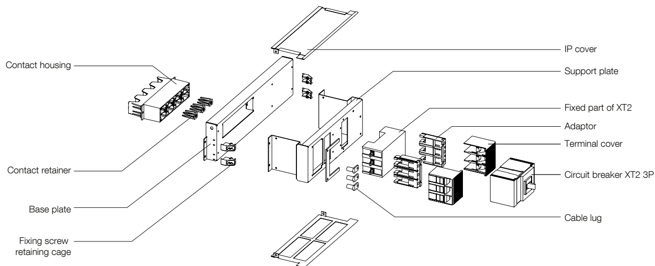
Figure 2-71 Exploded view of plug-in module cable connection to main contacts
