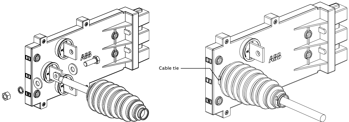
Figure 4-78 MNS Rear cables provided with bellows for \geq 4E modules and fixing material (1 spring lock washer and 2 plain washers)
