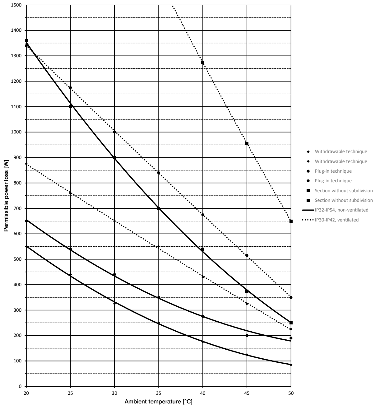
Figure 10-04 Standard values of maximum admissible effective power loss for sections with 600 mm equipment compartment width
