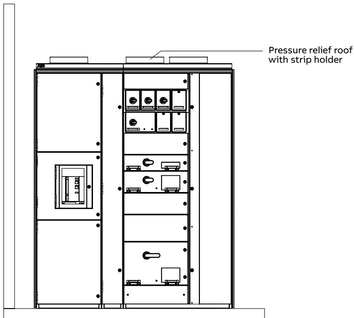
Figure 4-12 Example of section height extension parts
