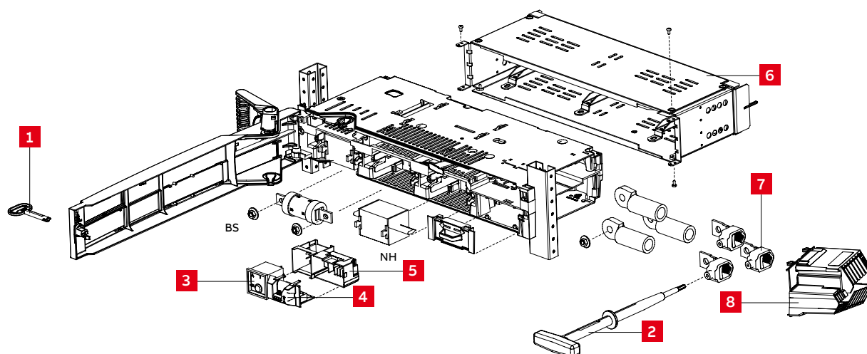
Figure 2-81 Exploded view and optional accessories of XR1
