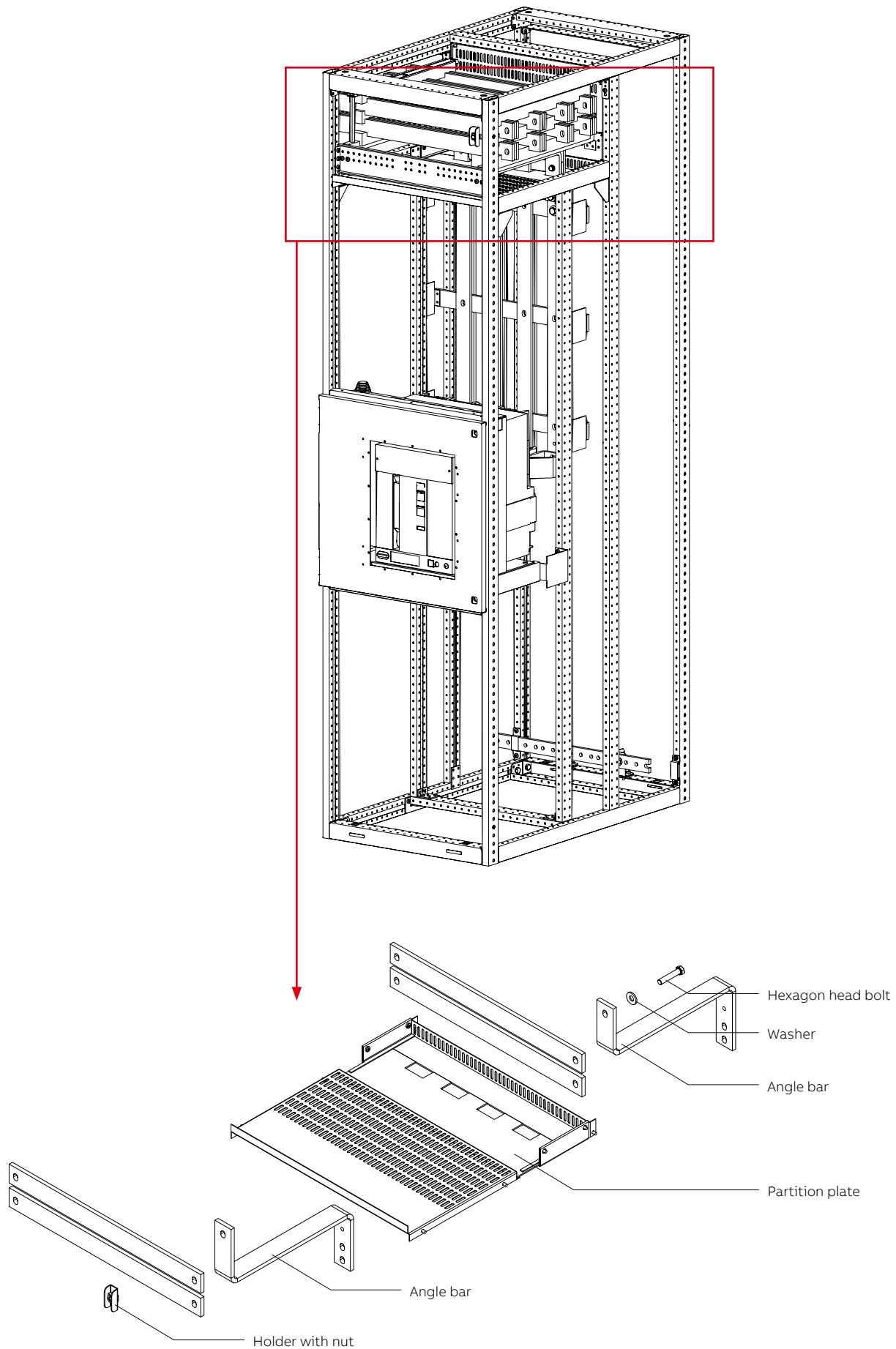
Figure 2-30 MNS Rear ACB copper connection to main busbar
