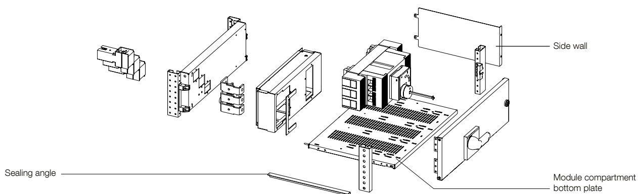
Figure 2-73 Exploded view of plug-in module with optional separation components
