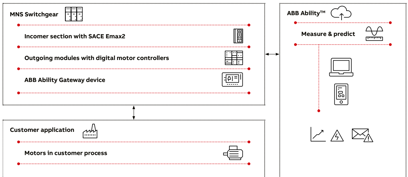
Figure 6-36 MNS Digital motor control operation
