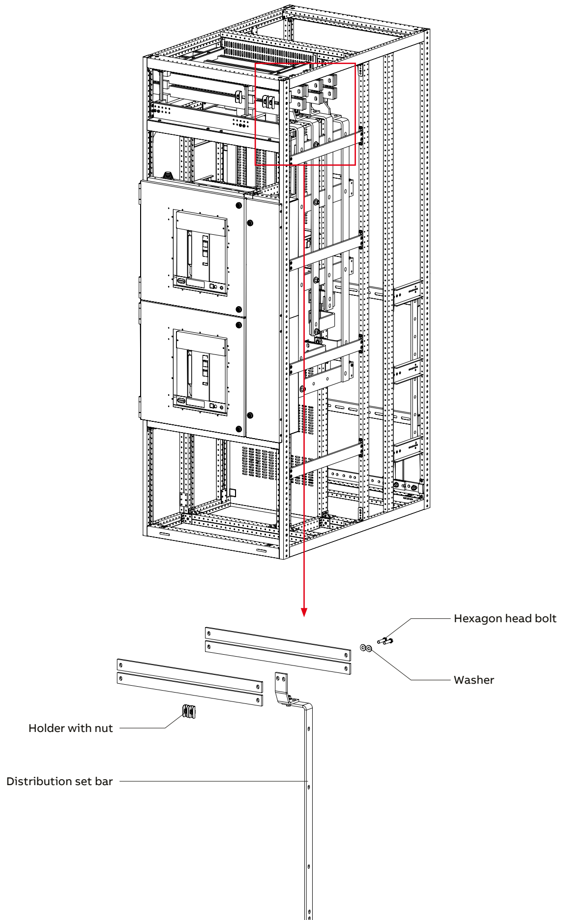
Figure 2-32 MNS Rear distribution set connection to main busbar
