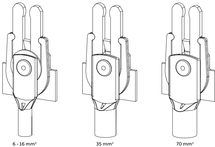
Figure 2-44 Power contacts used in MNS switchgear for different cable cross-sections
