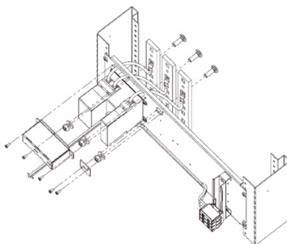
Figure 2-62 DBB connection with cables
