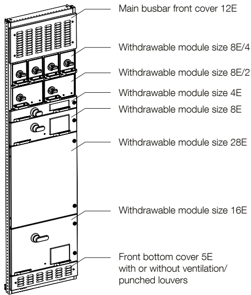
Figure 2-22 MNS Rear modules (example)
