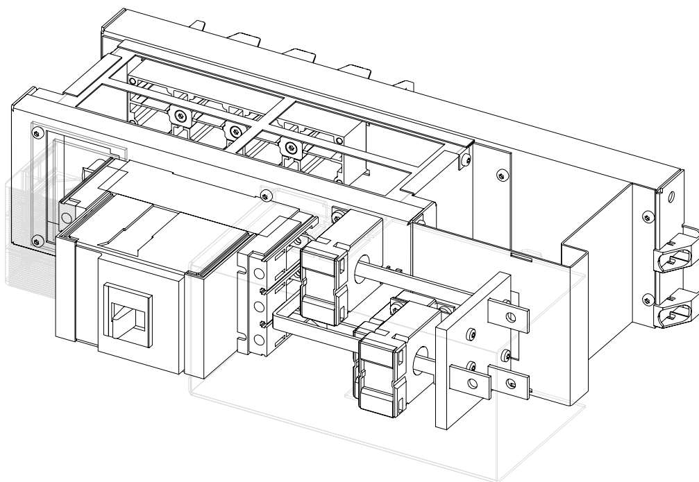
Figure 2-70 Energy distribution module with optional CT's
