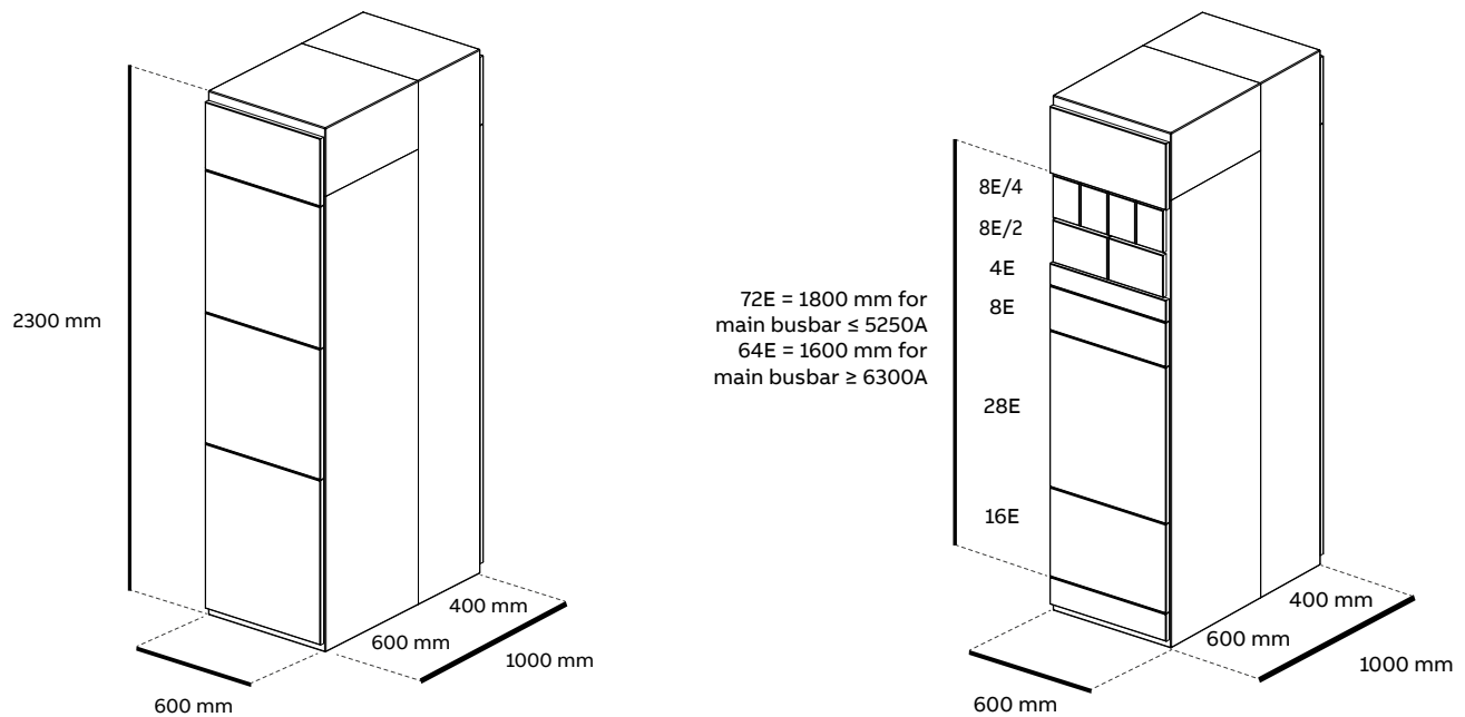
Figure 2-16 MNS Rear ACB section (left), module section (right)
