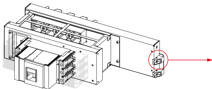
Figure 2-77 Fixing of the plug-in modules to the section
