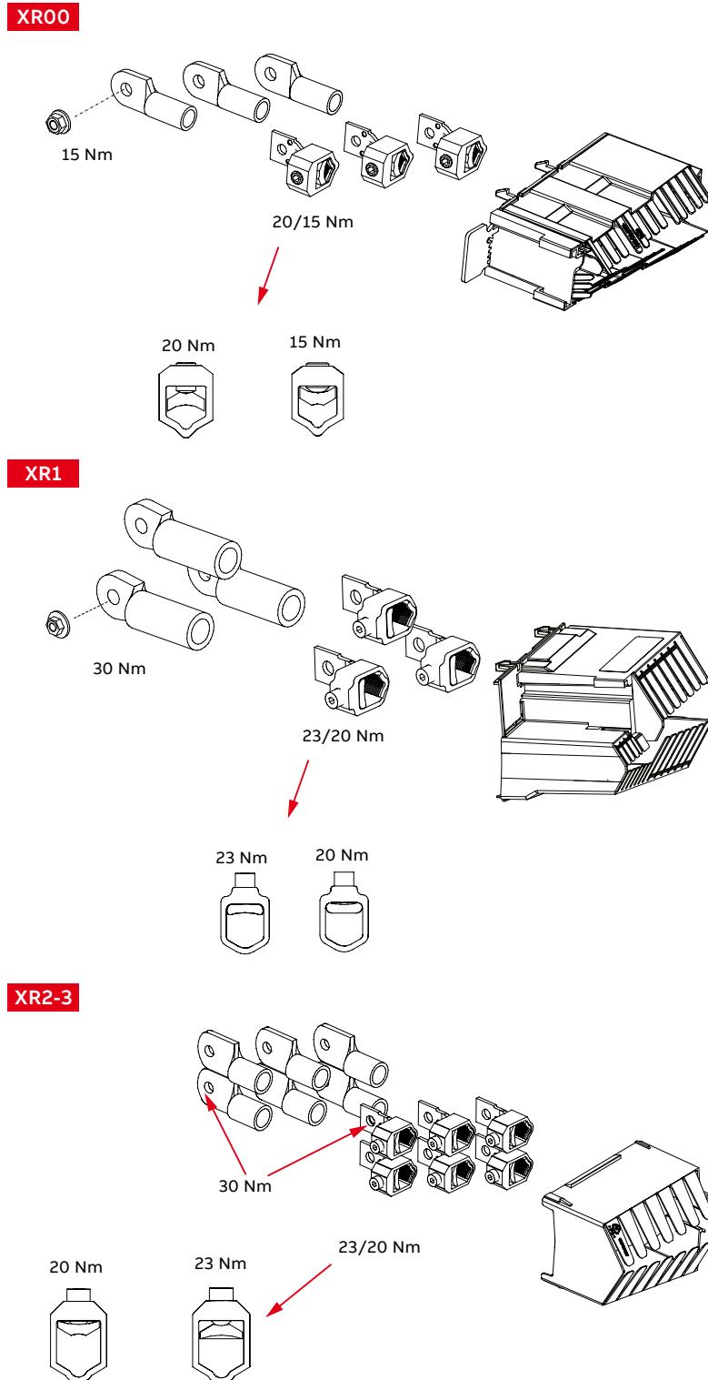
Figure 4-70 SlimLine modules cable connection
