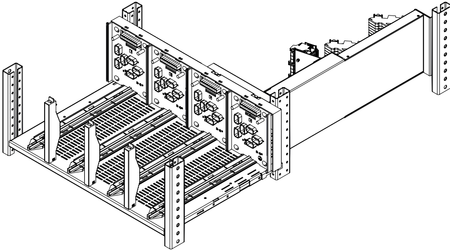
Figure 2-86 MNS Rear withdrawable module compartment for 4 units size 8E/4
