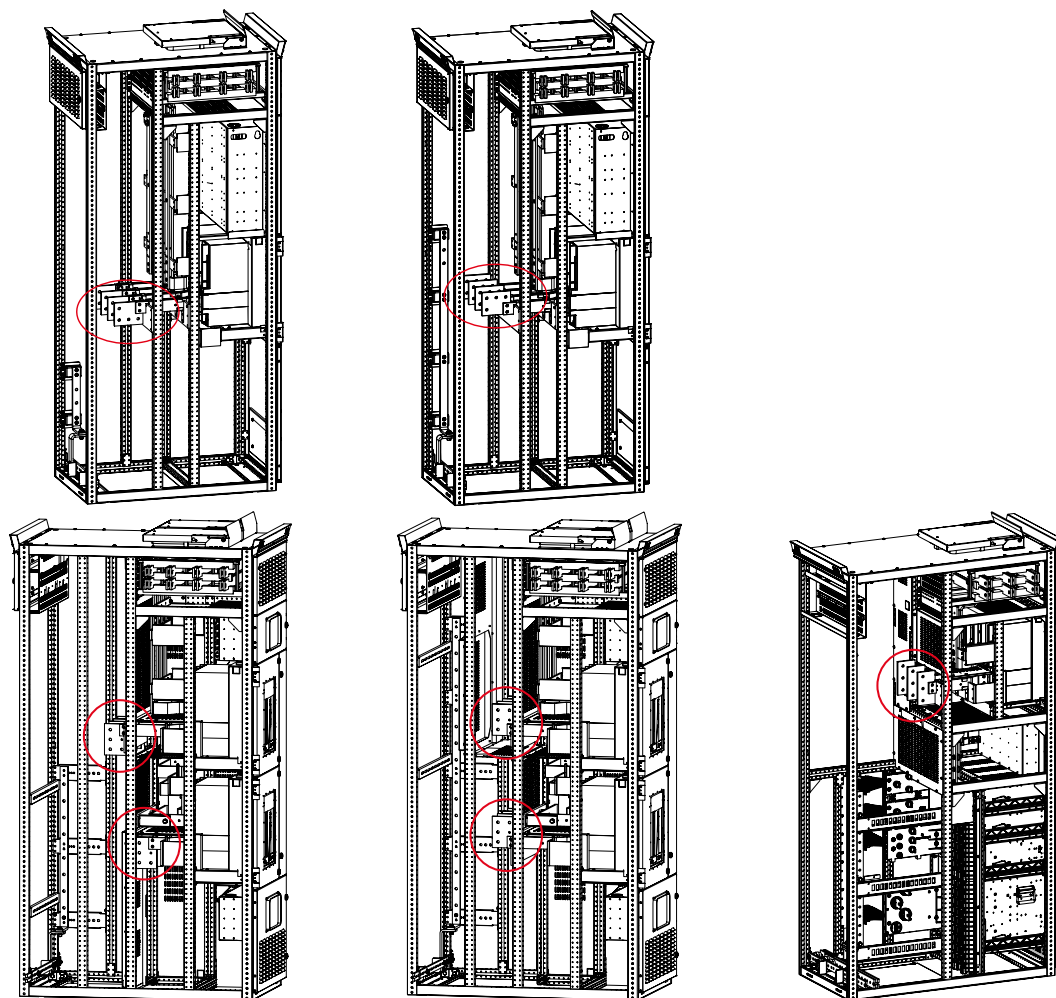
Figure 4-61 Location of MNS Rear cable bars acc. connection types
