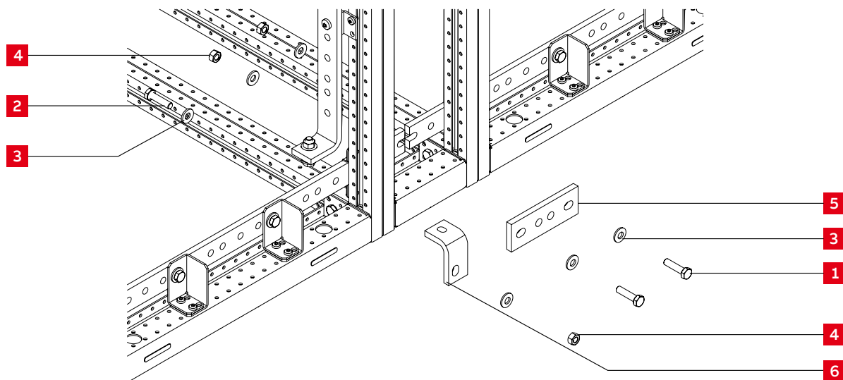
Figure 4-31 MNS Rear PE/PEN bar connection
