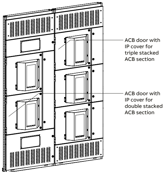
Figure 2-24 MNS Rear stacked sections (example)
