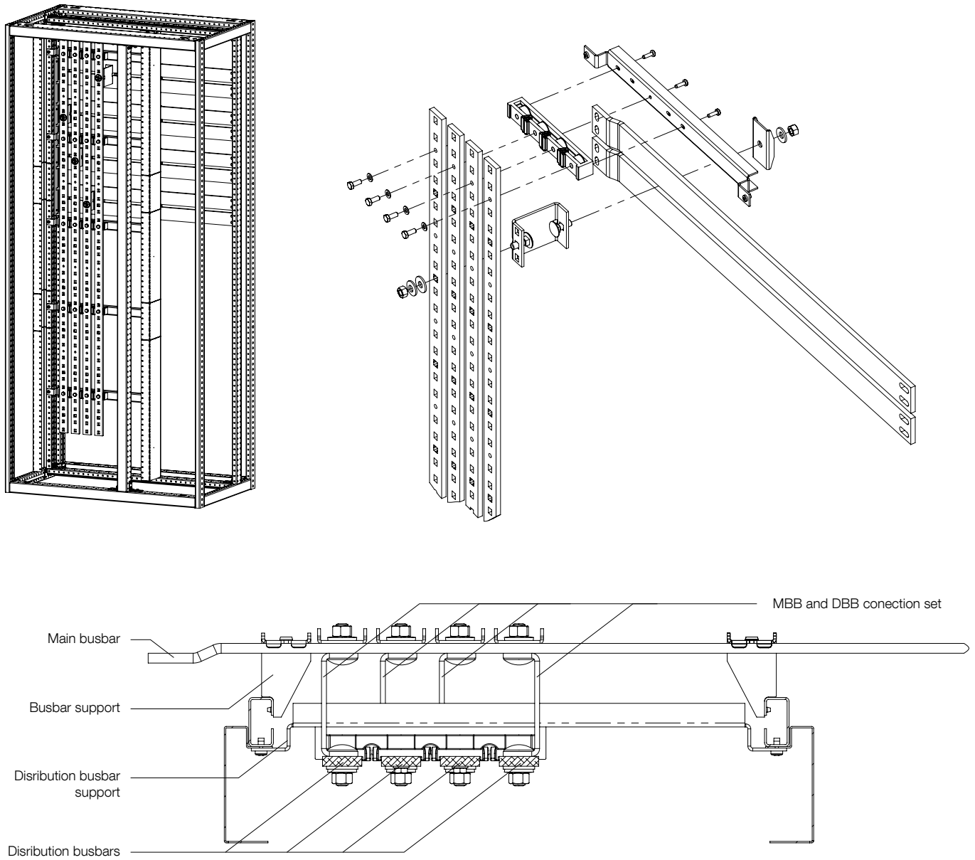
Figure 2-43 Fixed distribution bar system
