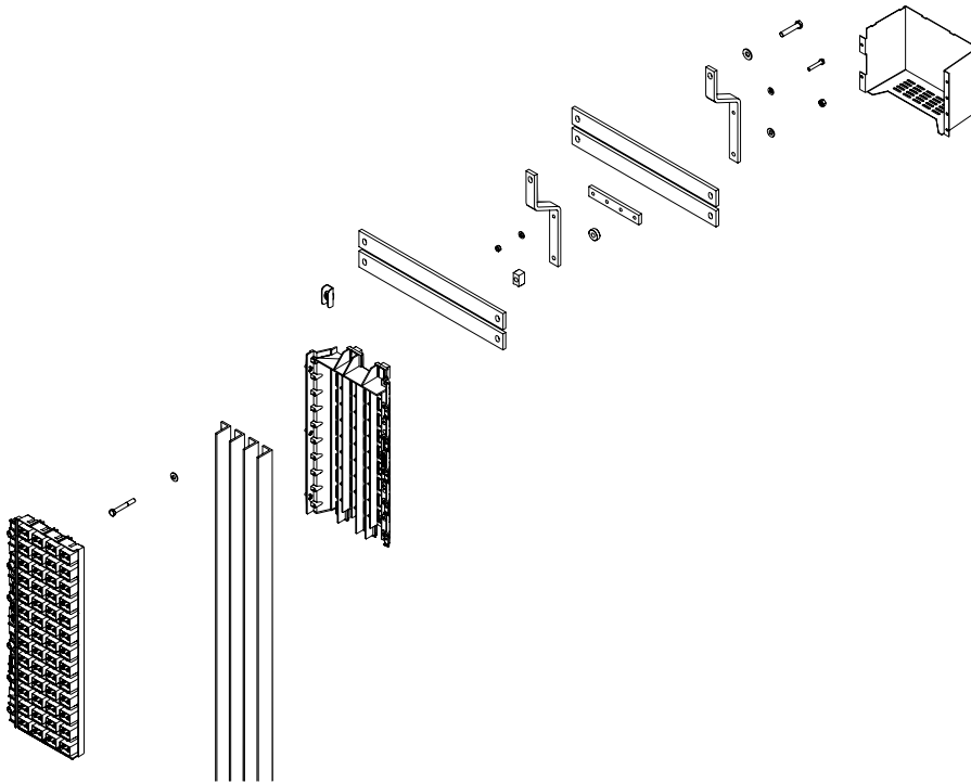
Figure 2-39 MNS Rear distribution bars
